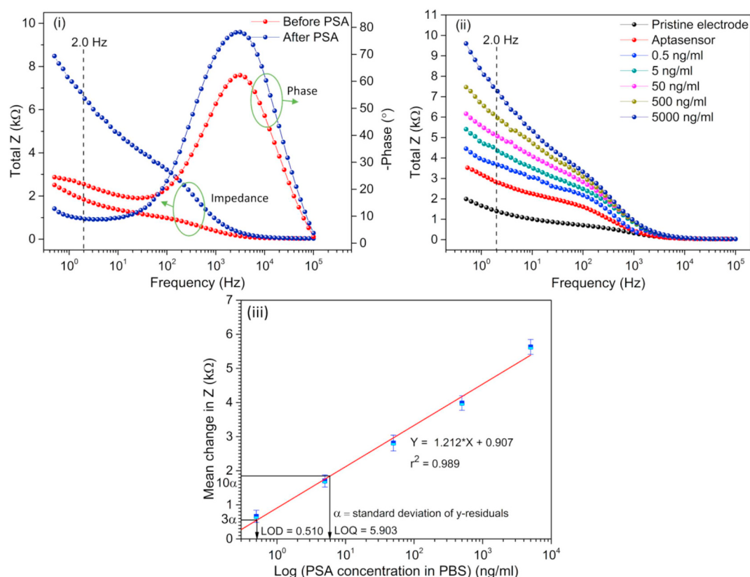
Fig. 5. The feasibility study of EIS responses for evaluating sensor's specificity, tested against different concentrations of PSA in undiluted human serum. (i). Dose-response for changes in total Z and phase data versus frequency before and after PSA binding at 1 µg/ml. (ii). Bode plot for detection of different concentrations of PSA. (iii). Calibration curve showing linear detection of PSA concentration in undiluted human serum.
