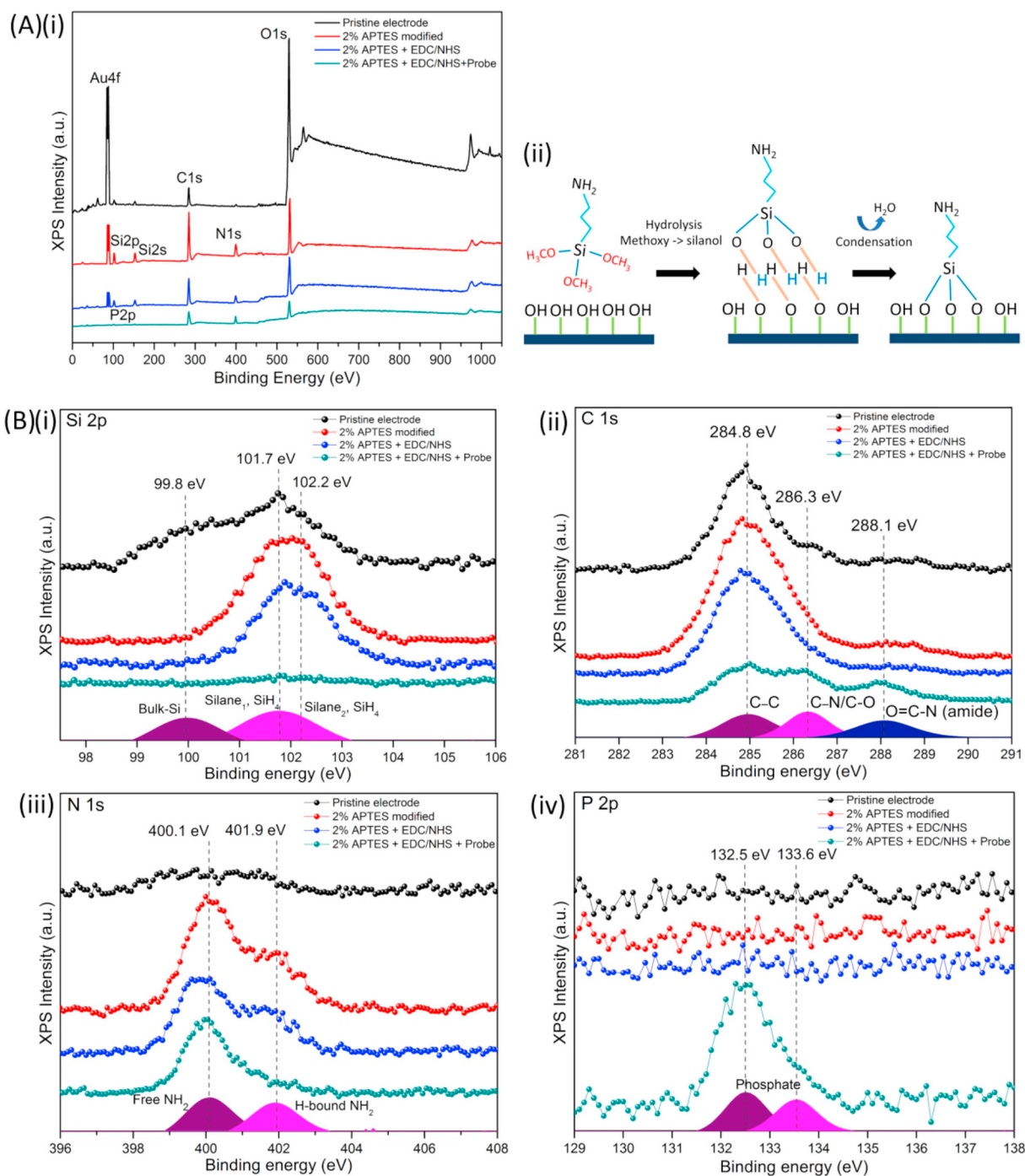
Fig. 2. XPS spectra analysis of surface functionalization on the sensing surface. Fig. 2A(i). An overlay of XPS survey spectra for each electrode modification step. Fig. 2A(ii). APTES silanization process with a hydroxyl group on SiO 2 substrate. Fig. 2B(i-iv). High-resolution narrow peaks of Si 2p, C 1s, N 1s and P 2p with respect to the binding energy (BE).
