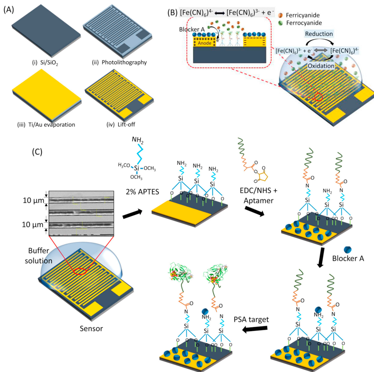
Fig. 1. A(i-iv). The conventional photolithography process steps to fabricate the gold interdigitated microelectrode. Fig. 1B. The Faradaic EIS detection scheme for PSA target on sensing surface. Fig. 1C. Representation of surface modification techniques on the electrode surface for the detection of PSA protein. Images drawn not according to the actual dimensions.
