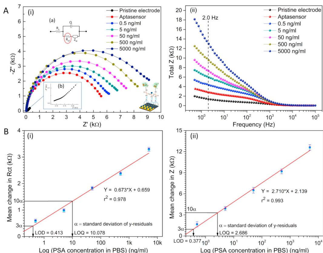
Fig. 4. EIS responses of developed sensing devices to detect different concentrations of PSA antigen, measured in Buffer C. A(i). The -Z'' vs. Z' 'Nyquist plot' with an inset (a) showing the equivalent Randle's circuit. A(ii). The total Z vs. frequency 'Bode plot'. Fig. B. The calibration curve with respect to (i) Nyquist plot and (ii) Bode plot.
