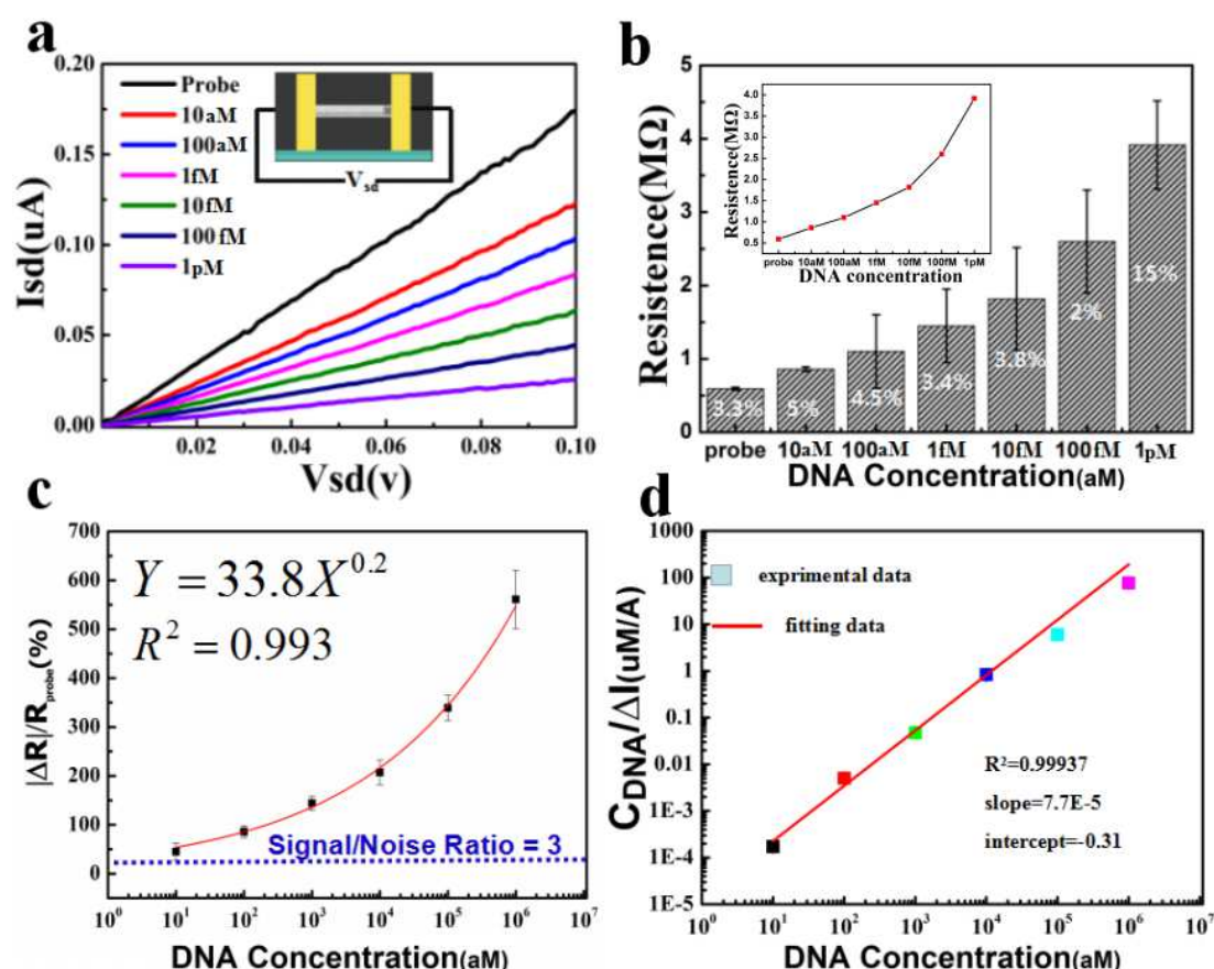
Fig. 5. (a) I_{sd} - V_{sd} curve of an SCNT-FET device hybridized with FC-DNA at a series of concentrations from 10 aM to 1 pM ( V_{sd}
