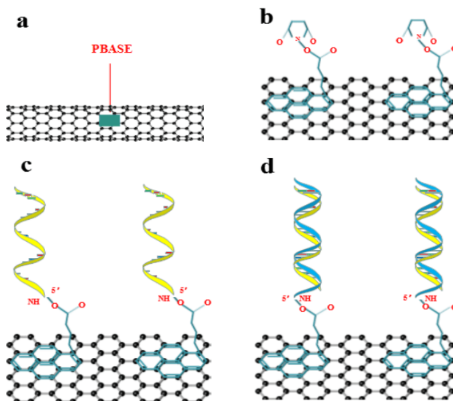
Fig. 3. Schematic illustration of a suspended CNTFET for DNA detection. (a) Functionalization of the SCNT surface by PBASE.
