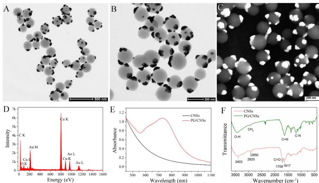
Fig. 1 TEM (A, B) and SEM (C) images of PG/CNSs; EDX pattern of PG/CNSs (D); UV-vis-NIR absorbance spectra (E) and FT-IR spectra (F) of CNSs and PG/CNSs.
