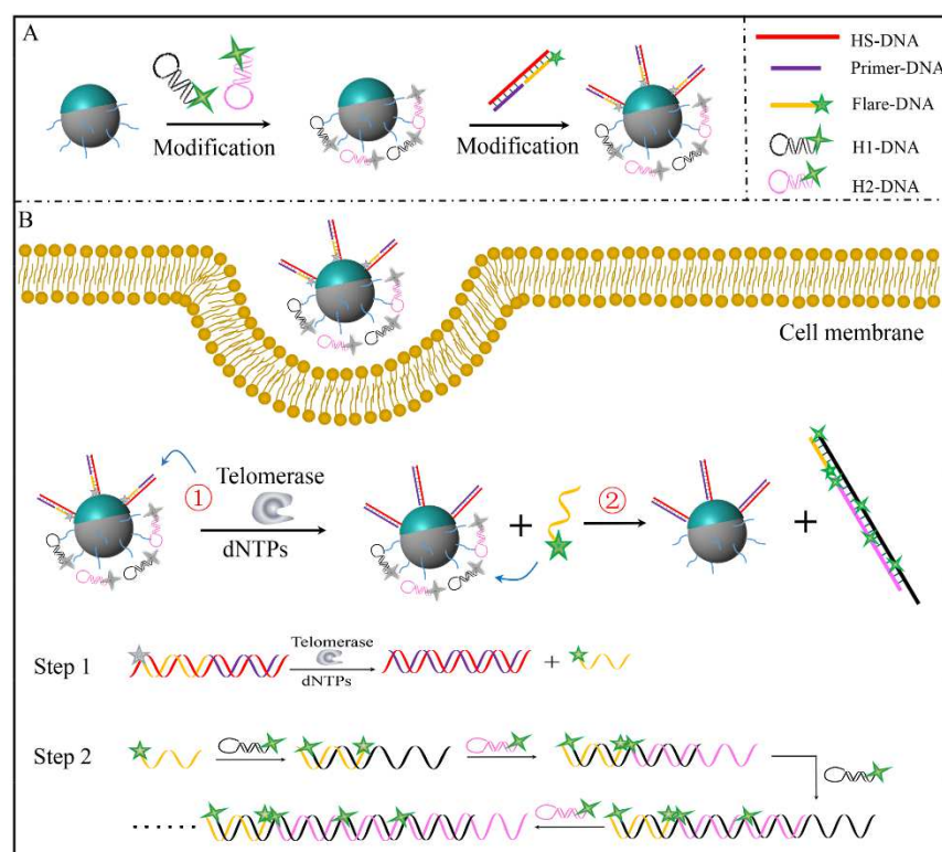
Scheme 1. (A) Schematic diagram of the preparation process of PG/CNS-based sensor. (B) Schematic illustration of PG/CNSs-based mimic-HCR sensor for in situ detection of intracellular telomerase.
