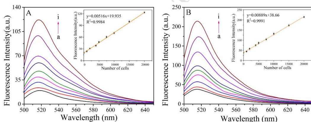
Fig. 5 Fluorescence spectra of the detection system by using sensor 1 (A) and sensor 2 (B). The different amounts of telomerase extracts from 0, 1000, 2000, 4000, 5000, 7500, 15000, 20000 A549 cells (a-i). Inset: The fluorescence intensity at 515 nm vs. the number of cells.
