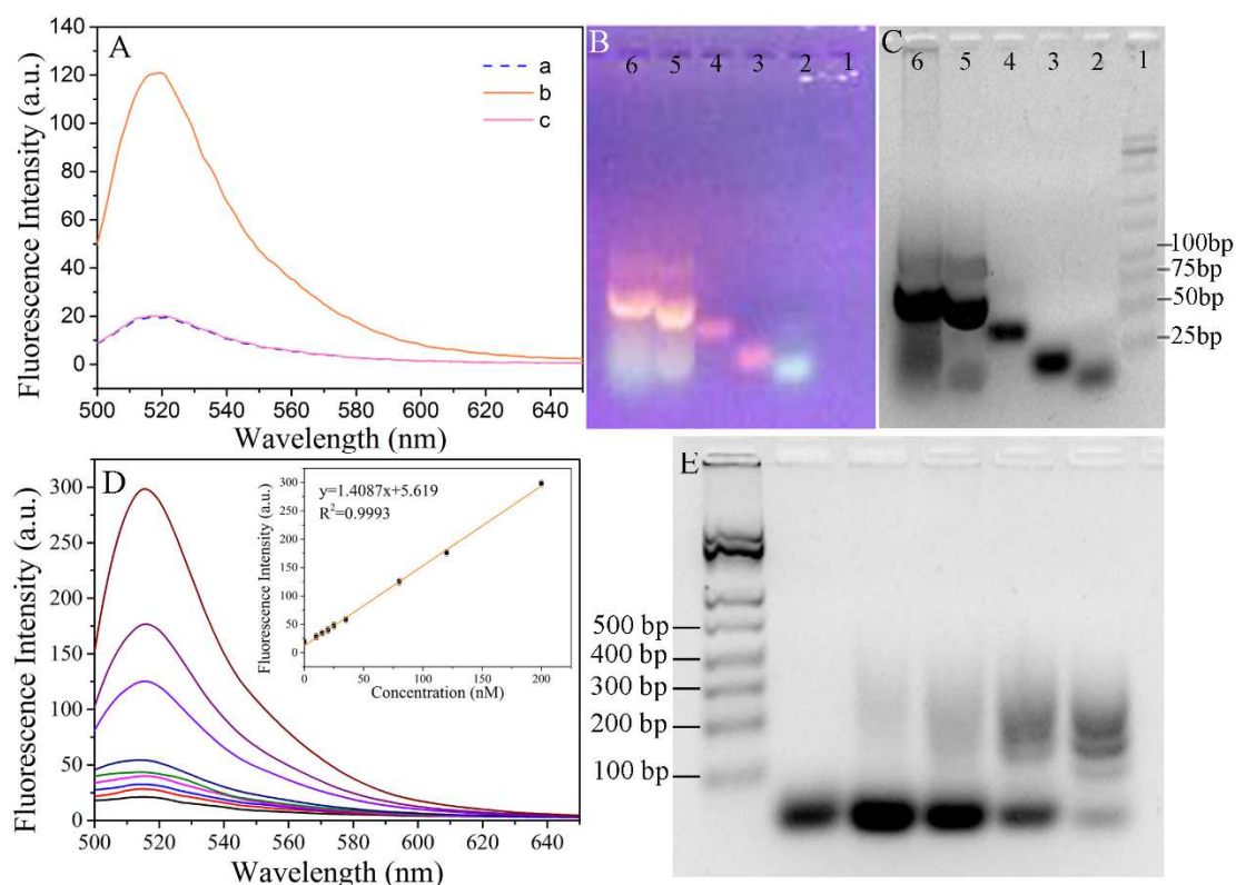
Fig. 2 (A) Fluorescence spectra of the sensor 1 (curve a), sensor 1 and dNTPs in the presence (curve b) or absence (curve c) of telomerase; (B, C) Analysis of gel electrophoresis for telomerase-triggered Primer-DNA extension and Flare-DNA release. (1: maker DNA, 2: Flare-DNA; 3: Primer-DNA; 4: HS-DNA; 5: hybridized-DNA + dNTPs; 6: hybridized-DNA + dNTPs + telomerase); (D) Fluorescence recovery after adding Trigger DNA (0, 10, 15, 20, 25, 35, 80, 120, 200 nM) into PG/CNSs mimic-HCR system ( 75 \mu\text{g} \cdot \text{mL}^{-1} ), Insert: the plot of fluorescence intensity recorded at 515 nm vs. the concentration of Trigger DNA. (E) Analysis of gel electrophoresis for Flare-DNA initiated mimic-HCR. (1: maker DNA, 2: H1-DNA, 3: H1-DNA+H2-DNA, 4: H1-DNA+H2-DNA+0.25 \mu\text{M} Flare-DNA, 5: H1-DNA+H2-DNA+1 \mu\text{M} Flare-DNA, 6: H1-DNA+H2-DNA+2.5 \mu\text{M} Flare-DNA after incubation for 2 h).
