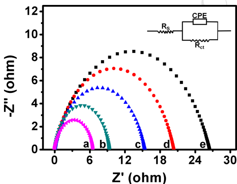
Fig. 2 Nyquist plots of EIS for different modified electrodes: (a) WS 2 NW/TM, (b) WS 2 NW/TM-aptamer, (c) WS 2 NW/TM-aptamer-BSA, (d) WS 2 NW/TM-aptamer-BSA-HER2, (e) WS 2 NW/TM-aptamer-HER2-[peptide-Au NPs-GOx].
