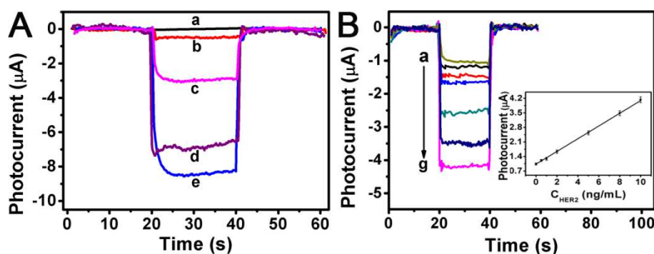
Fig. 3 (A) PEC responses of (a) bare Ti mesh, (b) WS 2 NW/TM, (c) WS 2 NW/TM-Au NPs, (d) WS 2 NW/TM containing 5 mM H 2 O 2 , (e) WS 2 NW/TM-Au NPs containing 5 mM H 2 O 2 in 0.1 M PBS (pH = 7.0). (B) Photoelectrochemical response of WS 2 NW/TM-aptamer-HER2-[peptide-Au-GOx] toward HER2 at different concentrations: (a) 0, (b) 0.5, (c) 1, (d) 2, (e) 5, (f) 8, (g) 10 ng/mL recorded in 0.1 M PBS containing 10 mM glucose. The inset is the linear range from 0.5 to 10 ng/mL for HER2 detection.
