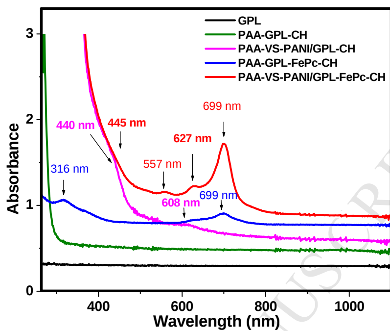
Fig. 1. UV-visible spectra of hydrogel modified electrodes
