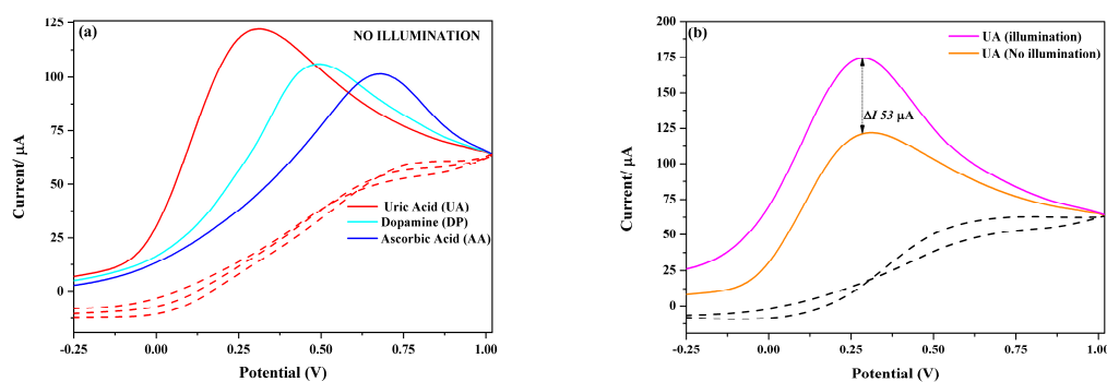
Figure 4. (a) CV curves depicting oxidation of UA, DP and AA with equimolar concentration of 1.5 mM under no-illumination condition (b) increased photocurrent oxidation response for UA under the illumination condition using ITO/NiWO 4 as working electrode respectively.
