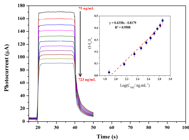
Figure 5. Photocurrent responses of ITO/NiWO 4 /Ab against different concentrations of NSE ranging from 75 to 723 ng.mL -1 . (inset) Corresponded calibration curve plotted between photocurrent and log of NSE concentration. Measurements were carried out in 0.1 M PBS (pH 7.0) with 1.5 mM UA at a bias potential of +0.3 V.
