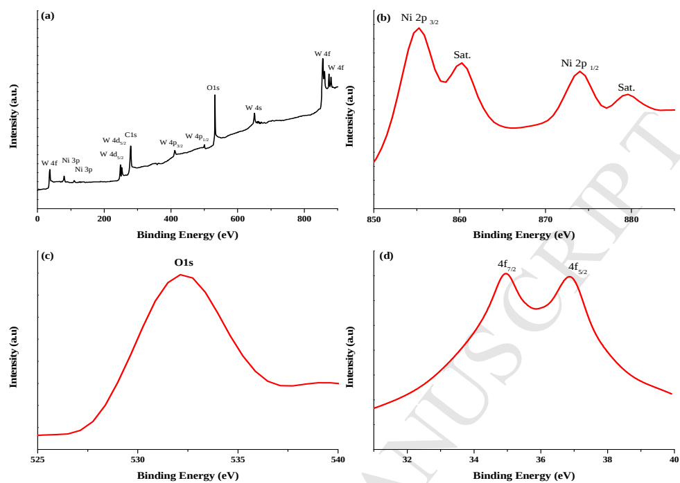
Figure 2. XPS analysis of in-situ-grown \text{NiWO}_4 nanostructures. (a) Survey spectrum consisting of peaks assigned to Ni, W and O. (b-d) High-resolution spectra for Ni2p, O1s and W4f binding energy regions, respectively.
