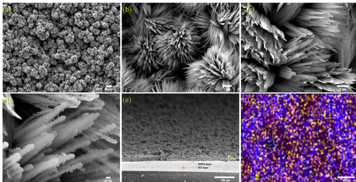
Figure 1. (a-d) FE-SEM images captured for ITO/NiWO 4 at various magnifications. (e) Cross-section of ITO electrode with in-situ-grown layer of NiWO 4 nanostructure, and (f) EDS elemental mapping indicating presence of Ni, W and O.
