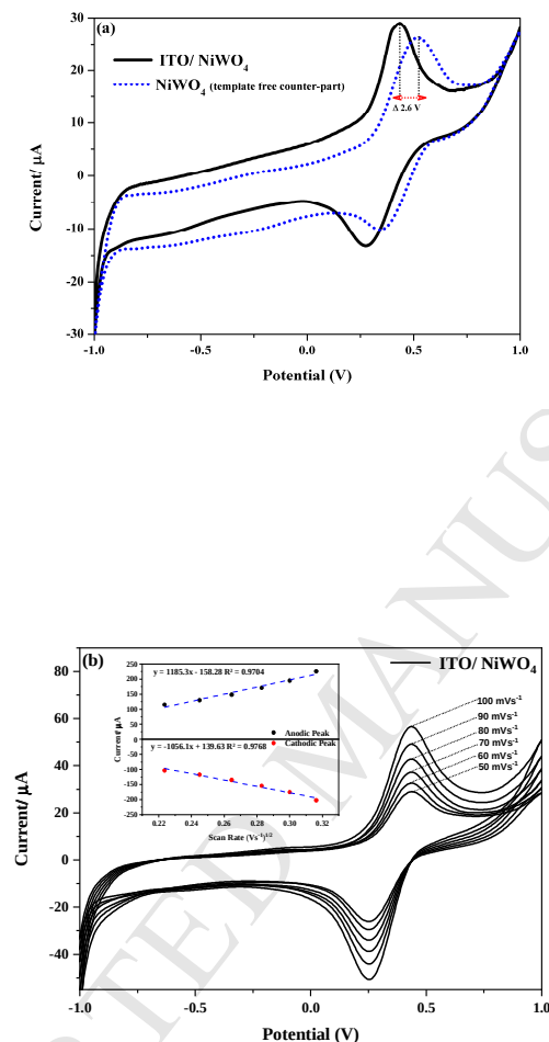
Figure 3. (a) CV behaviour of ITO/NiWO 4 in reference to its template-free counterpart deposited on GCE at a fixed scan rate of 50 mV.s -1 . (b) Increasing anodic and cathodic responses of ITO/NiWO 4 against gradual rise of scan rate from 50 to 100 mV.s -1 . (inset) Graph justifying the observed linearity between current and square root of scan rate.
