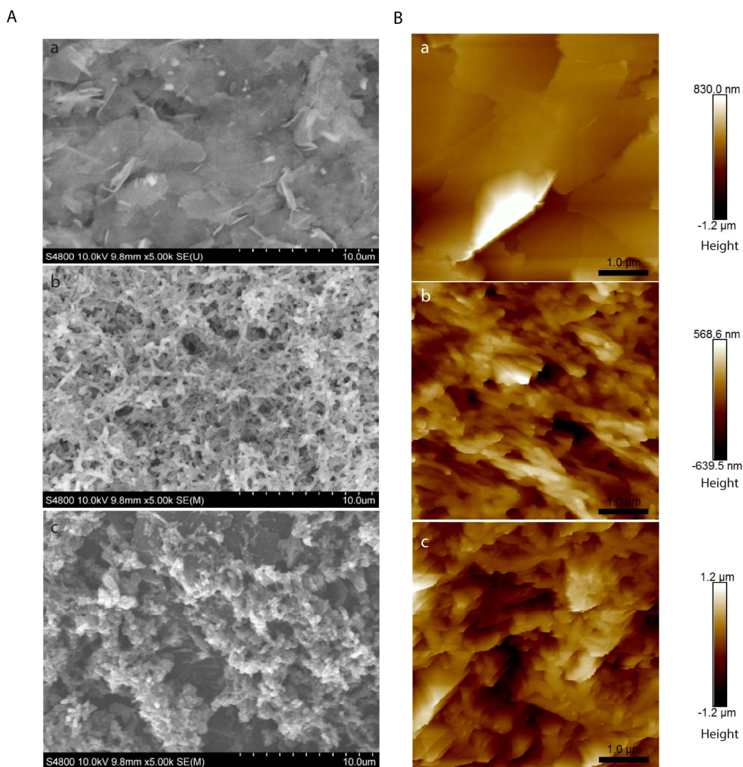
Fig. S1. Surface characterization of biosensor assembly. (A) Scanning Electron Microscopy of (a) unmodified graphene; (b) graphene modified with PANI (C); anti-ach3 attached to the PANI layer; (B) Atomic Force Microscopy of (a) unmodified graphene; (b) graphene modified with PANI (c); anti-ach3 attached to the PANI layer.
