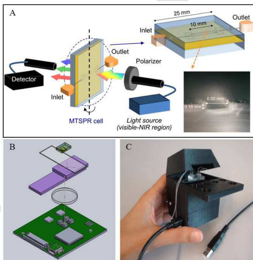
Fig. 5. (A) (Color online) Experimental setup of MTSPR measurement. Photographic image showing cross section of microchannel with the dimension of 0.50 \times 0.15 \text{ mm}^2
