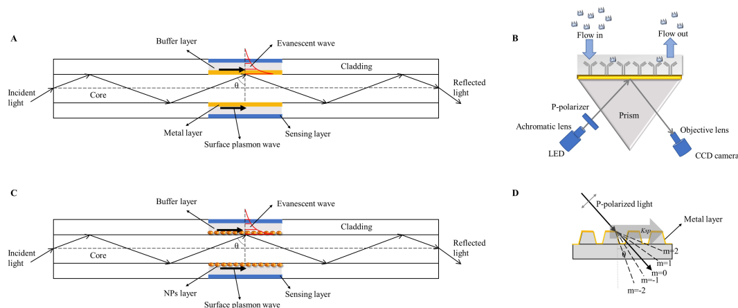
Fig. 2. Schematic diagrams of four types of SPR biosensors. (A) The fiber-optic surface plasmon resonance (FOSPR) biosensor. (B) The structure of a surface plasmon resonance imaging (SPRI) biosensor. (C) The localized surface plasmon resonance (LSPR)-based fiber-optic biosensor. (D) The conventional configuration of the transmission surface plasmon resonance (TSPR) biosensor.
