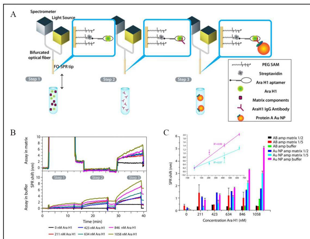
723 724 Fig. 10. (A) Schematic representation of multi-step protocol for Ara h 1 protein 725 detection in food matrix samples. (B) Detection of FOSPR aptasensor of Ara h 1 726 protein at various concentrations using the multi-step protocol in TGK buffer and 727 candy bar matrix. (C) Quantification of SPR signal shifts and calibration curves 728 obtained with FOSPR aptasensor (Tran et al., 2013).
