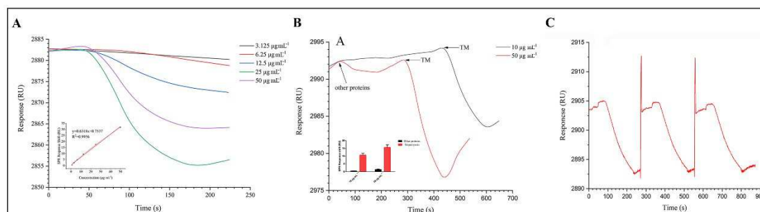
Fig. 11. (A) SPR sensorgram of tropomyosin standards at different concentrations and standard curve. (B) Relative responses of the other nonallergenic proteins in shellfish towards the sensor surface. (C) SPR sensorgram of tropomyosin standards under continuous injection.
