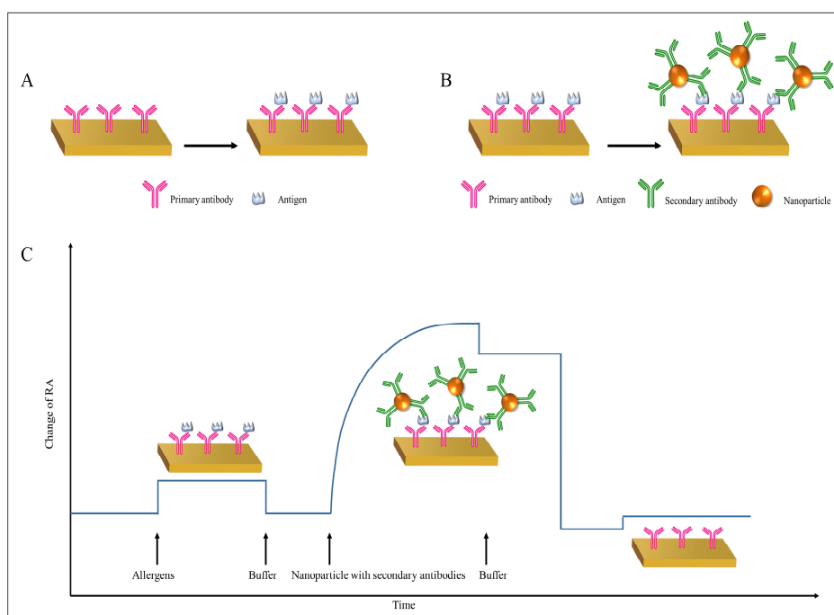
Fig. 6. Schematic diagram of antibody-based SPR biosensors to quantify food allergens. (A) Direct SPR immunoassay. (B) Sandwich SPR immunoassay. (C) The real-time SPR sensorgram of food allergens using an SPR immunoassay.
