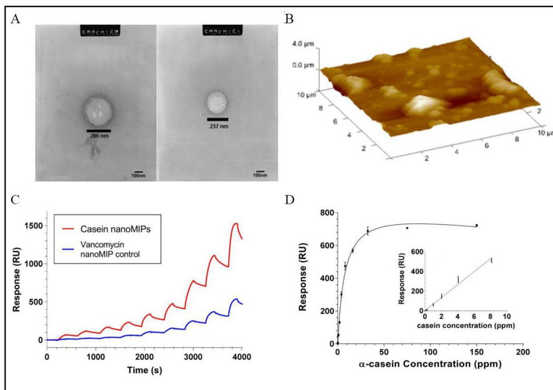
Fig. 8. (A) TEM image of \alpha -casein nanoMIPs taken on a Phillips CM20. (B) AFM covalently attached nanoMIPs. (C) Typical sensorgram for a nanoMIP based biosensor synthesized from the bead-based method. (D) Non-linear ( R^2=0.9934 ) and linear calibration ( R^2=0.9779 ) plot for the \alpha -casein nanoMIP based biosensor ( n=3 ) (Ashley et al., 2018b).
