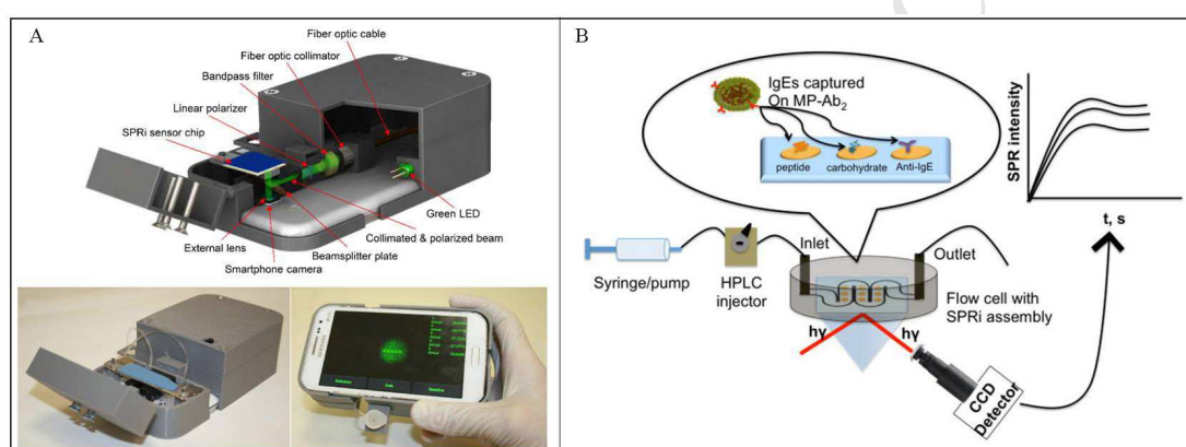
Fig. 3. (A) SPRI platform integrated with a smartphone for real-time and on-site monitoring of multiple sensing spots (Guner et al., 2017). (B) SPRI microarray configured to detect IgE binding to Ara h2 peptide, BXG, and anti-IgE using antibody-loaded magnetic particles (MP-Ab 2 ) for capture and signal amplification (Joshi et al., 2014).
