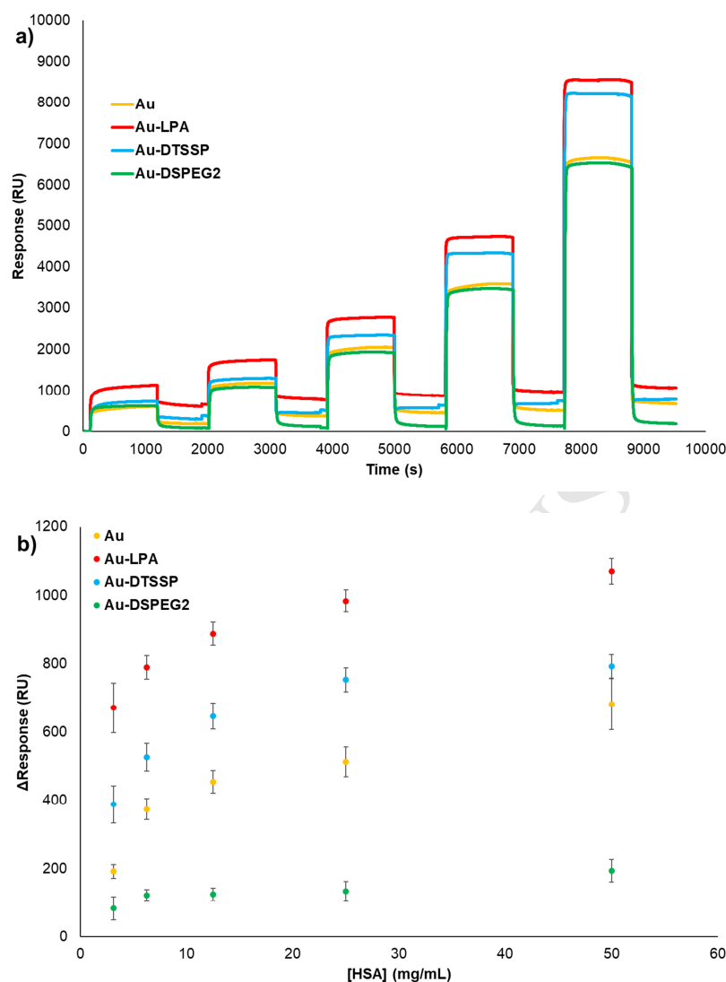
Figure 4. SPR sensorgrams of anti-NSA measurements using various concentrations of HSA on a bare gold surface (yellow), LPA-modified gold surface (red), DTSSP-modified gold surface (blue), and DSPEG2-modified gold surface (green). a) Real time SPR responses and b) \Delta Response displays the increase in SPR response before and after the exposure to increasing concentrations of HSA.
