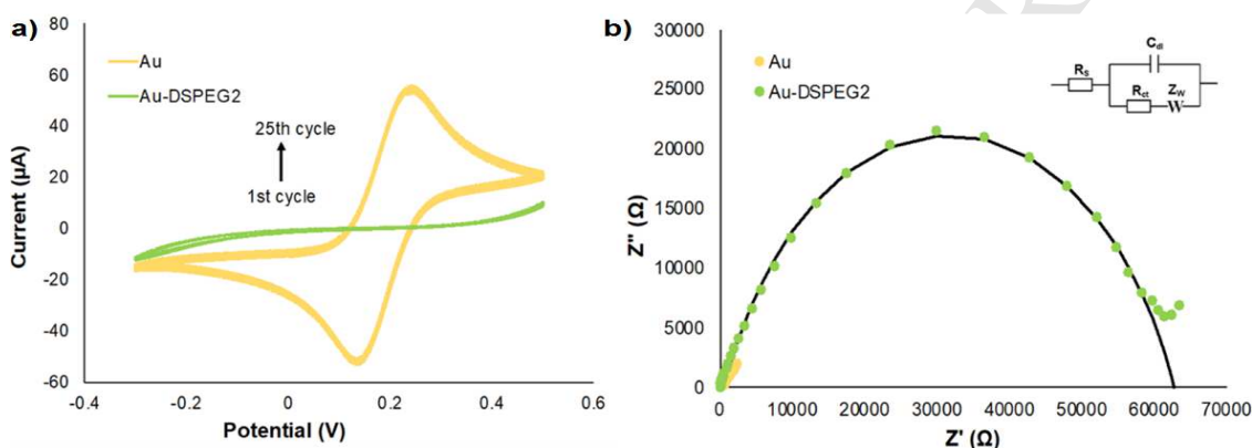
Figure 3. a) Cyclic voltammograms at a scan rate of 0.1 V/s for 25 cycles; and b) Nyquist plots with applied frequency from 0.1 Hz to 10 kHz of bare gold electrode (yellow) and DSPEG2 modified gold electrode (green) in 10 mM [\text{Fe}(\text{CN})_6]^{3-/4-} with 0.1 M \text{NaClO}_4 as supporting electrolyte. The charge-transfer resistance R_{ct} values were obtained by fitting the Nyquist plot with a Randles equivalent circuit (inset).
