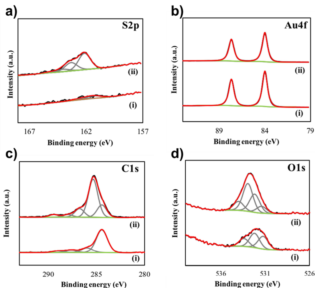
Figure 1. XPS data plots for S2p (a), Au4f (b), C1s (c) and O1s (d) on bare gold surface (i) and DSPEG2-modified surface (ii). Modification conditions were as described in Experimental section (a.u = arbitrary units).
