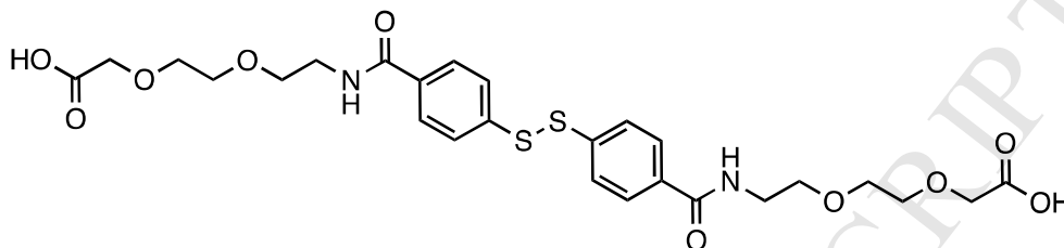
Scheme 1. Proposed structure of the thiolated-PEG linker molecule.
