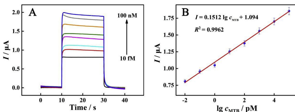
Fig. 5. PEC signals of the biosensor with various concentrations: 10.0 fM, 100 fM, 1.00 pM, 10.0 pM, 100 pM, 1.00 nM, 10.0 nM and 100 nM (A). Working curve between the photocurrent and the logarithm of different DNA concentration (B).
