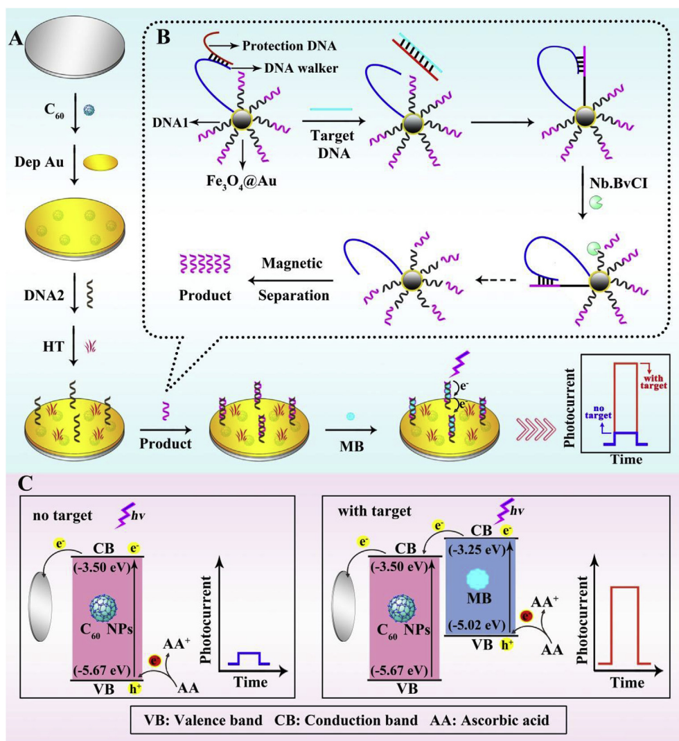
Scheme 1. The construction procedure of the PEC biosensor based on fullerene with methylene blue as a sensitizer for ultrasensitive DNA detection (A), the detailed enzyme-assisted signal amplification procedure (B), and the mechanism for photocurrent generation (C).
