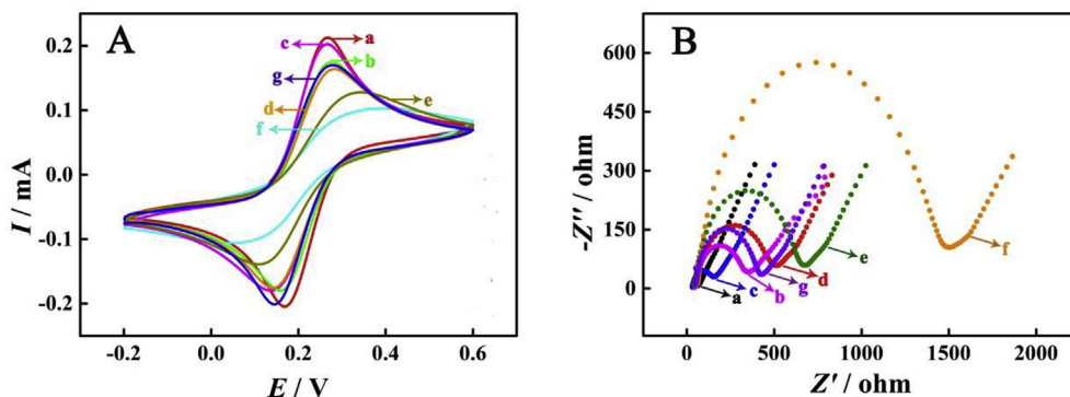
Fig. 3. CV and EIS responses of bare GCE (a), C_{60} NPs/GCE (b), Dep Au/ C_{60} NPs/GCE (c), DNA2/Dep Au/ C_{60} NPs/GCE (d), HT/DNA2/Dep Au/ C_{60} NPs/GCE (e), product/HT/DNA2/Dep Au/ C_{60} NPs/GCE (f) and MB/product/HT/DNA2/Dep Au/ C_{60} NPs/GCE (g).
