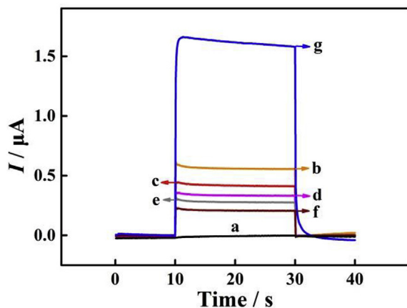
Fig. 4. PEC responses toward 1 nM target DNA of bare GCE (a), C_{60} NPs/GCE (b), Dep Au/ C_{60} NPs /GCE (c), DNA2/Dep Au/ C_{60} NPs/GCE (d), HT/DNA2/Dep Au/ C_{60} NPs/GCE (e), product/HT/DNA2/Dep Au/ C_{60} NPs/GCE (f) and MB/product/HT/DNA2/Dep Au/ C_{60} NPs/GCE (g).
