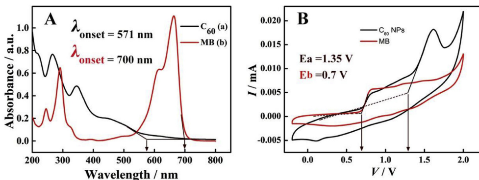
Fig. 2. (A) The UV-vis adsorption spectra of C_{60} NPs (a) and MB (b); (B) The CV measurements of the bare GCE modified by C_{60} NPs and MB in a deoxygenated anhydrous acetonitrile solution (5 mL) containing 0.1 M tetrabutylammonium hexafluorophosphate at 50 mV/s.
