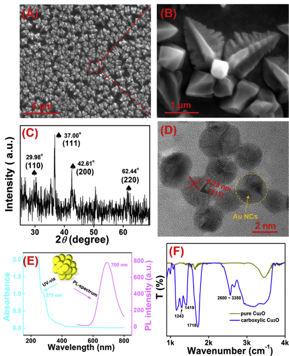
Fig. 1. (A, B) SEM images and (C) XRD pattern of \text{Cu}_2\text{O} films. (D) TEM image, (E) UV-vis absorbance (blue curve), PL spectrum (pink curve) of Au NCs. (F) FTIR spectra of pure \text{Cu}_2\text{O} (green curve) and carboxylic \text{Cu}_2\text{O} (blue curve). (For interpretation of the references to colour in this figure legend, the reader is referred to the Web version of this article.)
