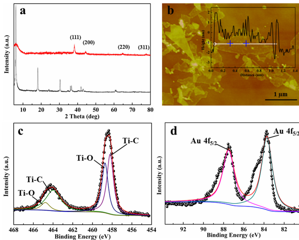
Fig. 2. XRD images of \text{Ti}_3\text{C}_2\text{-MXene} and \text{Ti}_3\text{C}_2\text{-MXene/AuNPs} (a), AFM image of \text{Ti}_3\text{C}_2\text{-MXene} (b) and High-resolution XPS spectra of Ti (c) and Au (d) of \text{Ti}_3\text{C}_2\text{-MXene/AuNPs} composite nanosheets.
