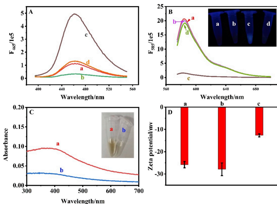
Fig. 2. (A) Fluorescence spectra of SC and (B) Fluorescence spectra of AR. ATCh/MnO 2 NS/SC/AR (a), AChE/MnO 2 NS/SC/AR (b), ATCh/AChE/MnO 2 NS/SC/AR (c), ATCh/AChE/OPs/MnO 2 NS/SC/AR (d). (Inset photograph of the corresponding fluorescence response under UV light.) (C) UV-vis absorption spectra of MnO 2 NS in the (a) absence and (b) presence of AChE. (Inset: the corresponding photos) (D) Zeta-potentials of MnO 2 NS (a), Zeta-potentials of MnO 2 NS in the (b) absence and (c) presence of AChE.
