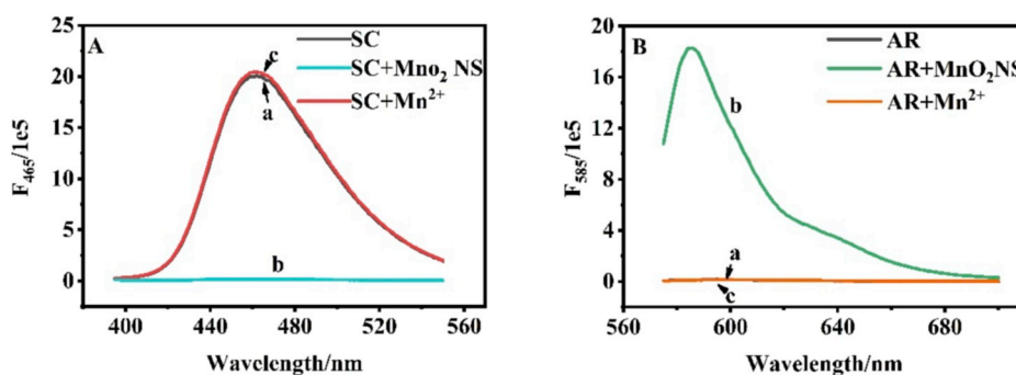
Fig. 1. (A) Fluorescence spectra of SC (a), SC/MnO 2 NS (b) and SC/Mn 2+ (c). (B) Fluorescence spectra of AR (a), AR/MnO 2 NS (b) and AR/Mn 2+ (c).
