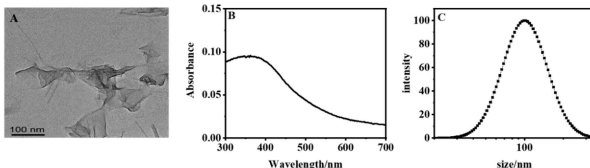
Fig. 3. (A) TEM image of as-synthesized MnO 2 NS; (B) UV-vis absorbance spectra of MnO 2 NS; (C) DLS characterization of the prepared MnO 2 NS.
