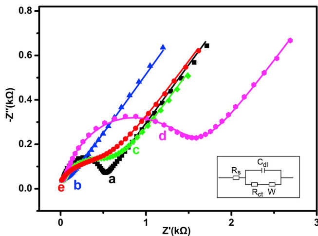
Fig. 2. EIS curves of the bare GCE (a), OMC/GCE (b), cDNA-OMC/GCE (c), aDNA2-cDNA-OMC/GCE (d), and AuNRs-aDNA2-cDNA-OMC/GCE (e); solution: K_3Fe(CN)_6/K_4Fe(CN)_6 (5.0 mM).
