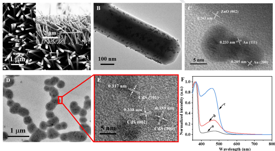
Fig.2 (A) SEM images of ZnO NWs; (B) TEM image and (C) HRTEM image of Au NPs/ZnO NWs; (D) TEM image and (E) HRTEM of CdS QDs@ E. coli aptamer; (F) UV-vis spectra of (a) ZnO NWs, (b) Au NPs/ZnO NWs, (c) CdS QDs@ E. coli aptamer/Au NPs/ZnO NWs.
