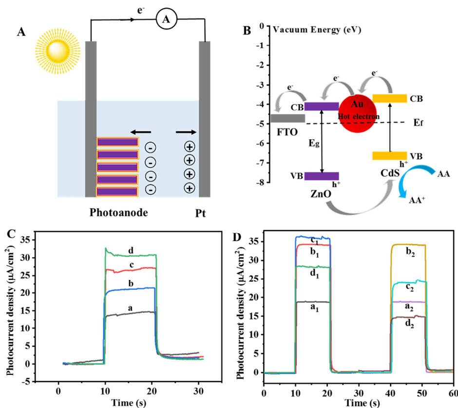
Fig.4 Scheme of the device configuration (A), charge transfer process (B) in the CdS QDs/Au NPs/ZnO NWs electrode; (C) I-T curves. (a) ZnO NWs, (b) CdS QDs/ZnO NWs, (c) Au NPs/ZnO NWs, (d) CdS QDs/Au NPs/ZnO NWs; (D) the assembly process of PEC sensor based on CdS QDs/Au NPs/ZnO NWs and Au NPs/ZnO NWs: (a 1 ) ZnO NWs, (b 1 ) Au NPs/ZnO NWs, (c 1 ) CdS QDs/Au NPs/ZnO NWs and Au NPs/ZnO NWs; (d 1 ) Blocking agent/CdS QDs@ E. coli aptamer/Au NPs/ZnO NWs; (a 2 ) ZnO NWs, (b 2 ) Au NPs/ZnO NWs, (c 2 ) E. coli aptamer/Au NPs/ZnO NWs, (d 2 ) Blocking agent/ E. coli aptamer/Au NPs/ZnO NWs.
