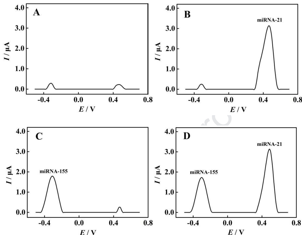
Figure 3. SWV responses of the biosensors: (A) in the absence of miRNA-21 and miRNA-155; (B) in the presence of miRNA-21 and in the absence of miRNA-155; (C) in the absence of miRNA-21 and in the presence of miRNA-155; (D) in the presence of miRNA-21 and miRNA-155.
