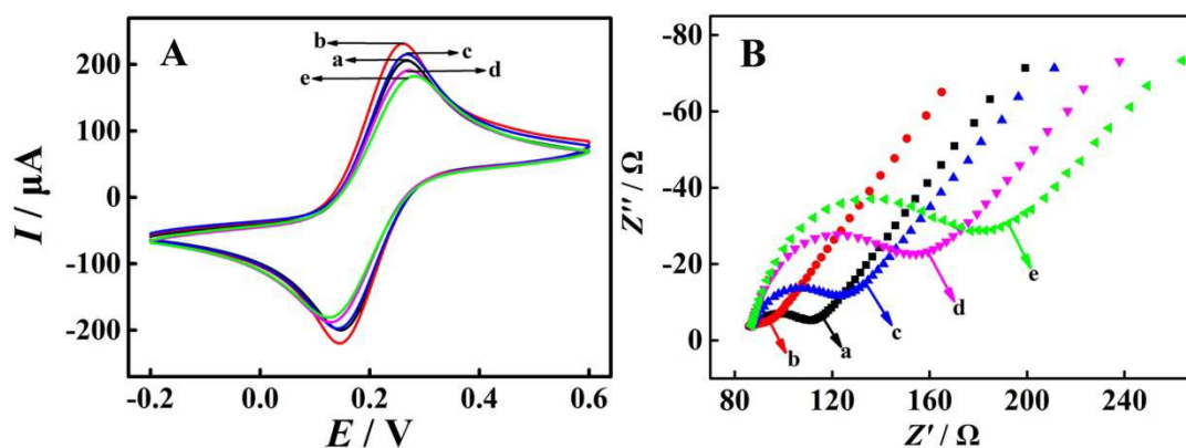
Figure 2. (A) CV and (B) EIS responses of: (a) bare GCE; (b) depAu/GCE; (c) TDN/depAu/GCE; (d) R-R1/TDN/depAu/GCE; (e) Helper1+Helper2/R-R1/TDN/depAu/GCE.
