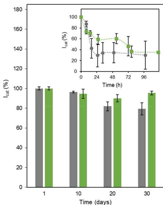
Fig. 4. Stability of wt (gray) and 29E4 PpDyP/SAM/Ag (green) electrodes response to \text{H}_2\text{O}_2 . Relative catalytic current response to 50 \mu\text{M} \text{H}_2\text{O}_2 , during storage at 4^\circ\text{C} for 1 month (shelf-life) measured on a batch of electrodes prepared on the same day ( n = 16 ). Inset: relative catalytic current measured using the same electrode ( n = 4 ) during a 5 day period. (For interpretation of the references to color in this figure legend, the reader is referred to the Web version of this article.)
