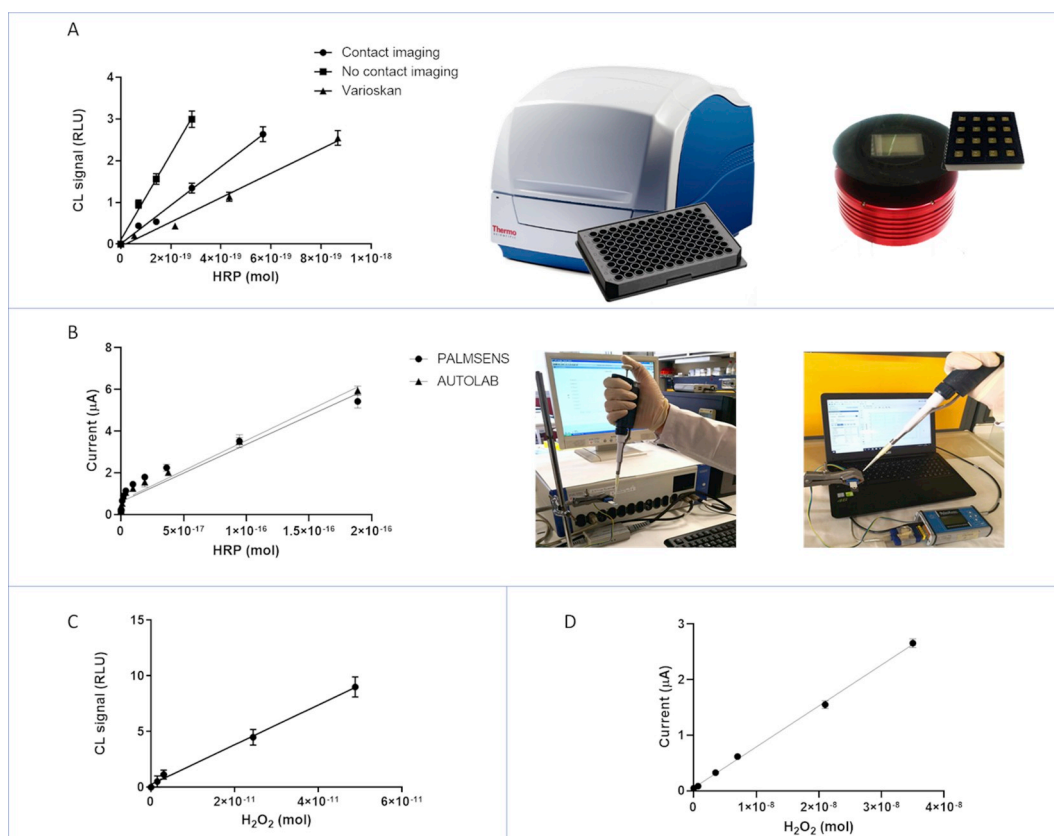
Fig. 4. A) Calibration curve of HRP by CL-based detection, employing the Varioskan bench-top instrumentation (triangles) or the cooled CCD-based portable device employed in the contact (circle) or optics-based (squares) configuration. B) Calibration curve of HRP using electrochemical sensor based on SPE modified with CB and portable instrument (blue line) or laboratory benchtop instrumentation (black line). C) CL calibration curve of H 2 O 2 using laboratory benchtop Varioskan instrumentation. D) Calibration curve of H 2 O 2 using laboratory benchtop instrumentation and SPE modified with CB/PBNPs. (For interpretation of the references to color in this figure legend, the reader is referred to the Web version of this article.)
