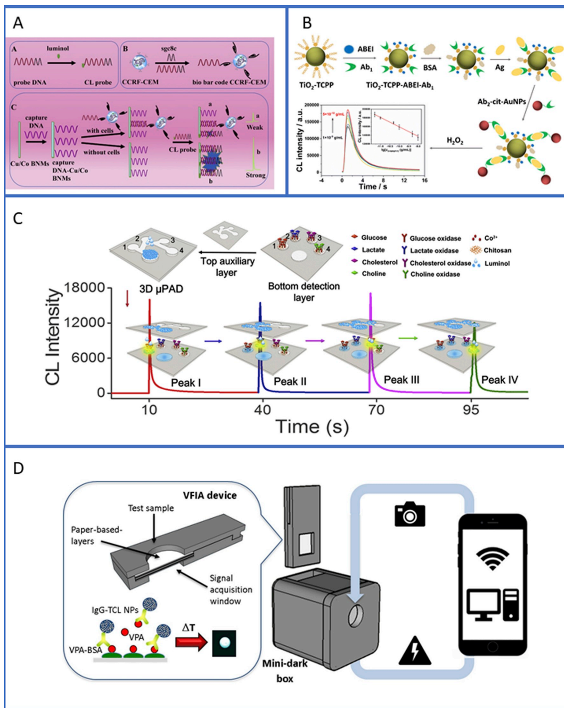
Fig. 1. Examples of different strategies for improving luminescence quantum yield and innovative CL-based analytical formats. A) Cu/Co bimetallic nanomaterials, employed as the nanocatalysts for the CL reaction, enabling detection of cancer cells down to 270 \text{ cells mL}^{-1} in an aptamer-based assay (Li et al., 2018); B) Turn-off CRET-based sandwich immunoassay exploiting \text{TiO}_2 NPs functionalized with a porphyrin derivative and N-(4-aminobutyl)-N-ethylisoluminol ( \text{TiO}_2\text{-TCPP-ABEI} nanoluminophores) as CL emitter and AuNPs as energy acceptor (Shu et al., 2019); C) a double-layered three-dimensional (3D) microfluidic network was exploited for temporizing reagents delivery, thus developing a multiplex CL enzyme assay for detecting glucose, lactate, choline, and cholesterol (Li et al., 2019); D) Smartphone-based thermochemiluminescent immunosensor for valproic acid detection (Roda et al., 2019).
