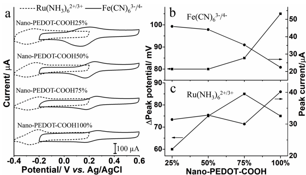
Fig. 2. (a) Cyclic voltammograms of different Nano-PEDOT-COOH modified electrodes in 2 mM \text{Fe(CN)}_6^{3-/4-} (solid curve), \text{Ru(NH}_3)_6^{2+/3+} (dashed curve) in 0.1 M KCl; Corresponding redox peak potential and peak current of different Nano-PEDOT-COOH modified electrodes to 2 mM \text{Fe(CN)}_6^{3-/4-} (b) and \text{Ru(NH}_3)_6^{2+/3+} (c) in 0.1 M KCl. Scan rate of 50 \text{mV s}^{-1} .
