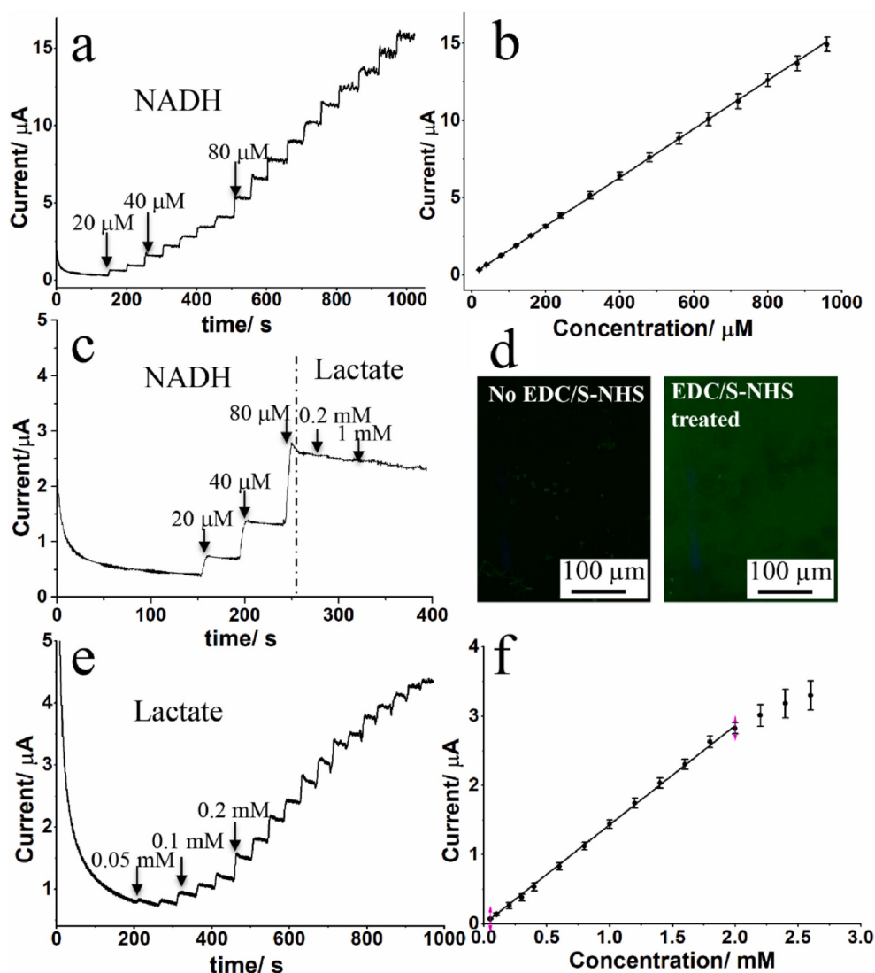
Fig. 5. (a) Current-time response curve of EA-neutralised Nano-PEDOT-COOH50% at 0.420 V for successive injections of NADH in 0.1 M PBS (pH 7.4); (b) Corresponding calibration curve for NADH sensing, n = 3 ; (c) Current-time response curve of EA-neutralised Nano-PEDOT-COOH50% at 0.420 V for varying concentration of NADH and lactate; (d) Fluorescence microscopy image of a FITC-BSA Bio-Nano-PEDOT interface without (left) and with (right) treatment; (e) Current-time response curve of LDH-Nano-PEDOT at 0.450 V for successive injection of lactate in 0.1 M PBS (pH 7.4); (f) Corresponding calibration curve for lactate biosensing, n = 3 .
