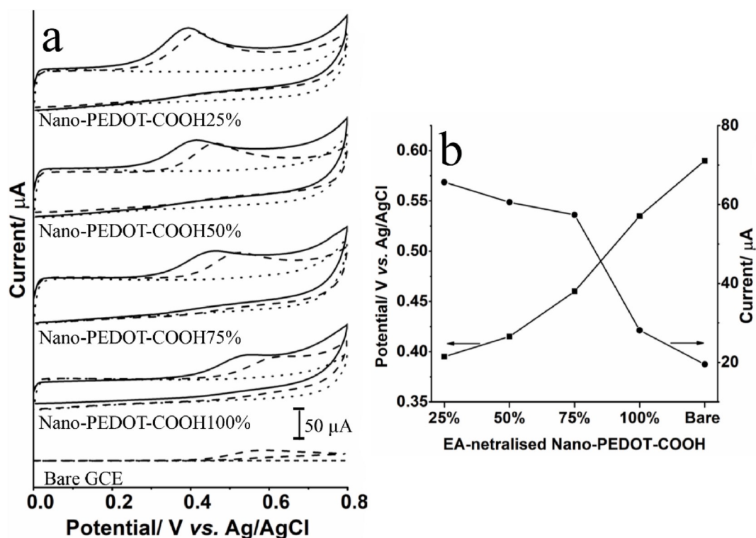
Fig. 4. (a) CV responses of different Nano-PEDOT-COOH modified electrodes with (dash: un-neutralised, solid: EA-neutralised) and without (dotted line) 2 mM NADH in 0.1 M PBS (pH = 7.4); (b) Corresponding NADH oxidation peak potentials and peak currents of EA-neutralised Nano-PEDOT-COOH modified electrodes to 2 mM NADH in 0.1 M PBS (pH = 7.4). Scan rate of 50 mV s -1 .
