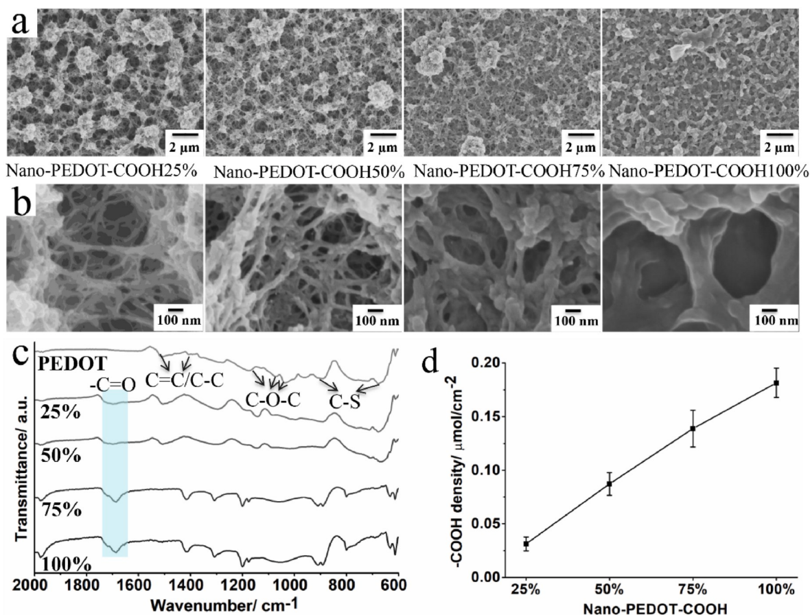
Fig. 1. (a) SEM images of Nano-PEDOT-COOH with different amounts of EDOT-COOH ranging from 25 to 100%; (b) High magnification SEM images; (c) FTIR spectra of PEDOT and nano-PEDOT-COOH25–100%; (d) Carboxylic acid density on Nano-PEDOT-COOH25–100% surface estimated by the TBO staining technique.
