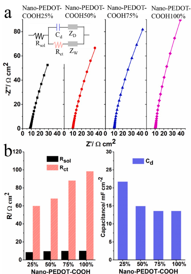
Fig. 3. (a) EIS analysis of different Nano-PEDOT-COOH modified electrodes in Nyquist plots obtained in 2 mM \text{Fe}(\text{CN})_6^{3-/4-} in 0.1 M KCl, inset is the equivalent circuits; (b) Corresponding curve fitting parameters.
