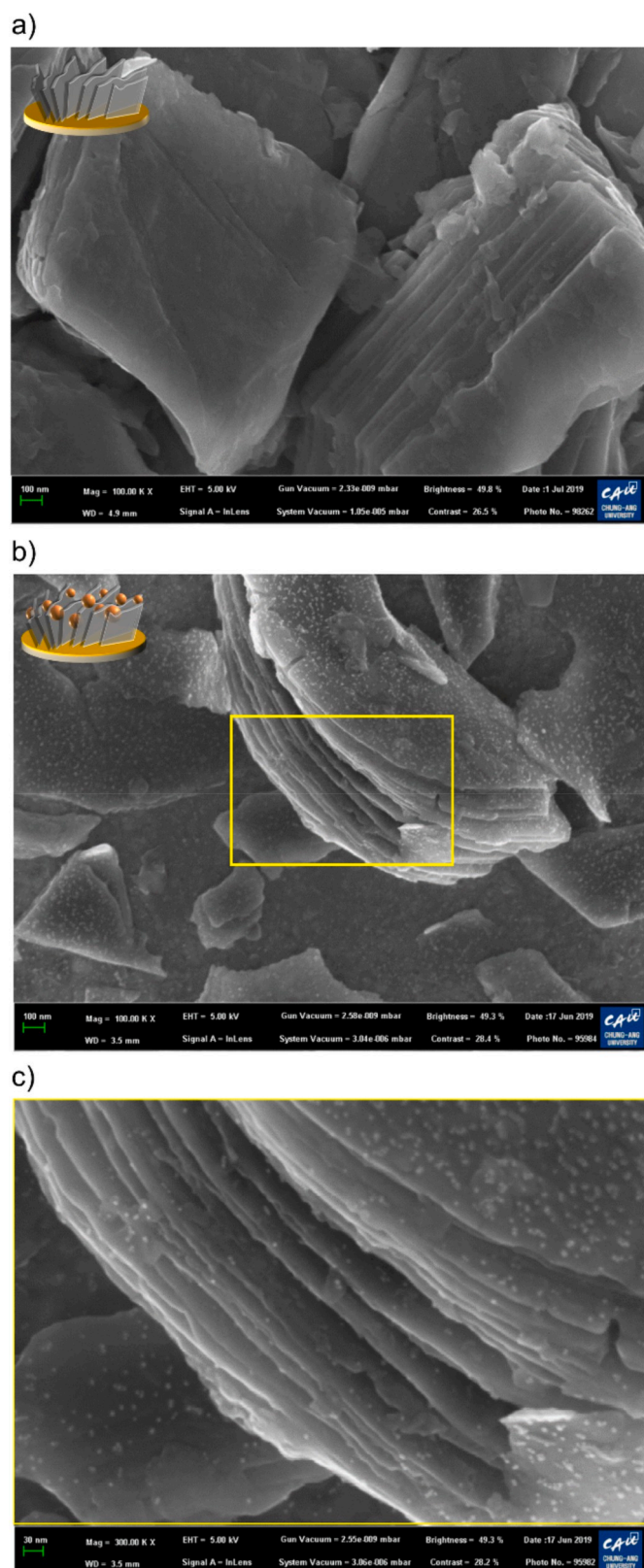
Fig. 2. FE-SEM images of: a) As-synthesized MXene-Ti 3 C 2 T x , b) AuNP@MXene, and c) Magnified image from the boxed region in (b); White dots represent the 5 nm AuNPs.
