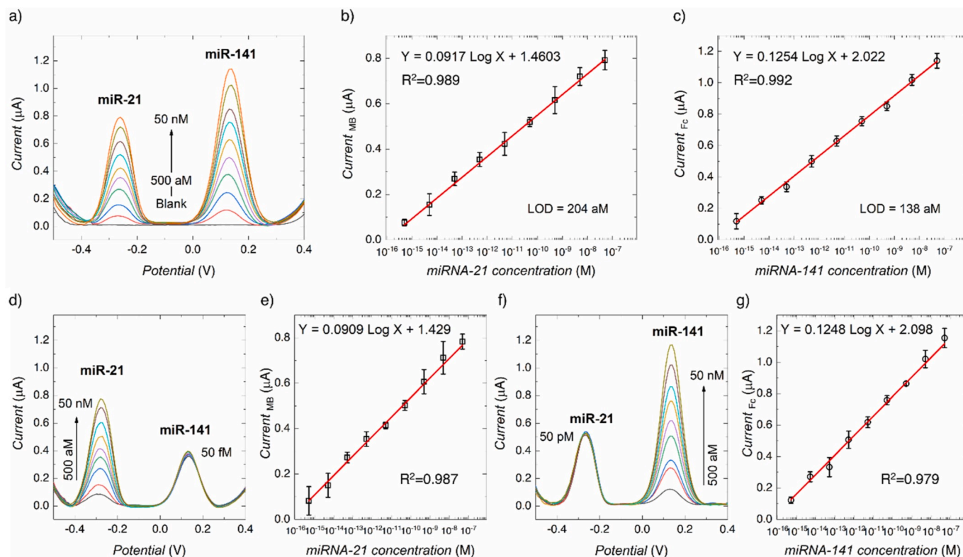
Fig. 4. a) Typical DPV response of the fabricated biosensor device toward multiple detection of serial concentrations of miR-21 and miR-141 (0, 500 aM, 5 fM, 50 fM, 500 fM, 5 pM, 50 pM, 500 pM, 5 nM and 50 nM) in HEPES buffer (pH 7.4). b) and c) Corresponding regression plot illustrating the oxidation current peak values of MB and Fc as a function of miR-21 and miR-141 concentrations, respectively. d) Representative DPV response of the fabricated biosensor device toward single target detection of serial concentrations of miR-21 and constant value of miR-141 (50 fM). e) Plotting the MB oxidation current peak values as a function of miR-21 concentration. f) Typical DPV response of the fabricated biosensor device toward single target detection of serial concentrations of miR-141 and constant value of miR-21 (50 pM). g) Plotting the Fc oxidation current peak values as a function of miR-141 concentration. Statistical data was attained from eight different samples under equal conditions. The DPV curves are shown after baseline subtraction.
