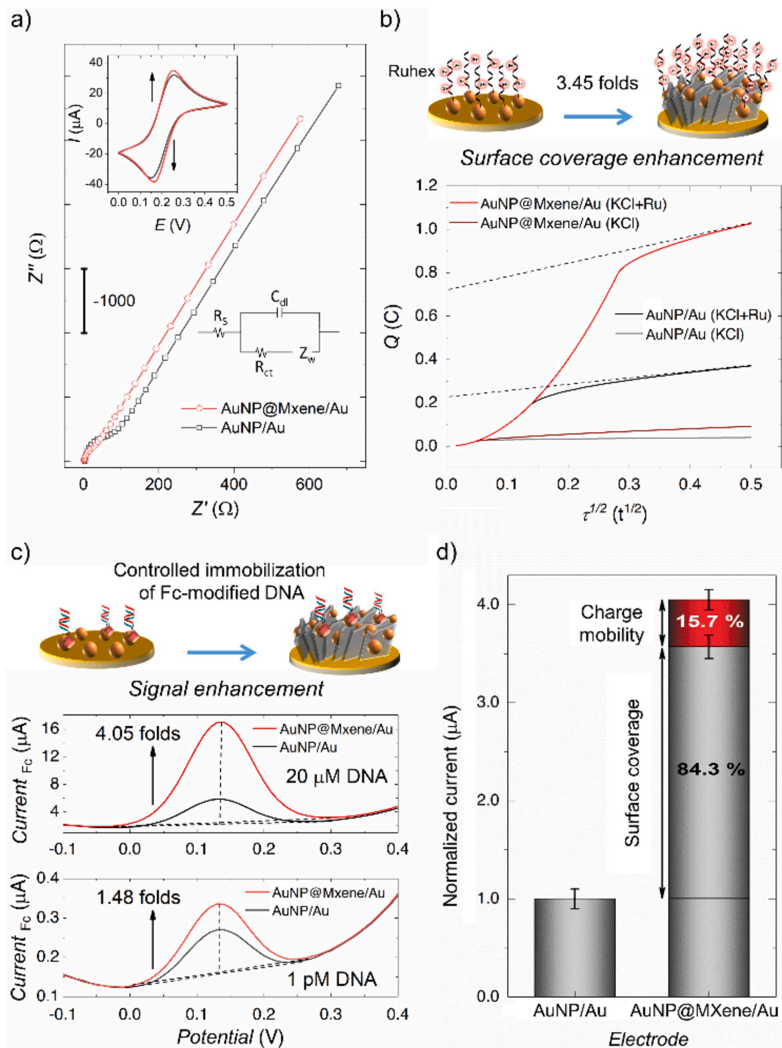
Figure 3. a) Nyquist plots ( Z' vs. -Z'' ) obtained for AuNP/Au and AuNP@MXene/Au and the equivalent Randles circuit model; Inset shows the corresponding cyclic voltammograms of AuNP/Au (black) and AuNP@MXene/Au (red); Experiments were performed in PBS (pH 7.4) comprising 5 mM of \text{Fe}(\text{CN})_6^{4-/3-} and 0.1 M KCl with CV scan rate of 50 mV/s. b) Typical chronocoulometric response of RuHex on AuNP/Au and AuNP@MXene/Au in 20 mM KCl and hexaammineruthenium(iii) chloride (200 \mu\text{M} ) + KCl (20 mM); Dash lines show the outward stretching tangents extrapolated to the Y-axis illustrating the intercept values. c) DPV curves obtained for Base 141 /AuNP/Au and Base 141 /AuNP@MXene/Au after being hybridized with uncleaved Fc-labeled DNA sequences (DSN products of 20 \mu\text{M} and 1 pM miR-141 reaction). d) Statistical analysis of the normalized oxidation current peak value of Fc obtained from Fig. 3c.
