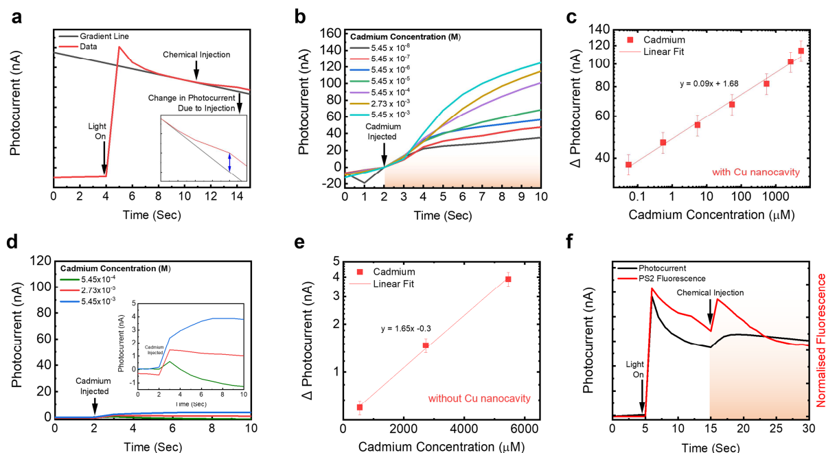
Figure 3. Demonstration of nanocavity-enhanced metal ion sensing with photocurrents. (a) Photocurrent measured from Chlorella sp. (red line) in the copper nanocavity microfluidic device. At t=4 , the violet light is turned on where the photocurrent quickly rises. At t=11 , metal ions are injected, and the photocurrent increases again. The measurement is defined as the difference between photocurrent and the gradient line (black line) as shown in the inset. The gradient is defined by the nominal response in the absence of injected metal ions. Inset: a closeup illustrating the measured difference between the red and black lines. (b) Normalized photocurrent with nanocavity enhancement after injection of different concentrations of cadmium metal ions ( \text{CdCl}_2 ). The injection occurs at t=2 , and the photocurrent rises proportionally to the concentration of the metal ions. (c) Summary of photocurrent increment vs. cadmium concentration (with nanocavity), both on a logarithmic scale with a standard fitting curve. The dots were based on the averages of several curves ( N=3 ). (d) Normalized photocurrent without nanocavity enhancement after injection of extremely high concentrations of cadmium metal ions. (e) Summary of photocurrent increment vs cadmium concentration (without nanocavity), both on a logarithmic scale with a standard fitting curve. ( N=3 ). (f) Photocurrent and photosystem fluorescence measured in parallel from the nanocavity microfluidic device. The metal ions are then injected at 15 seconds and quickly interact with the algae, resulting in further increases in the fluorescence and photocurrent. Violet LED excitation: 375 nm-450 nm. Average light intensity: 30 \text{ W/m}^2 .
