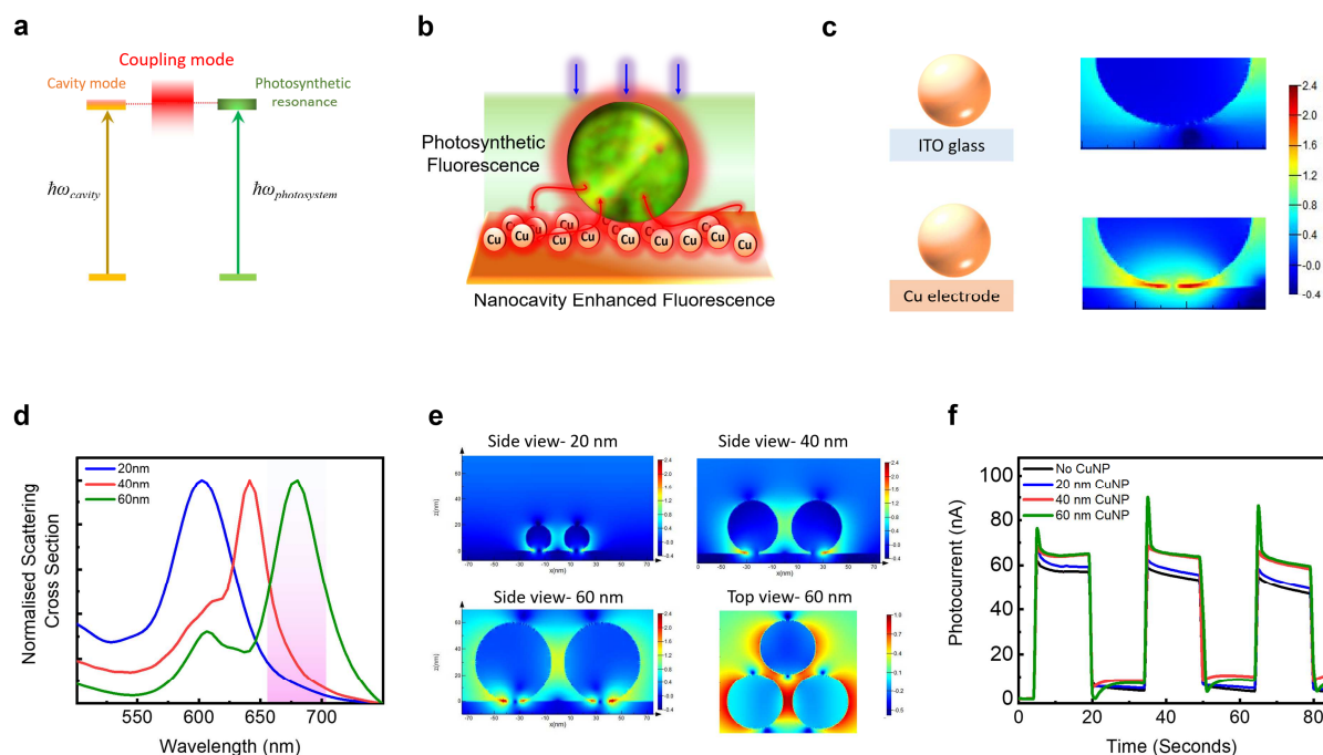
Figure 2. Principle of nanocavity-enhanced photoelectrochemistry with Cu nanoparticles. (a) Energy coupling diagram between nanocavity and photosynthetic fluorescence. (b) Schematic showing the nanocavity-enhanced fluorescence when Chlorella sp. undergo violet light excitation. Fluorescence emission from the photosystem will resonance with the CuNPs and reflect back to the microalgae. (c) Top: Electric field distribution of 60 nm CuNPs placed above an ITO glass substrate at a wavelength of 680 nm. Bottom: Electric field distribution of 60 nm CuNPs placed on Cu electrode at a wavelength of 680 nm. (d) Optical simulated normalized scattering cross-section of aggregated CuNPs on Cu thin film. Normalized intensity for three copper nanoparticles of sizes 20 nm, 40 nm and 60 nm. The pink area between 660-710 nm shows the resonance regime. (e) Electric field distribution of 20/40/60 nm CuNPs at the resonant wavelength of 680 nm. The side view shows the near-field enhancement due to Fabry-Perot nanocavity formed between the CuNPs and underneath Cu tape. The top view of 60 nm shows the improvement due to the interaction of Cu nanoparticles among themselves. (f) Photocurrent measured overtime from Chlorella sp. with 20nm, 40nm, and 60nm copper nanoparticles in the copper nanocavity microfluidic device and illuminated with violet light. Three intervals are shown with the violet light being turned on and off for 15 seconds each interval.
