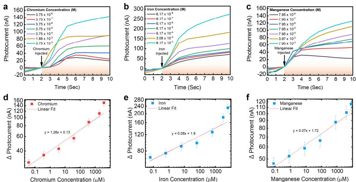
Figure 4. Ultra-low concentration detection of heavy and light metal ions. (a) Normalized photocurrent with nanocavity enhancement after injection of different concentrations of chromium metal ions ( \text{CrCl}_3 \cdot 6\text{H}_2\text{O} ). (b) Normalized photocurrent with nanocavity enhancement after injection of different concentrations of iron metal ions ( \text{FeCl}_3 ). (c) Normalized photocurrent with nanocavity enhancement after injection of different concentrations of manganese metal ions ( \text{MnCl}_2 ). (d) Summary of photocurrent increment vs. chromium concentration on a logarithmic scale. (e) Summary of photocurrent increment vs. iron concentration on a logarithmic scale. (f) Summary of photocurrent increment vs. manganese concentration on a logarithmic scale. For all three experiments, the injection occurs at t=2 , and the photocurrent rises proportionally to the concentration of the metal ions. The dots were based on the averages of several curves ( N=3 ) for each concentration. The fitting standard curves and formula for (a-c) are plotted in (d-f), respectively. Violet LED excitation: 375 nm-450 nm. Average light intensity: 30 \text{ W/m}^2 .
