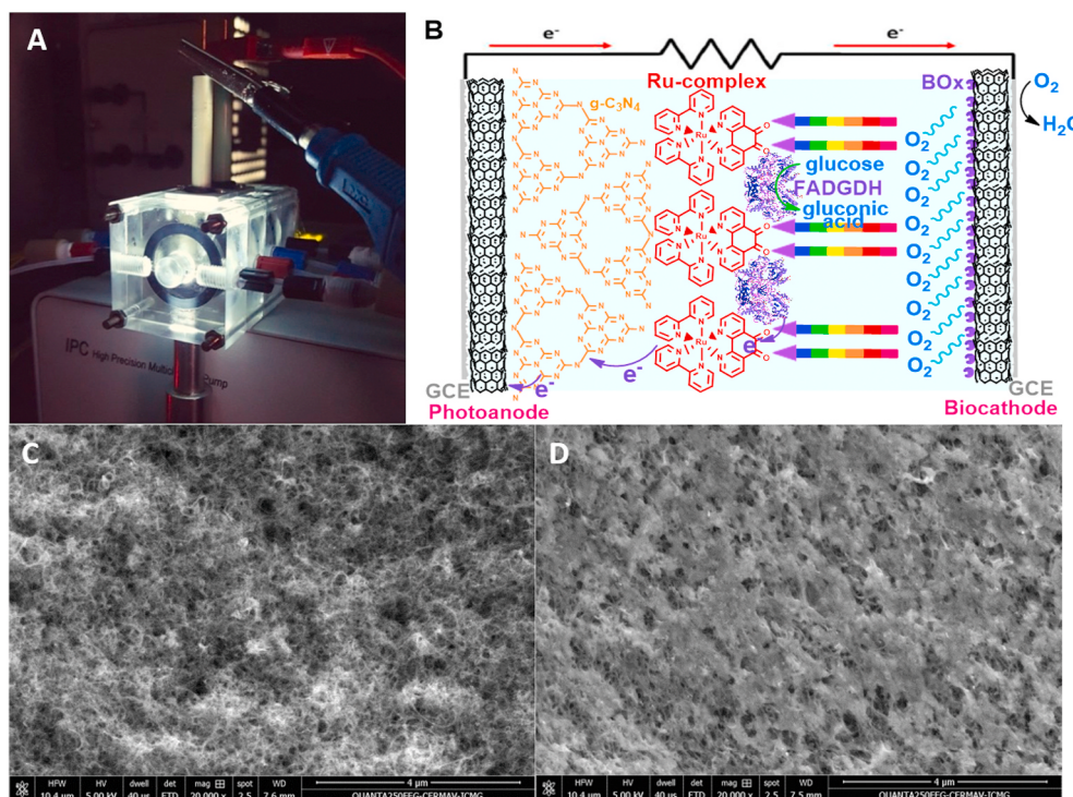
Fig. 1. The photograph of PBFC during operation (A); the schematic illustration of the PBFC principle (B); SEM image of GCE|MWCNT (C) and GCE|MWCNT|g-C 3 N 4 |Ru complex (D).
