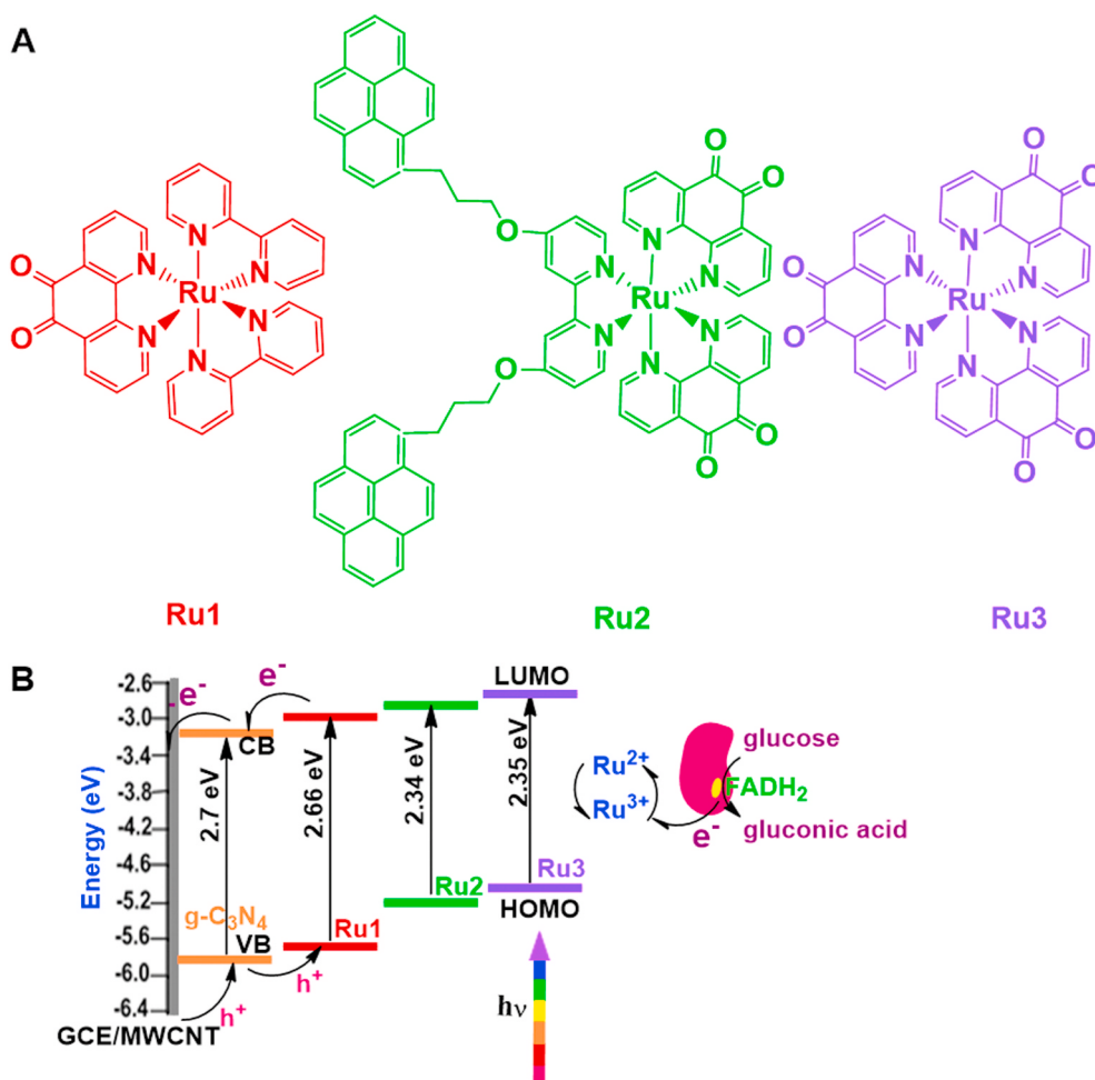
Scheme 1. Ru(II) complexes (counter ions: \text{PF}_6^- ) (A); Schematic illustration of light-driven electron-transfer cascade with the energetic levels of photoactive materials (B).
