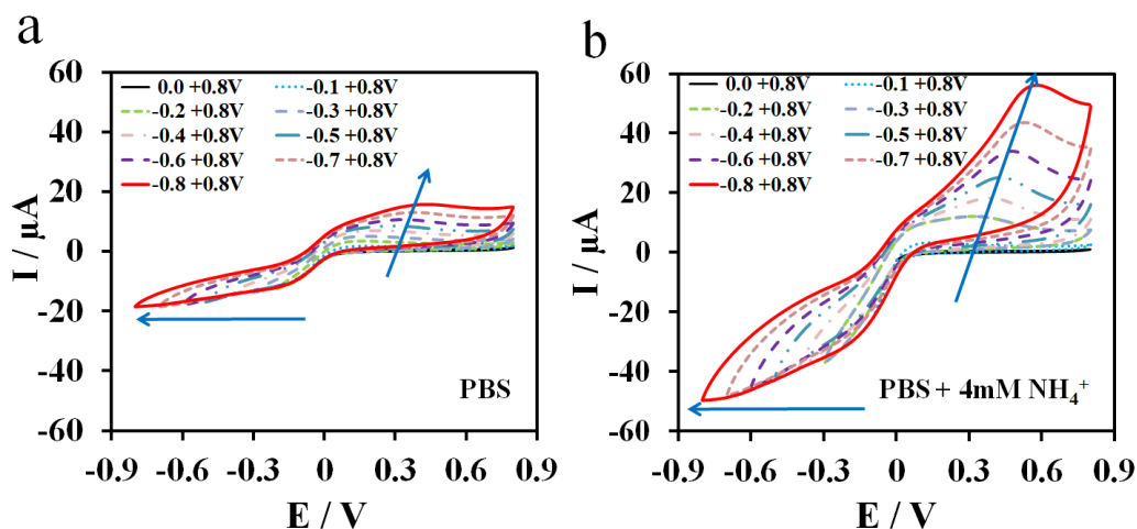
Fig. 3. The effect of potential range on doping/de-doping degree of the nano-PANI:PSS n in (a) 10 mM PBS and (b) 10 mM PBS containing 4 mM NH 4 + , scan rate of 50 mV s -1 .
