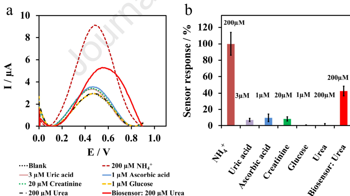
Fig. 5. (a) Selectivity study of GCE/PANI:PSS n electrode with respect to normal interfering species in urine; (b) Standardised current response for different interfering species.
