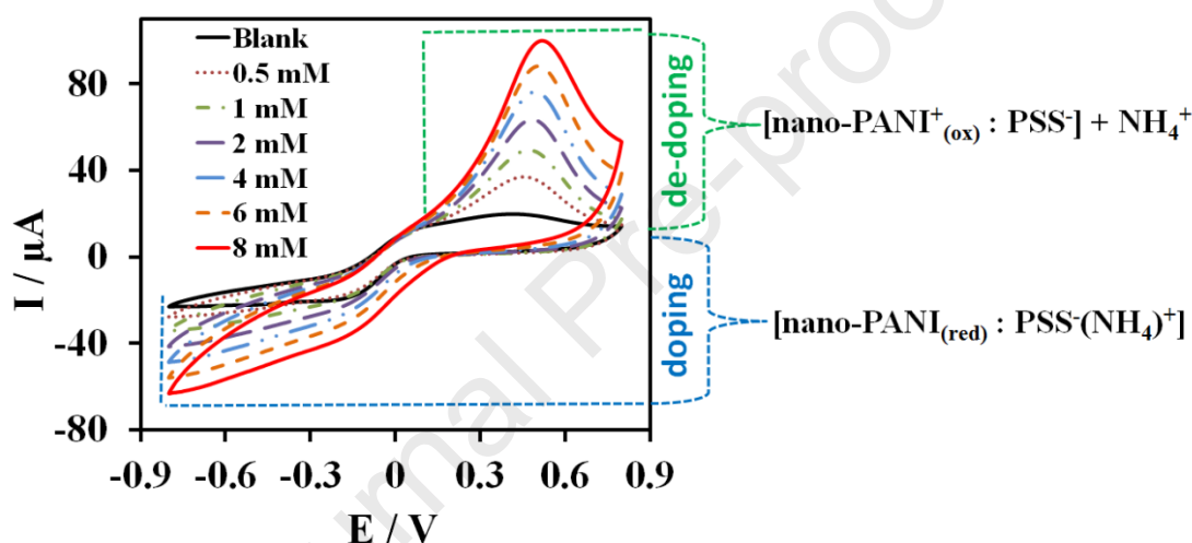
Fig. 2. Sensing mechanism of nano-PANI:PSS n electrode to \text{NH}_4^+ characterised by CVs response different concentration of \text{NH}_4^+ (0, 0.5, 1, 2, 4, 6, 8 mM) in 10 mM PBS (pH 7), scan rate of 50 \text{mV s}^{-1} .
