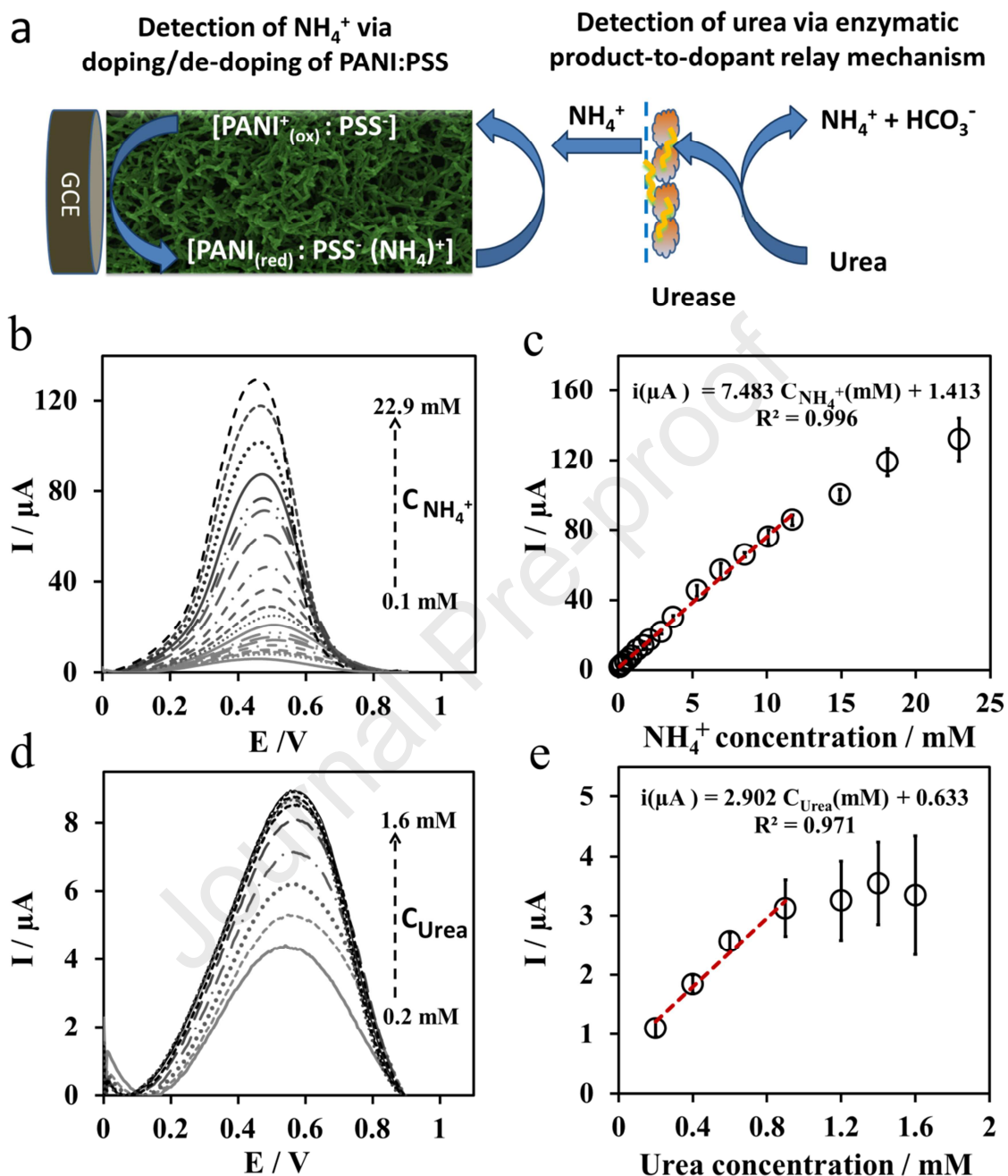
3 4 Fig. 4. (a) Schematic illustrating the \text{NH}_4^+ sensing mechanism of the nano-PANI:PSS n sensor and the 5 coupling of the enzyme urease with nano-PANI:PSS n as a urea biosensor with an innovative catalytic 6 product-to-dopant relay mechanism; (b) the SWV responses of nano-PANI:PSS n sensor towards 7 successive addition of \text{NH}_4^+ in 10 mM PBS (pH 7); (c) corresponding calibration curve for \text{NH}_4^+ 8 sensing, n = 3 ; (d) SWV response of nano-PANI:PSS n /CPM-urease biosensor towards successive 9 addition of urea in 10 mM PBS (pH 7); (e) corresponding calibration curve for urea biosensing, n = 3 .
