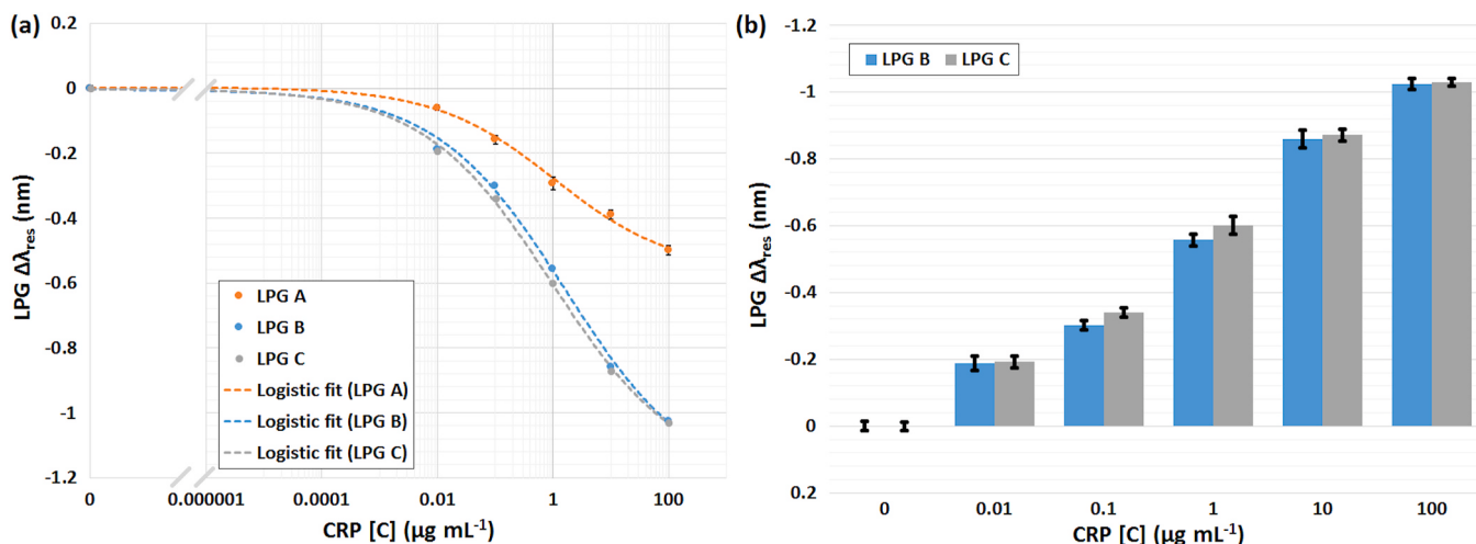
Fig. 8. (a) Semi-log calibration curves of LPG-A (orange), LPG-B (blue) and LPG-C (grey), obtained from the respective sensorgrams of Fig. 7. Each concentration of CRP (circles) is expressed in terms of the mean value and the respective standard deviation within 20 measurements showed for LPG-A (black error bars). The dashed curves (orange for LPG-A, blue for LPG-B and grey for LPG-C) represent the fitting of the experimental data by using the Logistic function. (b) Comparative histogram of the results attained for the detection of CRP with two independent and repeated experiments using LPG-B (blue) and LPG-C (grey). Each column represents the mean value of the signal, together with the respective standard deviation within 20 measurements (black error bars). (For interpretation of the references to color in this figure legend, the reader is referred to the Web version of this article.)
