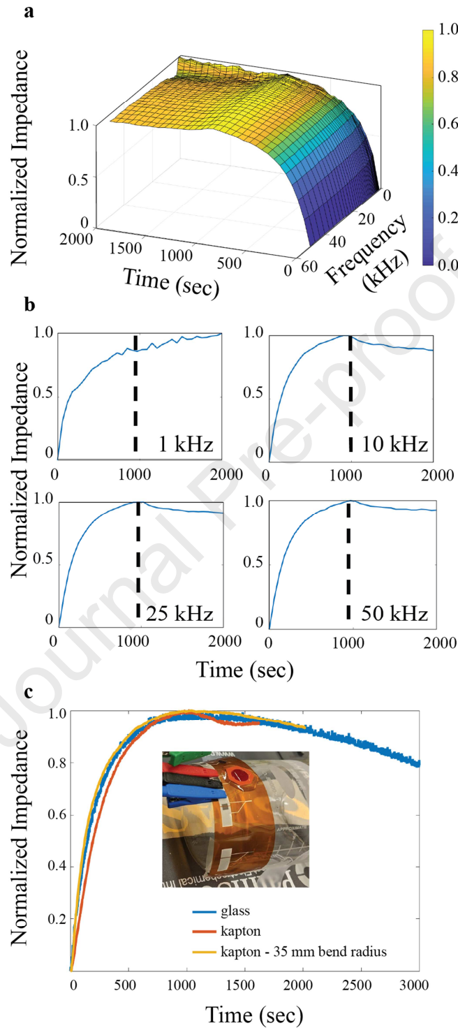
Figure 2. Impedance-based coagulation testing of chicken blood with printed biosensors. a) Response from sensors tested at frequencies ranging from 1 to 50 kHz over the course of a complete clotting test, revealing the unstable response at sub-10 kHz frequencies. b) Single frequency cross-sections of the full data in a) at 1 kHz (top left), 10 kHz (top right), 25 kHz (bottom left), and 50 kHz (bottom right). c) PT tests at 15 kHz using printed biosensors on
