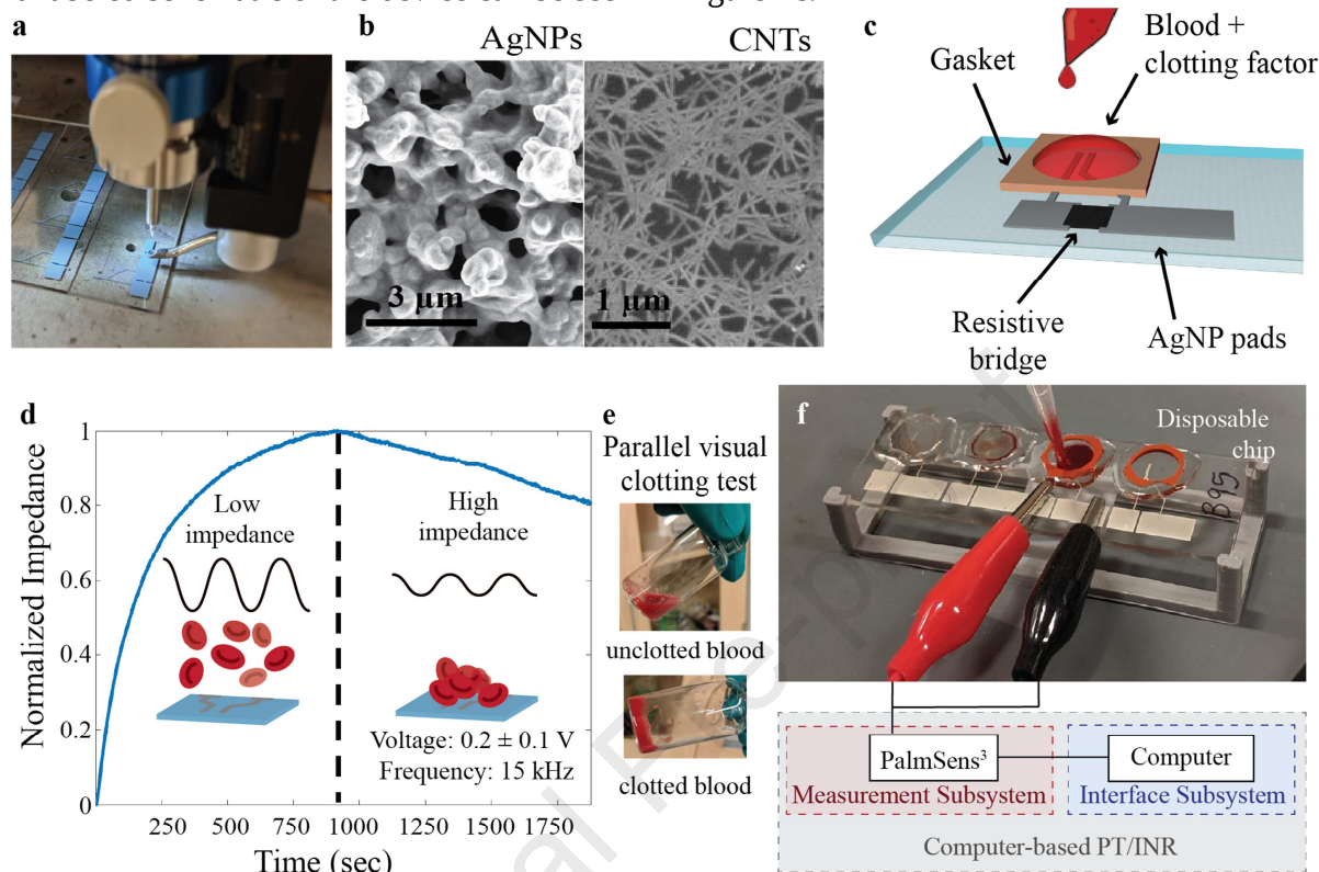
Figure 1: Printed prothrombin time device fabrication and testing. a) AJ printing of AgNPs for PT/INR device. b) SEM images of (left) AgNP electrode and (right) unsorted carbon nanotube conductive resistive bridge. c) Schematic of device design. d) Representative impedance curve illustrating coagulation test for chicken blood with e) a parallel visual clotting test. The dashed line represents the clotting time as determined by the impedance maximum and the gelatinization of the blood. Before the blood clots, the red blood cells are floating in solution (d – left insert, e - top) and thus the impedance is low; as the blood clots, the red blood cells deposit onto the device and cause the impedance to increase (d – right insert, e - bottom), maximizing at the point of clotting. (f) Picture of testing setup showing blood addition to the sensor and schematic of computer-based impedimetric testing interface.
