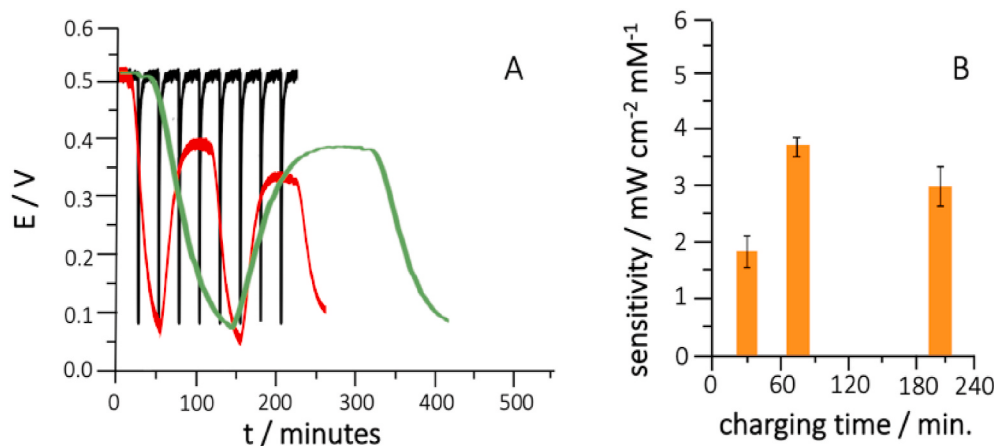
Fig. 5. (A) Charge/discharge curve of self-charging FDH/PABA/MWCNT/G-CSC||CSC-G/MWCNT/2-ANT/TvL BSC; discharge was carried out by applying a pulse current of 100 μA for 3 s (black curve), constant load of 250 Ω for 50 mins and self-charging for 70 mins (red curve), constant load of 250 Ω for 100 mins and self-charging for 200 mins (green curve). Experimental conditions: 50 mM NaAc pH 5 containing 20 mM D-Fructose and air-equilibrated. (B) Sensitivity calculated from the calibration curve measured for the self-charging BSC working as self-powered biosensor upon different charging times. (For interpretation of the references to color in this figure legend, the reader is referred to the Web version of this article.)
