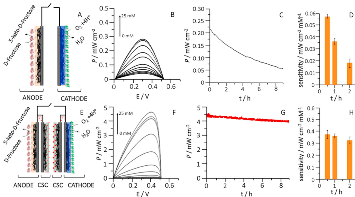
Fig. 4. (A) Schematic representation of EFC: FDH/PABA/MWCNT/G||G/MWCNT/2-ANT/TvL (B) Power output profiles recorded for FDH/PABA/MWCNT/G||G/MWCNT/2-ANT/TvL EFC in 50 mM NaAc buffer pH 5 containing different concentrations of D-Fructose from 0 mM up to 25 mM and in equilibrium with air (source of O 2 ). The plot was obtained from linear sweep voltammetry at 1 mV s -1 . (C) Power output trend of EFC upon 8 working hours applying a constant load of 250 Ω. (D) Sensitivity calculated from the calibration curve measured for the EFC working as self-powered biosensor upon operation time. (E) Schematic representation of BSC: FDH/PABA/MWCNT/G-CSC||CSC-G/MWCNT/2-ANT/TvL (F) Power output profiles recorded for FDH/PABA/MWCNT/G-CSC||CSC-G/MWCNT/2-ANT/TvL BSC in 50 mM NaAc buffer pH 5 containing different concentrations of D-Fructose from 0 mM up to 25 mM and in equilibrium with air (source of O 2 ). The plot was obtained from linear sweep voltammetry at 1 mV s -1 . (G) Power output trend of BSC upon 8 working hours applying a constant load of 250 Ω. (H) Sensitivity calculated from the calibration curve measured for the BSC working as self-powered biosensor upon operation time.
