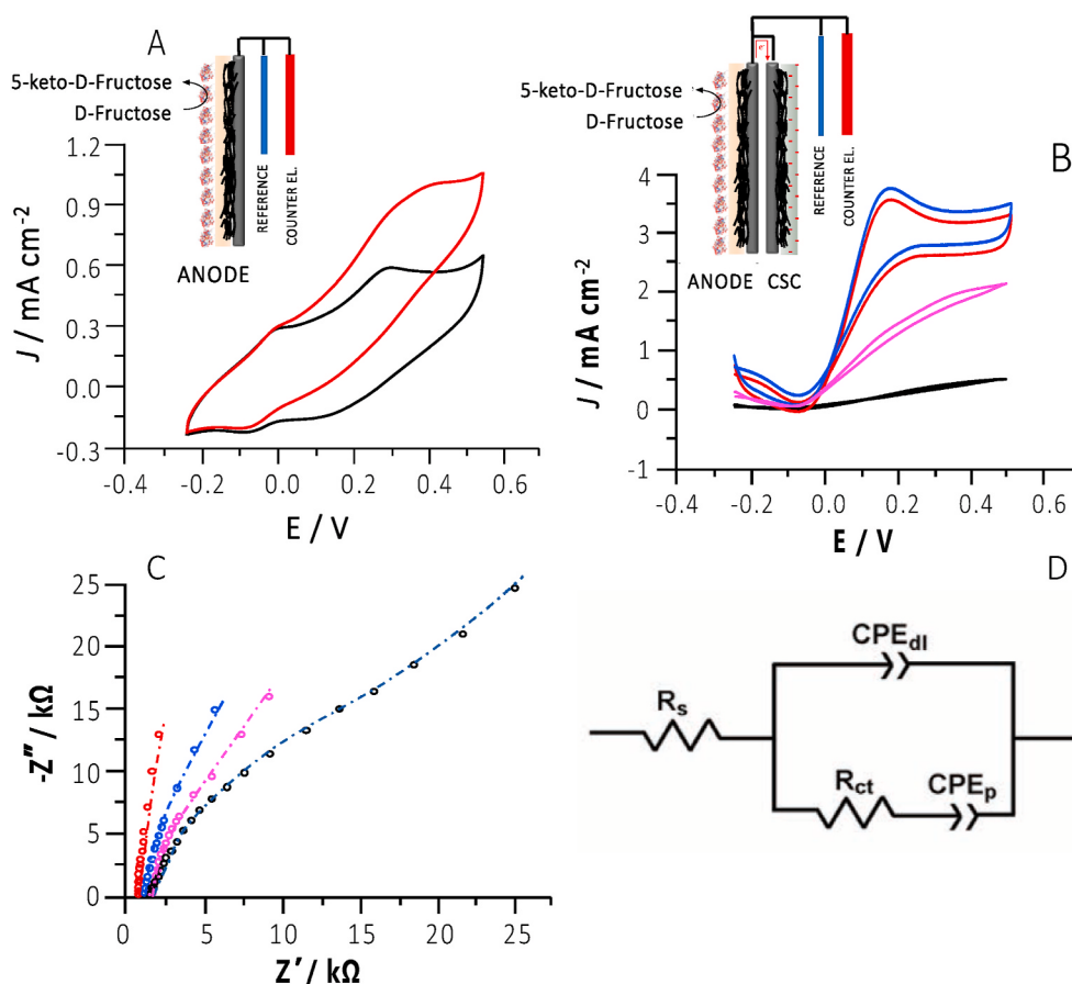
Fig. 3. (A) CVs of FDH/PABA/MWCNT/G in absence (black curve) and in presence of 10 mM D-Fructose (red curve). (B) Subtracted CVs for FDH/PABA/MWCNT/G supercapacitive electrode (SCP, black curve) and SCP containing charge storing components (CSCs) of 0.5 (magenta curve), 1.2 (blue curve) and 2 (red curve) mF in presence of 10 mM D-Fructose. Experimental conditions: 50 mM NaAc buffer at pH 5, scan rate 5 \text{ mV s}^{-1} , T = 25^\circ \text{C} . (C) Experimental (dots) and modeled (dashed curves) Nyquist plots at 0.4 V for FDH/PABA/MWCNT/G supercapacitive electrode (SCP, black curve) and SCP containing CSCs of 0.5 (magenta curve), 1.2 (blue curve) and 2 (red curve) mF. (D) Equivalent circuit model used to fit the EIS spectra reported in (C). (For interpretation of the references to color in this figure legend, the reader is referred to the Web version of this article.)
