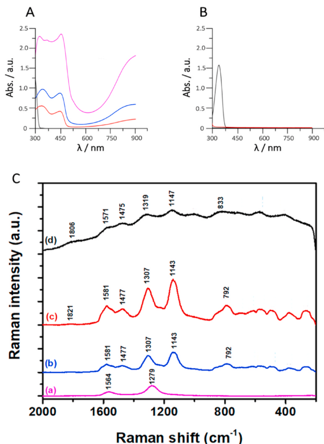
Fig. 2. (A) UV-Vis spectra of PANI electropolymerized onto ITO electrodes in 1 M H 2 SO 4 : aniline monomer (black curve), PANI t exp = 200 s (red curve), PANI t exp = 400 s (blue curve) and PANI t exp = 600 s (magenta curve); Optimal experimental conditions of PANI electropolymerization: [ANI] = 0.1 M, E ox = 0.9 V vs. Ag|AgCl (3M KCl), t ox = 0.4 s, E red = -0.1 V vs. Ag|AgCl (3M KCl), t red = 0.2 s and t exp = 300 s. (B) PABA electropolymerized onto ITO electrodes in 1 M H 2 SO 4 : 2-aminobenzoic acid monomer (black curve), PABA t exp = 300 s (red curve). Optimal experimental conditions of PABA electropolymerization: [ABA] = 0.1 M, E ox = 0.7 V vs. Ag|AgCl (3M KCl), t ox = 0.4 s, E red = -0.1 V vs. Ag|AgCl (3M KCl), t red = 0.2 s and t exp = 300 s. (C) Raman spectra of (a, magenta curve) MWCNT/G, λ exc = 514 nm, (b, blue curve) PANI t exp = 200 s/MWCNT/G, (c, red curve) PANI t exp = 400 s/MWCNT/G and (d, black curve) PANI t exp = 600 s/MWCNT/G, λ exc = 784 nm for PANI/MWCNT/G. (For interpretation of the references to color in this figure legend, the reader is referred to the Web version of this article.)
