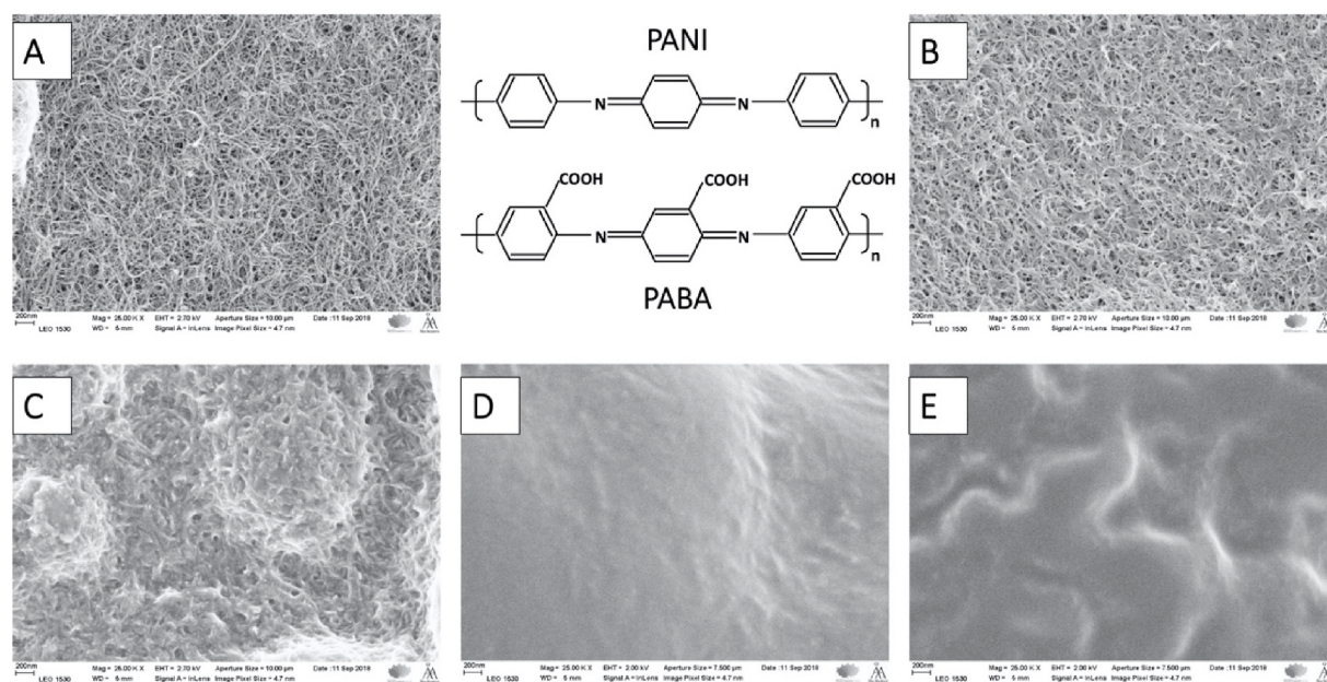
Fig. 1. The chemical structures for PANI and PABA and SEM images of (A) MWCNT/G (accelerating voltage: 2.7 kV), (B) PABA/MWCNT/G, (C) PANI/MWCNT/G with t_{\text{exp}} = 200 s, (D) PANI/MWCNT/G with t_{\text{exp}} = 400 s and (E) PABA/MWCNT/G with t_{\text{exp}} = 600 s (only for D and E accelerating voltage: 2.0 kV).
