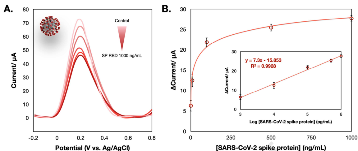
Figure 5. (A) SWV responses of the COVID-19 ePAD tested with different concentrations of the SARS-CoV-2 spike protein in the presence of 5 mM [\text{Fe}(\text{CN})_6]^{3-/4-} . (B) The relationship between \Delta\text{current} and concentration of SARS-CoV-2 spike protein; the inset shows its corresponding calibration plotted between the \Delta\text{current} and logarithmic concentration of the SARS-CoV-2 spike protein.
