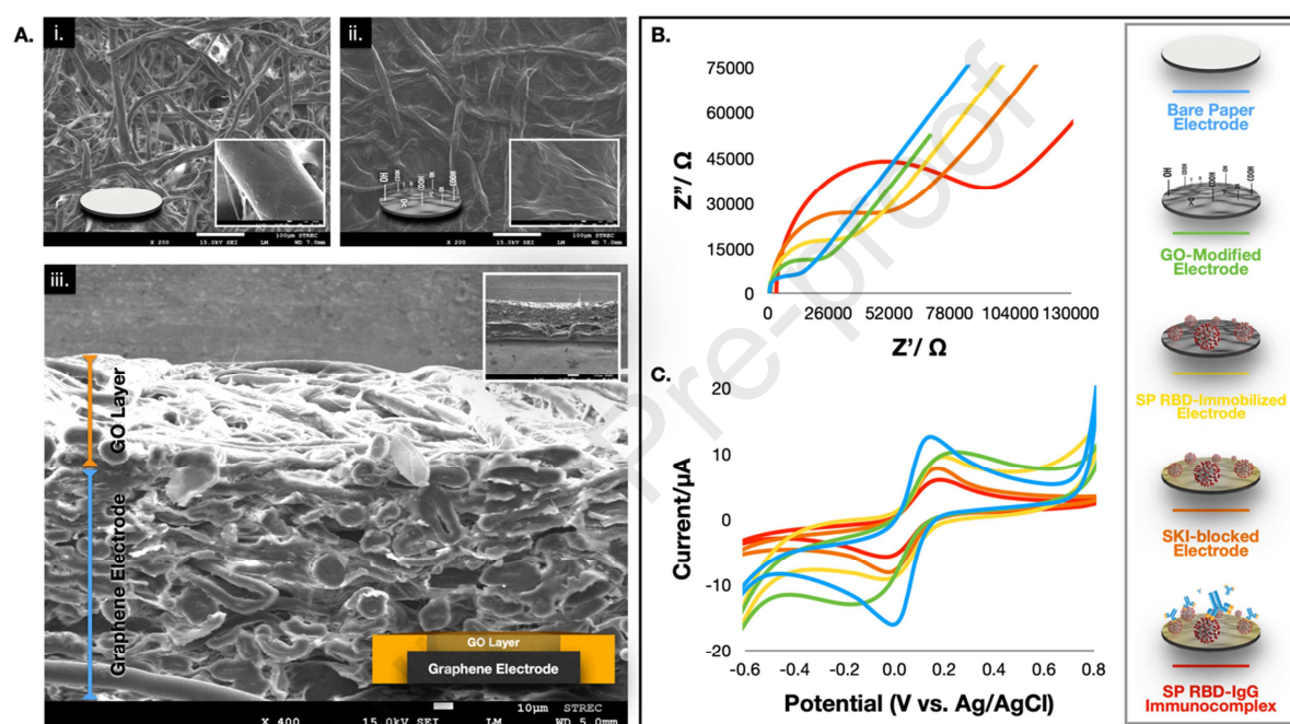
Figure 2. (A) SEM images of the bare paper (i), the GO modified paper (ii), and its corresponding cross-sectional image (iii). Characterization results of each fabrication step using the EIS (B) and CV (C) techniques. Note that all EIS Nyquist plots were fitted with the Randles equivalent circuit.
