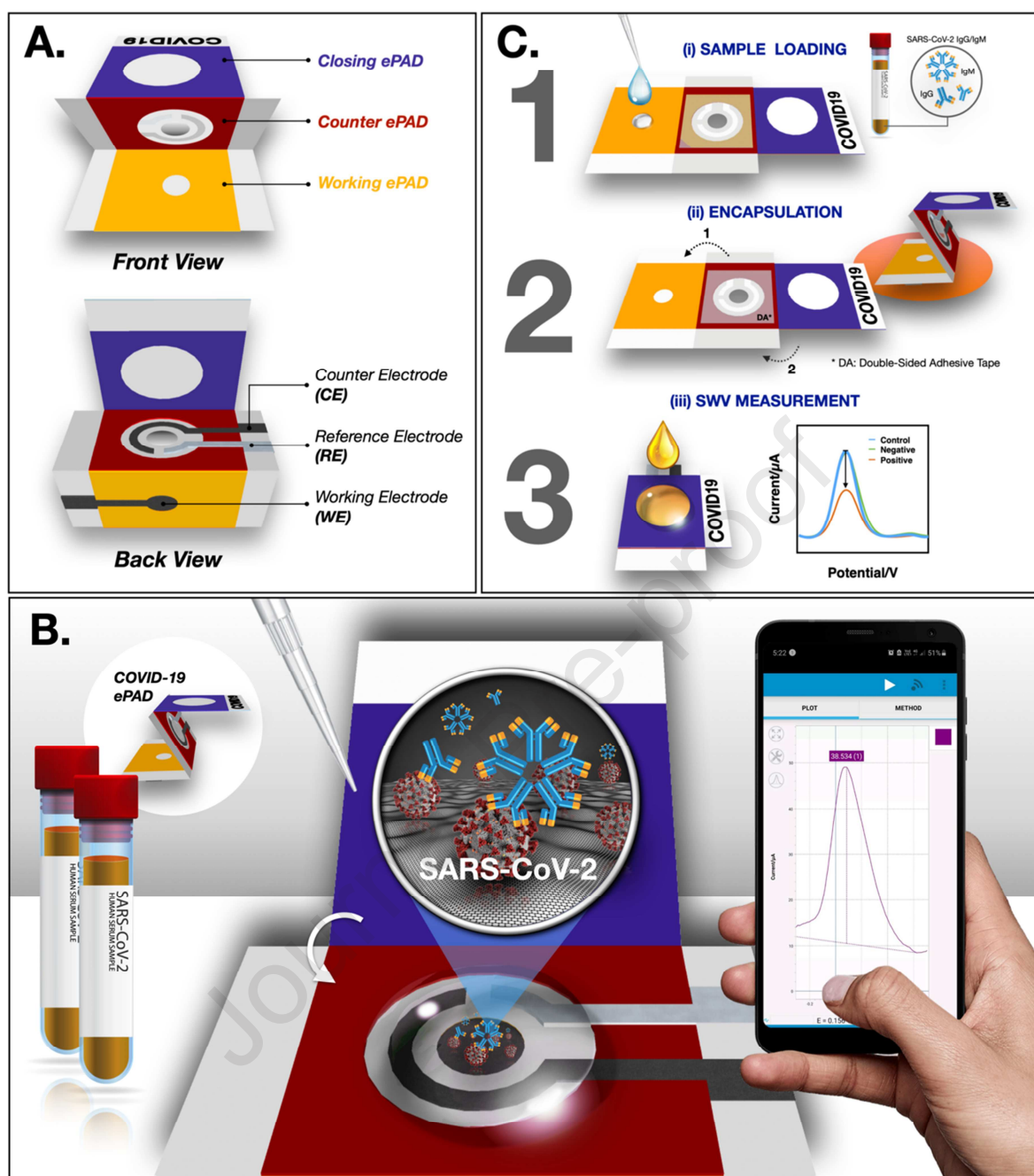
Figure 1. Schematic illustration of the (A) device components, (B) detection principle and (C) detection procedure of the COVID-19 ePAD.
