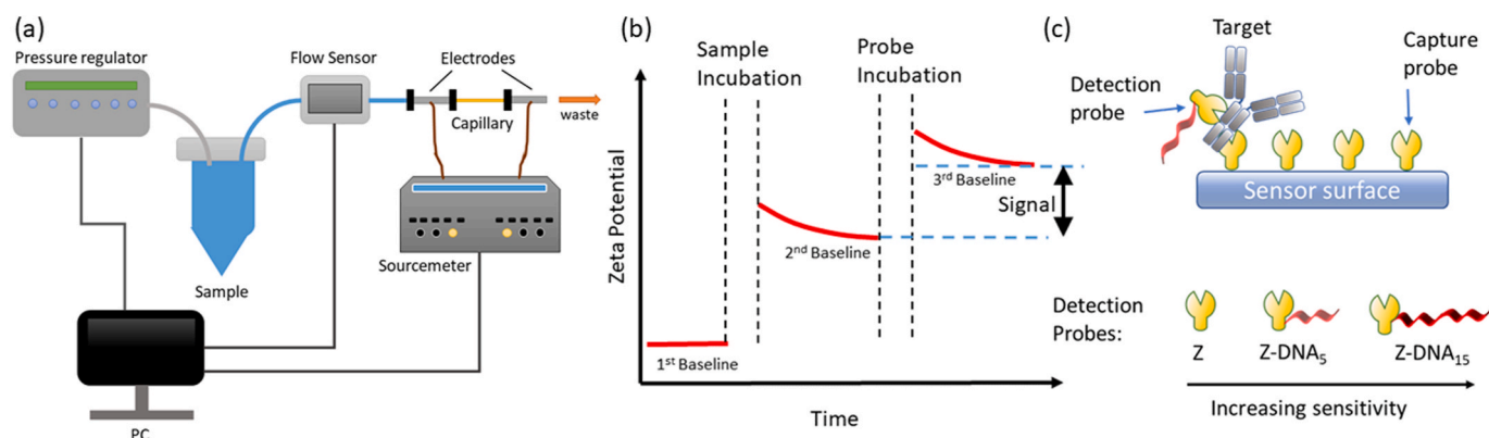
Fig. 1. Schematic representation of (a) the experimental setup and (b) the sequence of a multistep measurement for the sandwich assay, starting with the recording of the 1 st baseline, followed by the injection of the target until an equilibrium is reached. Thereafter, the 2 nd baseline is recorded for a fixed duration. After the injection of the detection probe, the recording of the 3 rd baseline follows. The signal of the sandwich assay is the difference indicated by the double-arrow. Panel (c) shows (top) a schematic of a sandwich assay, depicting the target, along with the capture and detection probes (not drawn to scale) and (bottom) the detection probe and its charge modification with the conjugation of DNA oligonucleotide of different lengths.
