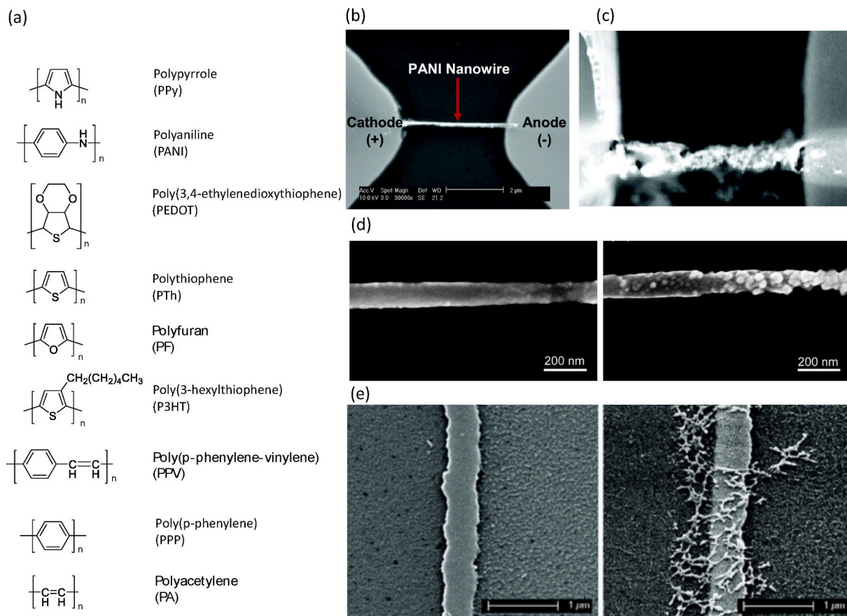
Fig. 4. Molecular structures of common CPNWs and some of their SEM images. (a) Molecular structure of common conducting polymers. (b) SEM image of a 100 nm wide by 4 μm long PANI nanowire. Scale bar: 2 μm. Reprinted with permission from (Ramanathan et al., 2004). Copyright (2004) American Chemical Society. (c) SEM image of a single avidin-conjugated ZnSe/CdSe quantum dots-embedded PPy nanowire (200 nm wide). Reprinted with permission from (Ramanathan et al., 2005). Copyright (2005) American Chemical Society. (d) SEM images of single PANI NW before (left) and after (right) functionalization with monoclonal antibodies. Adapted from (Lee et al., 2012). (e) SEM images of single PEDOT NWs (left) and net-like structure of virus-PEDOT composite (right). Reprinted with permission from (Arter et al., 2012). Copyright (2012) American Chemical Society.
