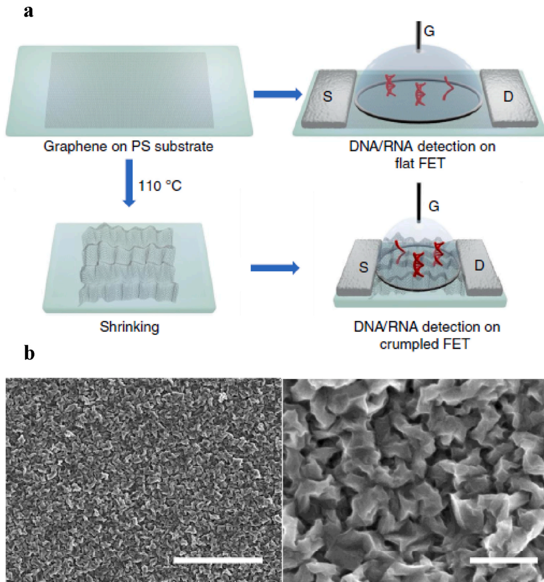
Fig. 9. FET biosensors of flat and crumpled graphene. (a) A schematic of the flat and crumpled graphene on polystyrene (PS) for detection of DNA/RNA. (b) SEM images of flat (left) and crumpled (right) graphene. The scale bar is 5 μm (left) and 500 nm (right). Adapted from (Hwang et al., 2020).
