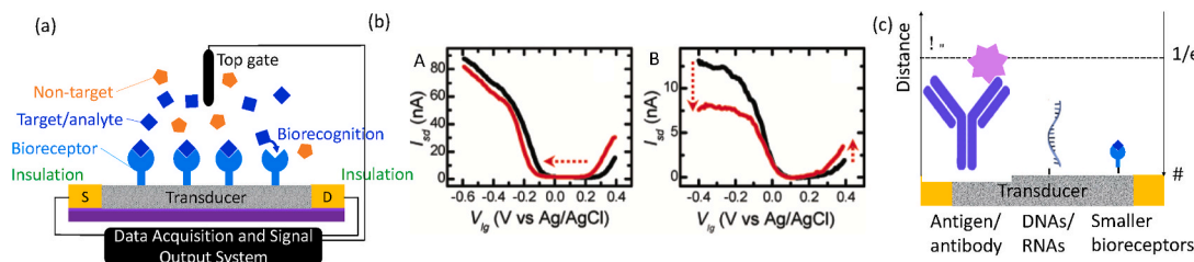
Fig. 2. Schematic diagrams of the FET biosensors structure, functionalization strategies and mechanism (not to scale). (a) A schematic illustration of the top-gated FET biosensor structure. (b) Modulation of SWCNT-FET transfer curve due to (A) electrostatic gating and (B) Schottky barrier effect. Reprinted with permission from (Heller et al., 2008). Copyright (2008) American Chemical Society. (c) A conceptual diagram for the Debye Length ( \lambda_D ) and relative size comparison of different bioreceptors and the relative point of observation of biorecognition events.
