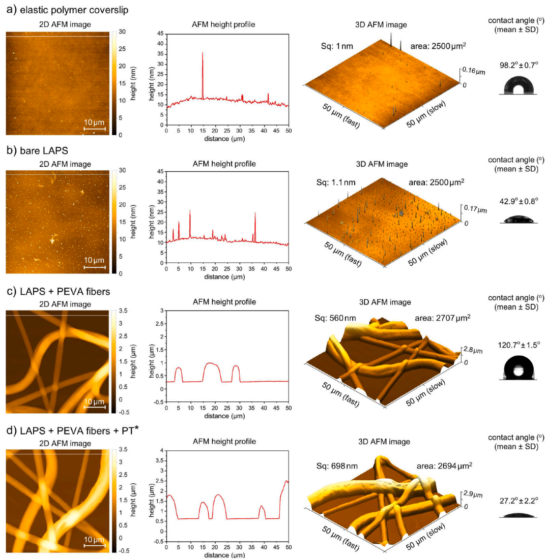
Fig. 2. Surface characteristics such as surface topography and wettability for various surfaces, a) elastic polymer coverslip, b) bare LAPS, c) LAPS modified with PEVA fibers and d) LAPS modified with PEVA fibers and then treated with O_2 plasma. The representative images and a profile graph for each surface are shown under different AFM analysis (2D height image, corresponding height profile and 3D height image) to indicate the surface topography. The representative photos of water droplets for each surface, which were obtained by sessile drop contact angle measurements of deionized (DI) water, indicate the wettability of the surfaces. The mean values of their contact angles, which were obtained from the measurement of the multiple samples, are also presented above each column. Notes: *PT indicates O_2 plasma treatment for 30 s. The AFM height profile for each surface is obtained from the area depicted in the corresponding 2D AFM image, along the trace indicated in white. Sq: Root mean square (RMS) roughness; area: Surface area.
