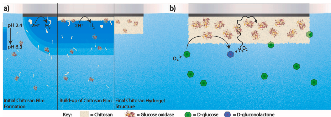
Fig. 1. a) The formation of the GOx-chitosan hydrogel on the surface of a platinum electrode through the electrodeposition of chitosan in the presence of GOx. b) The reaction that occurs on the surface of the GOx-chitosan platinum electrode to alter the surface potential. Glucose is oxidized to gluconolactone in the presence of \text{O}_2 , forming \text{H}_2\text{O}_2 as a byproduct. The \text{H}_2\text{O}_2 in the hydrogel then alters the measured open circuit potential.
