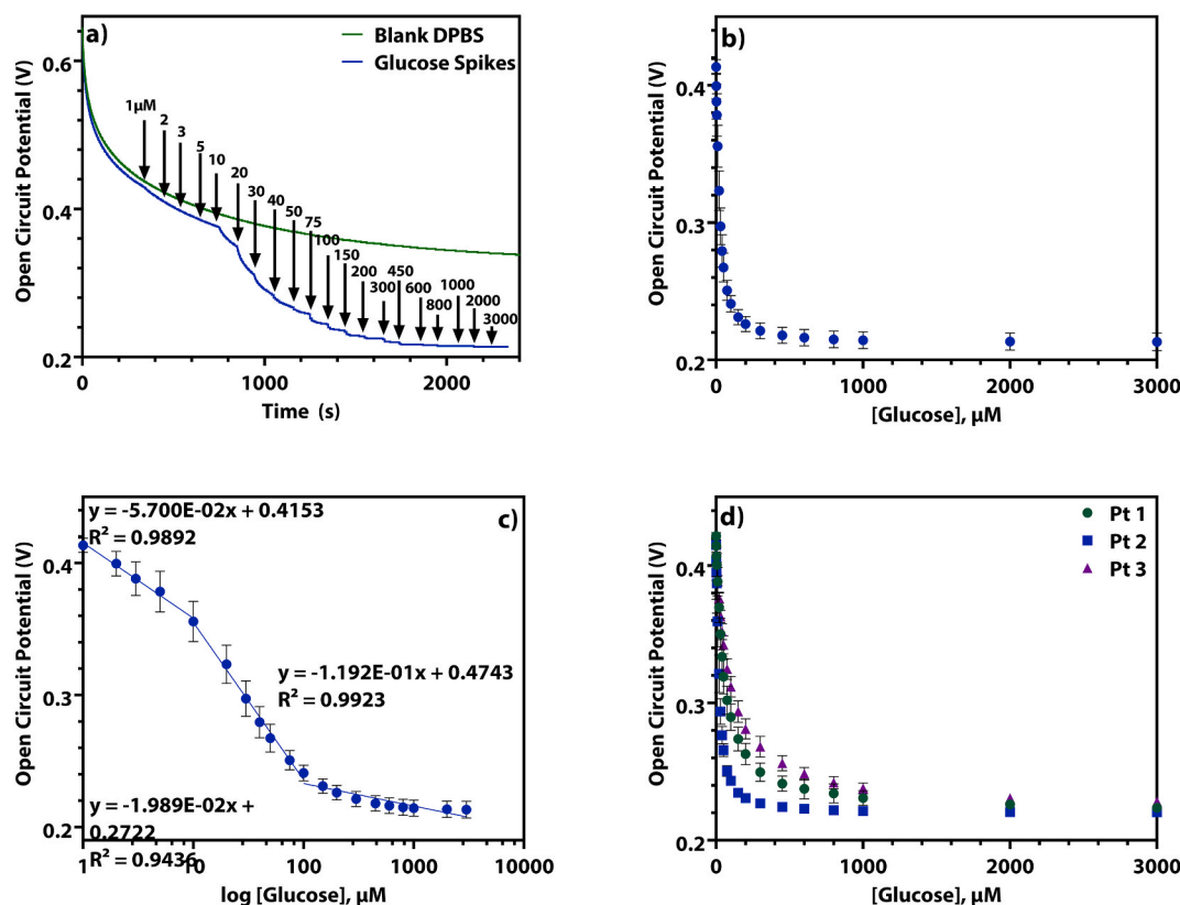
Fig. 2. a) The open circuit potential of a GOx-chitosan platinum macroelectrode in (green) a blank solution of DPBS and (blue) as 1 \mu\text{M} to 3 mM glucose is spiked into a solution of DPBS. b) The open circuit potential of a GOx-chitosan platinum macroelectrode as 1 \mu\text{M} to 3 mM glucose is spiked into a solution of DPBS over 28 days ( n = 21 , RSD = 4.50%). c) The semi-log plot of the open circuit potential of a GOx-chitosan platinum macroelectrode as 1 \mu\text{M} to 3 mM glucose is spiked into a solution of DPBS over 28 days ( n = 21 , RSD = 4.50%). d) The open circuit potential of 3 GOx-chitosan platinum macroelectrodes as 1 \mu\text{M} to 3 mM glucose is spiked into a solution of DPBS ( n = 3 , each). (For interpretation of the references to colour in this figure legend, the reader is referred to the Web version of this article.)
