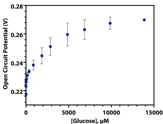
Fig. 4. The open circuit potential of a GOx-chitosan platinum microelectrode as 1 \mu\text{M} to 14 \text{ mM} glucose is spiked into a solution of DPBS ( n = 3 , RSD = 3.10%).
