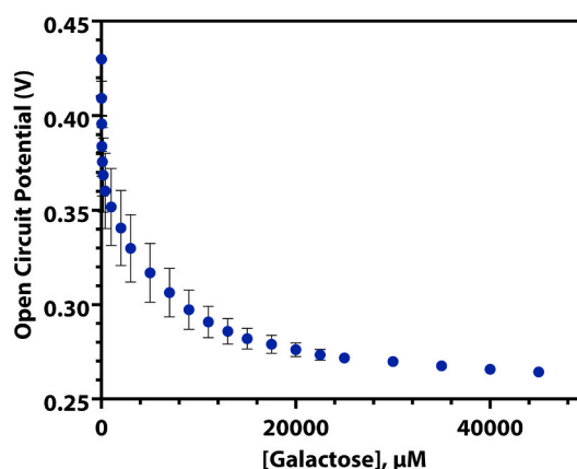
Fig. 5. The open circuit potential of a galactose oxidase-chitosan platinum macroelectrode as 10 \mu\text{M} to 50 \text{ mM} galactose is spiked into a solution of DPBS ( n = 3 , RSD = 5.84%).
