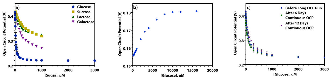
Fig. 3. a) The open circuit potential of a GOx-chitosan platinum macroelectrode as 1 \mu M to 3 mM different sugars are spiked into a solution of DPBS (n = 3). b) The open circuit potential of a GOx-chitosan platinum macroelectrode as 200 \mu M to 18 mM glucose is spiked into a solution of DPBS containing 1.3 mM acetaminophen and 170 \mu M ascorbic acid. c) The experimental open circuit potential (n = 3) of a GOx-chitosan platinum macroelectrode when 1 \mu M to 3 mM glucose is spiked into a solution of DPBS (blue) before being used in a continuous measurement, (green) after being used in a continuous measurement for 6 days, and (purple) after being used in a continuous measurement for 12 days. (For interpretation of the references to colour in this figure legend, the reader is referred to the Web version of this article.)
