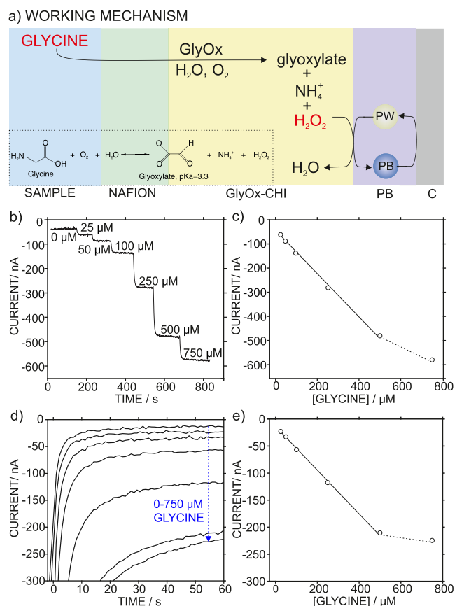
Fig. 1. a) Working mechanism underlying the response of the glycine biosensor. Amperometric response of the biosensor at increasing concentrations of glycine in artificial serum using b) the batch method, with c) the corresponding calibration graph and d) the drop method, with e) the corresponding calibration graph.
