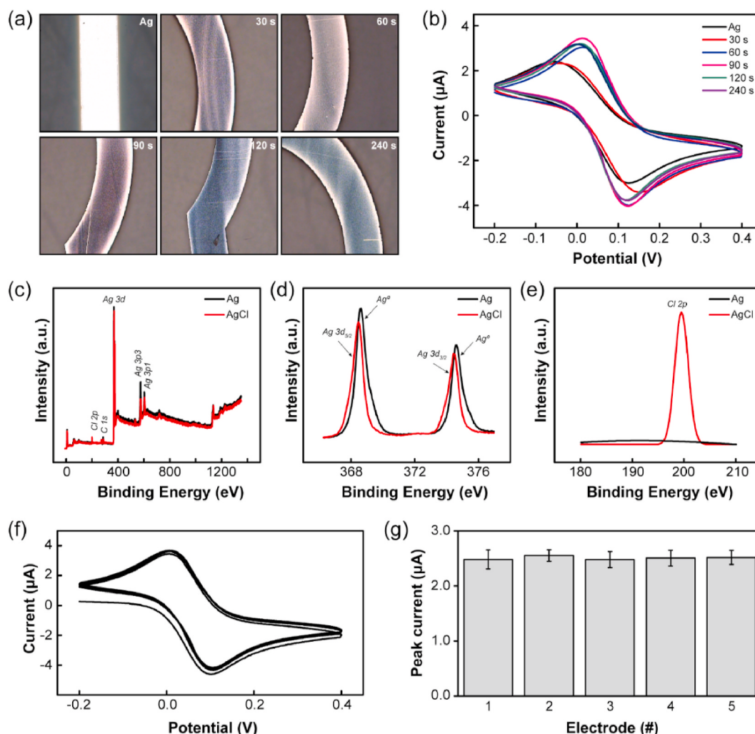
Fig. 2. Characterization of the Ag/AgCl electrode. (a–b) Optical images (a) and cyclic voltammograms (b) obtained from an Ag electrode after AgCl formation by immersing in a bleach solution for 30 s intervals. (c–e) X-ray photoelectron spectroscopy (XPS) spectra of Ag and AgCl electrodes: (c) survey spectrum, (d) Ag 3d 5/2 and Ag 3d 3/2 and (e) Cl 2p regions. (f–g) stability (f) and reproducibility (g) of the electrochemical biosensors by CV measurements.
