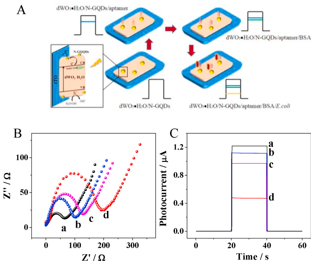
Fig. 2. (A) The fabrication process of the PEC aptasensor for detection of E.coli O157:H7. (B) EIS and (C) PEC characterization of the PEC aptasensor during the fabrication process. Here, curve a is for original ITO electrode modified with \text{dWO}_3\cdot\text{H}_2\text{O}/\text{N-GQDs} nanocomposite; curve b is after aptamer conjugation on ITO electrodes modified with nanocomposite; curve c is after BSA blocking on aptamer-conjugated ITO electrodes modified with nanocomposite; curve d is for E.coli O157:H7 capturing on aptamer-conjugated ITO electrodes modified with nanocomposite after BSA blocking.
