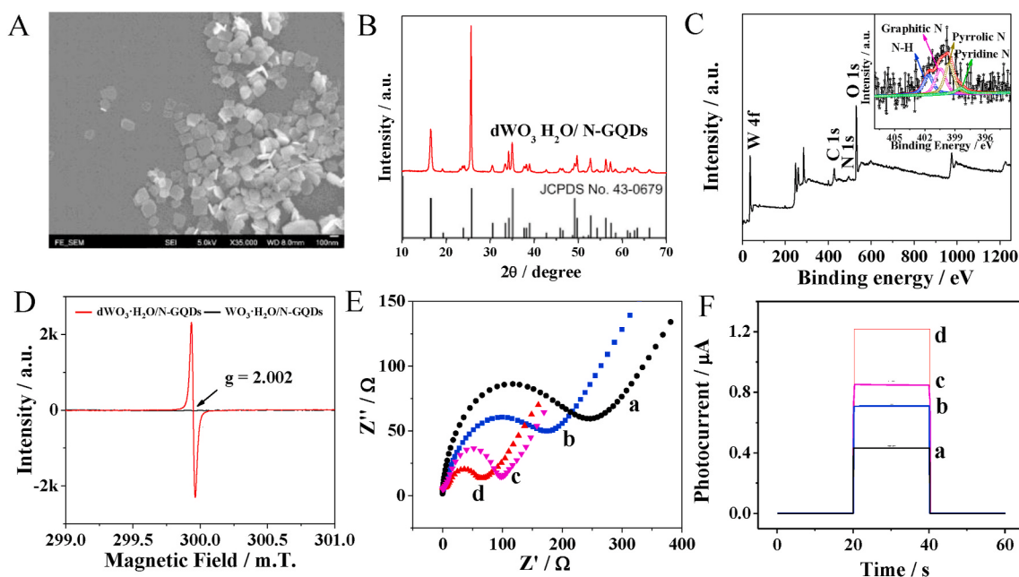
Fig. 1. (A) SEM image of \text{dWO}_3\bullet\text{H}_2\text{O}/\text{N-GQDs} nanocomposite. (B) XRD patterns of JCPDS no. 43-0679 and \text{dWO}_3\bullet\text{H}_2\text{O}/\text{N-GQDs} nanocomposite. (C) XPS survey spectra of \text{dWO}_3\bullet\text{H}_2\text{O}/\text{N-GQDs} nanocomposite. Inset: high resolution XPS spectra of the \text{N}_{1s} region of the nanocomposites. (D) ESR survey spectra of nanocomposite \text{WO}_3\bullet\text{H}_2\text{O}/\text{N-GQDs} with and without oxygen vacancies. (E) EIS Nyquist plots and (F) photocurrents of ITO electrodes coated with \text{WO}_3\bullet\text{H}_2\text{O} (curve a), \text{dWO}_3\bullet\text{H}_2\text{O} (curve b), \text{WO}_3\bullet\text{H}_2\text{O}/\text{N-GQDs} (curve c), and \text{dWO}_3\bullet\text{H}_2\text{O}/\text{N-GQDs} (curve d).
