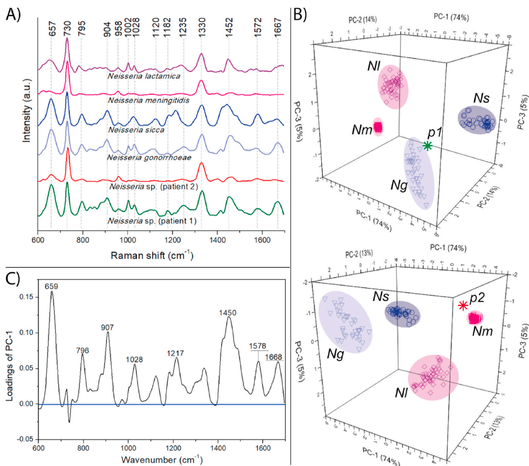
Fig. 3. The SERS spectra (A), 3D-PCA (B), and loadings plot (C) performed for two Neisseria strains detected in urethra swabs of two male patients: Patient 1 (p1) and Patient 2 (p2), and for type strains of N. gonorrhoeae (Ng), N. meningitidis (Nm), N. lactamica (Nl), and N. sicca (Ns).
