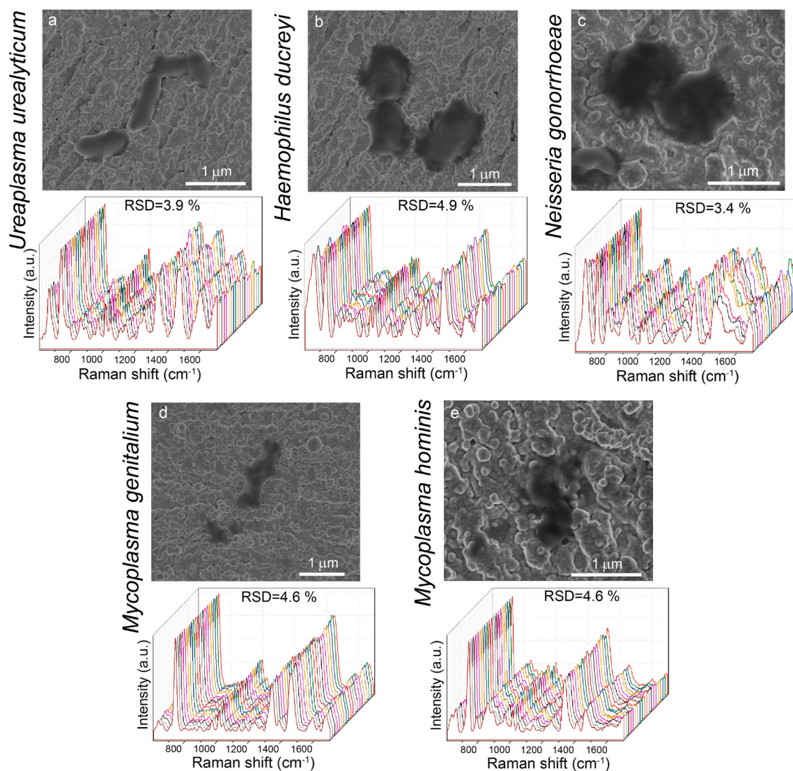
Fig. 1. The SEM images and SERS spectra with calculated RSD (relative standard deviation) for five investigated pathogens: U. urealyticum , H. ducreyi , N. gonorrhoeae , M. genitalium , and M. hominis placed onto the Si/Ag SERS platforms.
