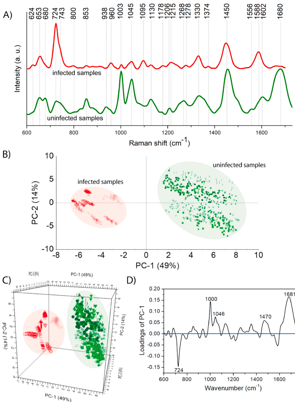
Fig. 4. The averaged SERS spectra (A), 2D-PCA (B), 3D-PCA (C), and loading plot (D) calculated for 20 different samples of male urethra swabs: 10 from control group (signed as 'uninfected samples' and marked with green) and 10 from experimental group (signed as 'infected samples' and marked with red). (For interpretation of the references to colour in this figure legend, the reader is referred to the Web version of this article.)
