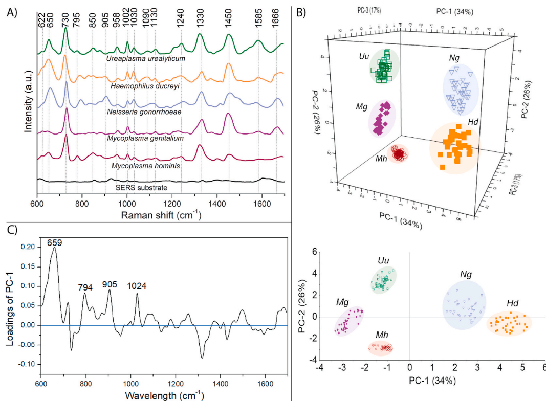
Fig. 2. The SERS spectra (A), PCA (B), and loadings plot of PC-1 (C) obtained for five investigated, sexually transmitted pathogens: U. urealyticum ( Uu ), H. ducreyi ( Hd ), N. gonorrhoeae ( Ng ), M. genitalium ( Mg ), and M. hominis ( Mh ).
