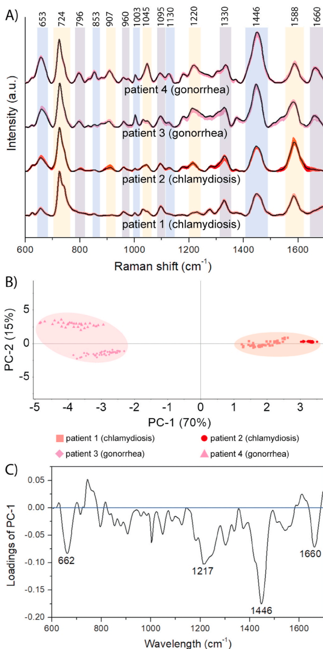
Fig. 5. The SERS spectra (A), 2D-PCA (B), and loading plot (C) obtained for four infected male urethra swabs collected from patients diagnosed with chlamydia and gonorrhea. For each specimen at least 30 single spectra were superimposed along with the averaged spectrum (black).
