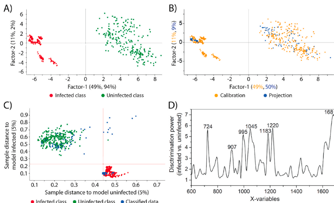
Fig. 6. The results of PLS1-DA analysis in the form of: (A) scores plot (LV1 vs LV2) for eight infected and eight uninfected samples of men's urethra swabs and (B) projection of tests samples (blue dots) onto the prepared PLS1-DA calibration model (orange dots). The results of SIMCA analysis in the form of: (C) Coomans' plot for infected and uninfected samples and (D) sample discrimination power on X-variables between infected and uninfected classes. For each analyzed sample about 30 spectra were used to create the calibration model. The green and the red clusters refer to all infected and uninfected samples, respectively (training set), while the blue points to the samples of the test set. (For interpretation of the references to colour in this figure legend, the reader is referred to the Web version of this article.)
