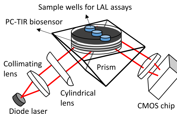
Fig. 1. Schematic drawing of the experimental setup for LAL assays using a PC-TIR biosensor.
