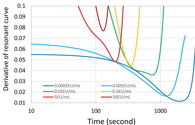
Fig. 4. Time derivatives of the resonant line shifts. The time corresponding to the minimum of each curve determines the onset time of the coagulation process of the LAL reaction to endotoxins, which increases with lowering the endotoxin concentration.
