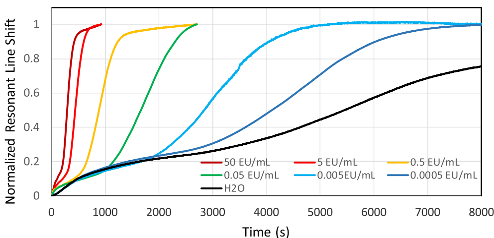
Fig. 3. Representative curves of the time dependence of the resonant line shifts of a PC-TIR sensor for samples with different concentrations of endotoxins; 50, 5, 0.5, 0.05, 0.005 and 0.0005 EU/mL. Different onset times can be observed for different endotoxin concentrations. Even the most diluted endotoxin solution used (0.0005 EU/mL) can be easily distinguished from the negative control.
