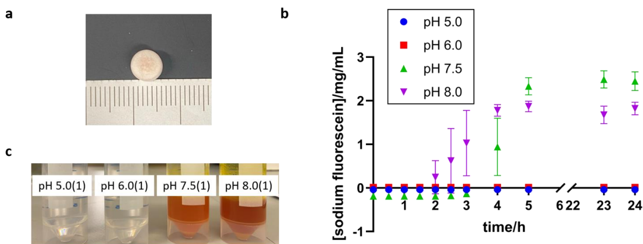
Figure 1. Functionality testing of the tablet-based lozenge. (a) A coated tablet-based lozenge, scale in mm. (b) Concentration of SF released from lozenge in buffers of varying pH (5.0, 6.0, 7.5 & 8.0), sodium fluorescein quantified using calibration curves ( Supplementary Fig.1 ). (c) The lozenge was placed in the falcon tubes, visual analysis of SF released from the lozenge release buffers of varying pH (5.0, 6.0, 7.5 & 8.0). Plots were prepared using GraphPad Prism version 9. Mean from four independent experiments are shown with error bars representing the standard deviation.
