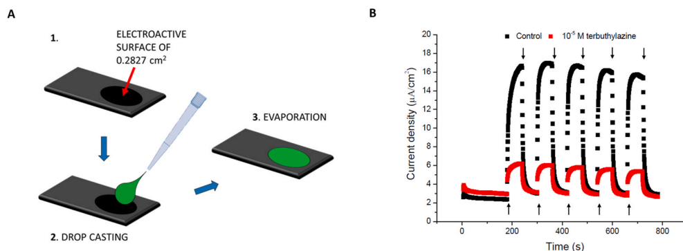
Fig. 1. Setup and electrochemical characterization of the biosensor. (A) Schematic representation of the procedure adopted for the fabrication of the bio-electrode. (B) Typical chronoamperometric response curve recorded with the thylakoids (chlorophyll concentration 1000 μg/mL, 20 μL)-functionalized carbon paper electrode in the absence (black curve, control) or presence of 10 -5 M terbuthylazine (red curve) in the measuring buffer. Upwards arrows indicate light on and downwards arrows light off. (For interpretation of the references to colour in this figure legend, the reader is referred to the Web version of this article.)
