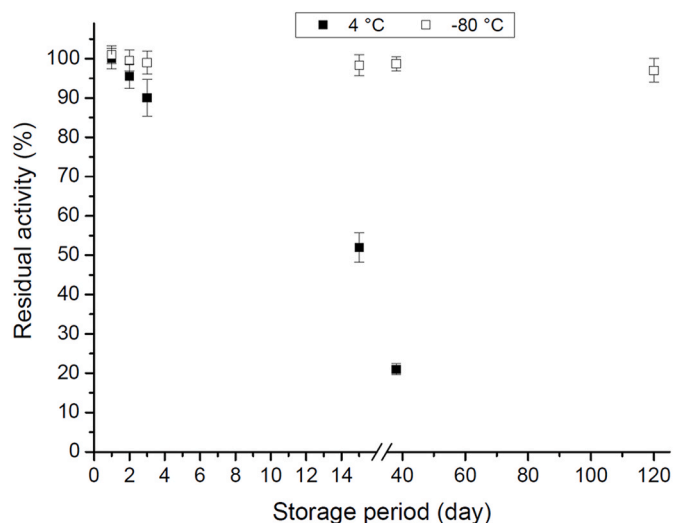
Fig. 2. Stability of the biosensor stored in the dark at 4 °C and -80 °C. The residual activity (%) of the biosensor was calculated as the ratio of the photocurrent density obtained in each condition and the photocurrent density of the biosensor stored for 1 day at 4 °C. Points and bars are means and standard deviations of three replicates.
