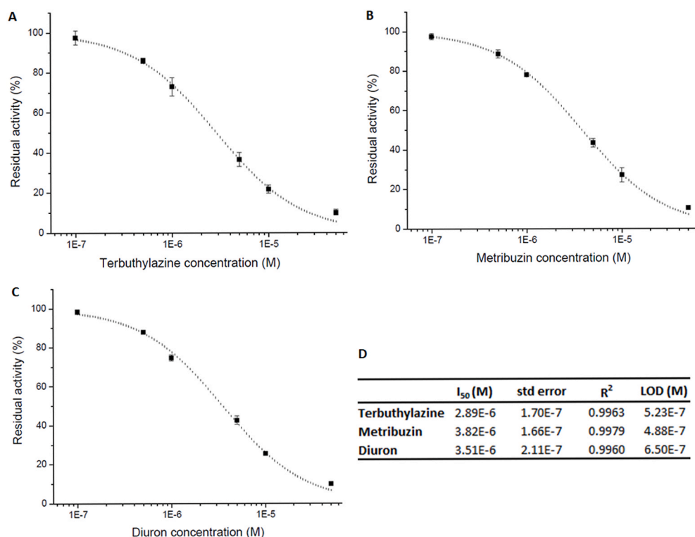
Fig. 3. Concentration-response curves for the herbicides terbutylazine, metribuzin and diuron. The residual activity (%) of the biosensor was calculated as the ratio of the photocurrent density obtained in the presence and in the absence of terbutylazine (A), metribuzin (B) and diuron (C). Points and bars are means and standard deviations of three replicates. The experimental points were fitted using the Langmuir adsorption isotherm (fit curves in dotted line) according to (Koblížek et al., 2002) and the I_{50} dose and LOD values were derived together with the R^2 and standard errors (D) (for I_{50} and LOD determination and statistical analysis see details in the Supporting Information).
