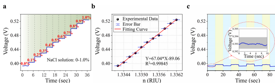
Fig. 3. Results of RI sensing. a Signal of different NaCl solution concentrations; b Fitting curve of the response to different concentrations of NaCl solution corresponding to a . The error bar is the standard deviation of the voltage corresponding to each concentration; c Signal of pure water and 0.003% NaCl solution. The data in the blue background corresponds to pure water, and the data in the green background corresponds to 0.003% NaCl. Inset: the voltage fluctuation of the biosensor corresponding to pure water. (For interpretation of the references to color in this figure legend, the
