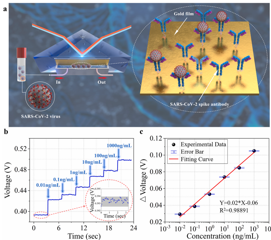
Fig. 5. Detection of the SARS-CoV-2 spike antigen. a Schematic illustration of the sensing unit; b Signal of different concentrations of SARS-CoV-2 spike antigen. Inset: the voltage fluctuation of the biosensor corresponding to the blank sample; c Response voltage changes as a function of solution concentrations and the fitting curve. The error bar is the standard deviation of the voltage change corresponding to each concentration.
