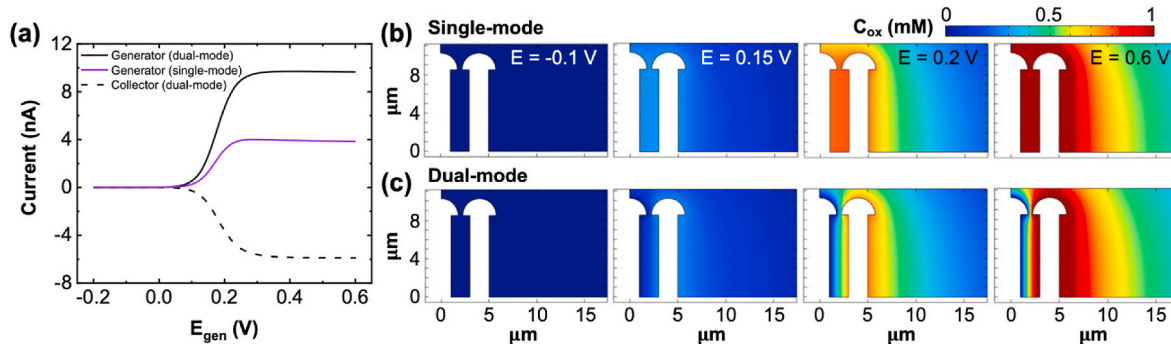
Fig. 2. a) A representative voltammogram of the ring-disk microelectrode configuration in single- and dual-mode (1 mM [\text{Fe}(\text{CN})_6]^{4-} , 1 mM KCl, scan rate = 50 \text{ mV s}^{-1} , E_{coll} = -0.15 \text{ V} or floating). The resulting concentration profiles of [\text{Fe}(\text{CN})_6]^{3-} are shown for b) single-mode, and c) dual-mode over the course of the voltammetric scan. Note that the formal potential of the redox probe is around 0.17 \text{ V} .
