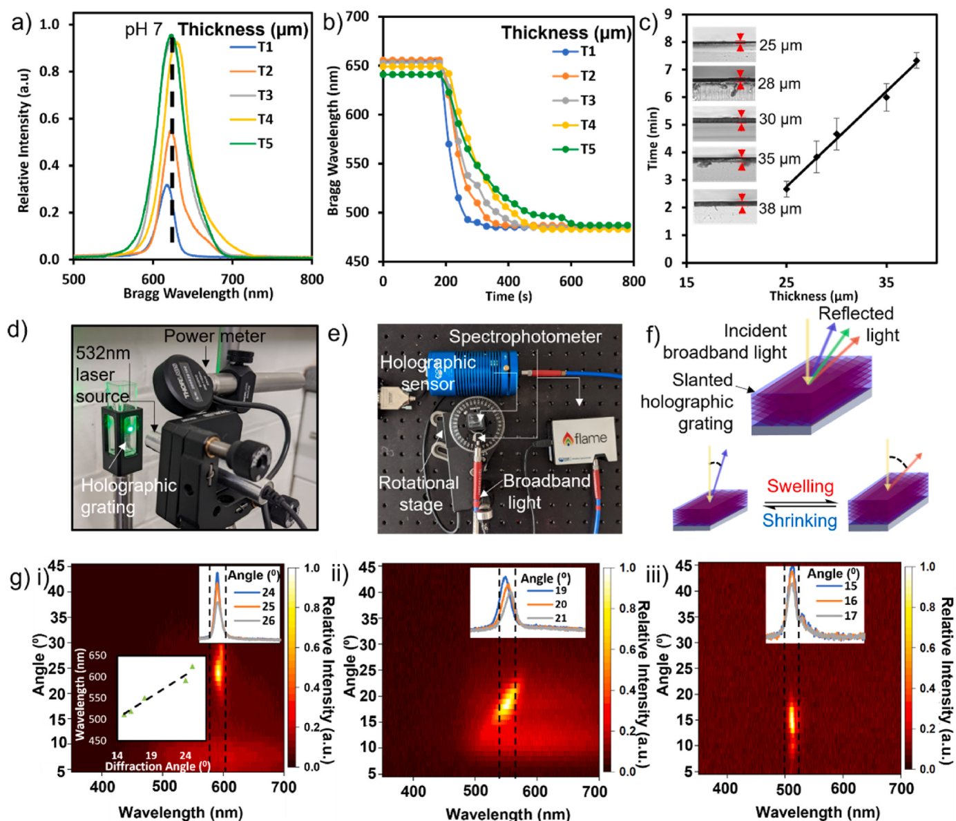
Fig. 4. Thickness and angular replay dependency of the holographic sensor; a) Bragg replay wavelength as a function of thickness in tris-buffer solution (pH 7, 50 mmol \text{L}^{-1} , KCl). b) Rate of movement for the sensors with differing thickness. c) A graph to demonstrate the relationship between hydrogel thickness and response time, microscope images of holographic hydrogels with thicknesses 25 \mu\text{m} , 28 \mu\text{m} , 30 \mu\text{m} , 35 \mu\text{m} , and 38 \mu\text{m} , where error bars represent the calculated standard error of 3 independent sets of results. d) Diffraction efficiency measurement set up with 532 nm laser and power meter. e) Optical set up utilised to record the angle of highest intensity reflection. f) Relationship of diffraction angle to reflection wavelength recorded from holographic sensors. g) Angular measurements from rotational stage for holographic sensors with replay wavelengths of i) 592 nm, ii) 550 nm, and iii) 520 nm, inset highlights the diffraction at angles of greatest intensity.
