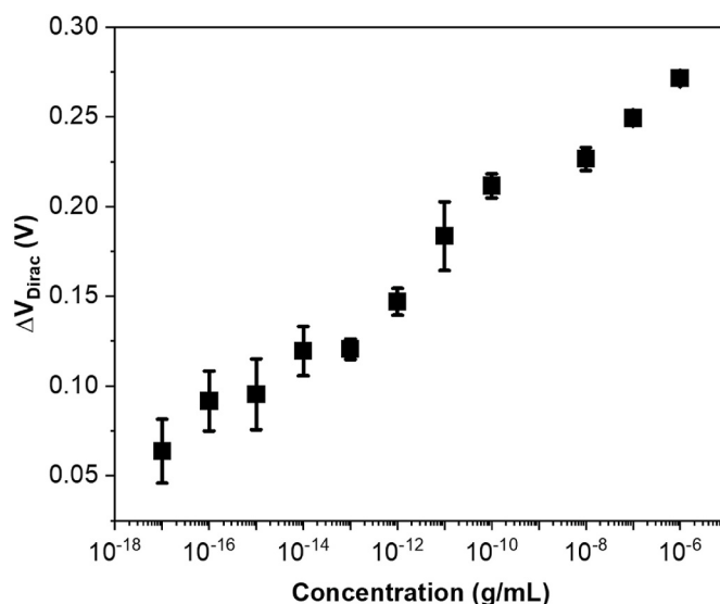
Fig. 6. The shift in the Dirac voltage in response to increasing concentrations of the N-proteins in the solution demonstrates a detection range stretching over 11 orders of magnitude.
