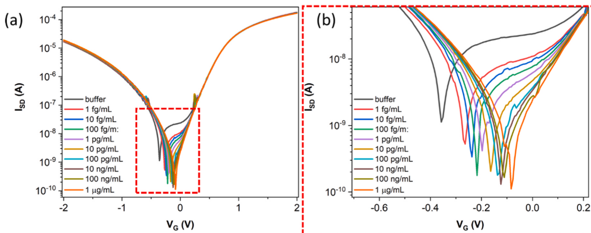
Fig. 4. SARS-CoV-2 N-protein biosensing performance of the antibody-functionalized BN-GO gel FET. (a) The shift in the Dirac voltage in response to increasing concentrations of the N-protein solutions. (b) The magnification of the Dirac points in (a).
