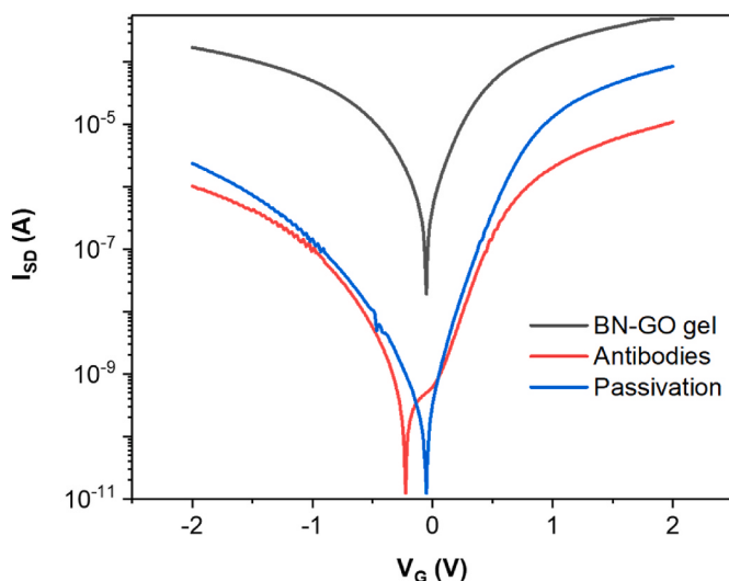
Fig. 3. The change in drain current vs gate voltage plot for a constant drain bias of the BN-GO gel FET after the antibody immobilization and after the passivation with ethanolamine.
