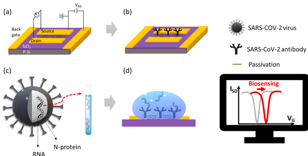
Fig. 1. The schematics of the device configuration and biosensing mechanism of the BN-GO gel FET SARS-CoV-2 N-protein biosensor. (a) The back-gated FET device configuration with the BN-GO gel channel located between the source and drain electrodes. (b) The device configuration after the SARS-CoV-2 antibody functionalization and the passivation with ethanolamine. (c) The N-protein of the SARS-CoV-2 virus is diluted in a buffer solution. (d) The biosensing response is determined based on the shift in the Dirac voltage after the addition of the N-protein-containing solution.
