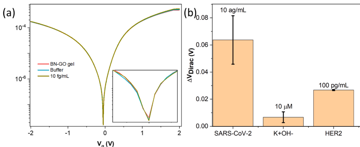
Fig. 5. (a) Specificity and (b) selectivity results for the BN-GO gel FET biosensor. The inset in (a) is a 40x enlargement of the Dirac points.
