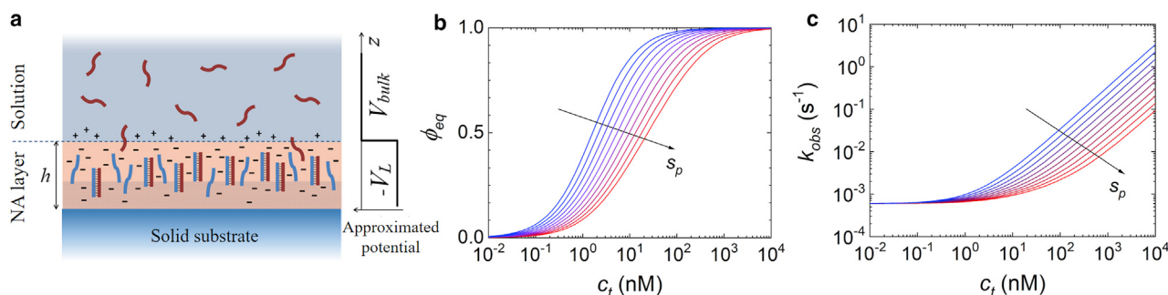
FIGURE 5 Schematic representation and numerical solution of the NLER model. (a) The surface region is rich in NA probes (blue) immobilized on the copolymer coating (shaded area) and hence provides a negative net charge, which further increases upon hybridization with the target strands (dark red). The electrostatic potential is approximated by a step function having a value lower than that of the bulk solution up to a distance h from the RPI solid surface. (b) Fraction of hybridized probes at equilibrium and (c) kinetic rate computed for different surface densities of probes, from 10^{10} \text{ mm}^{-2} (blue) to 10^{11} \text{ mm}^{-2} (red). The curves were computed with fixed kinetic parameters k_{on}^0 = 2.3 \times 10^{-4} \text{ nM}^{-1} \text{ s}^{-1} and k_{off} = 7.2 \times 10^{-4} \text{ s}^{-1} and for \Gamma = \gamma s_p , with \gamma = 2 \times 10^{-11} \text{ mm}^2 . To see this figure in color, go online.
