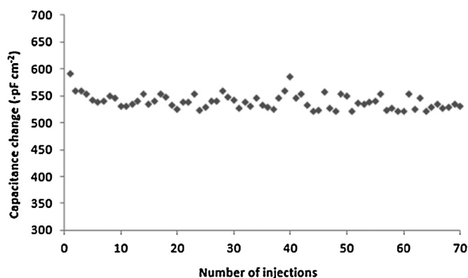
Fig. 7. Reproducibility of the microcontact-BSA imprinted capacitive biosensor (BSA concentration: 1.0 \times 10^{-10} M; flow rate: 100 \mu L/min; sample volume: 250 \mu L; running buffer: 10 mM phosphate, pH: 7.4; regeneration buffer: 25 mM glycine-HCl, pH: 2.5).
