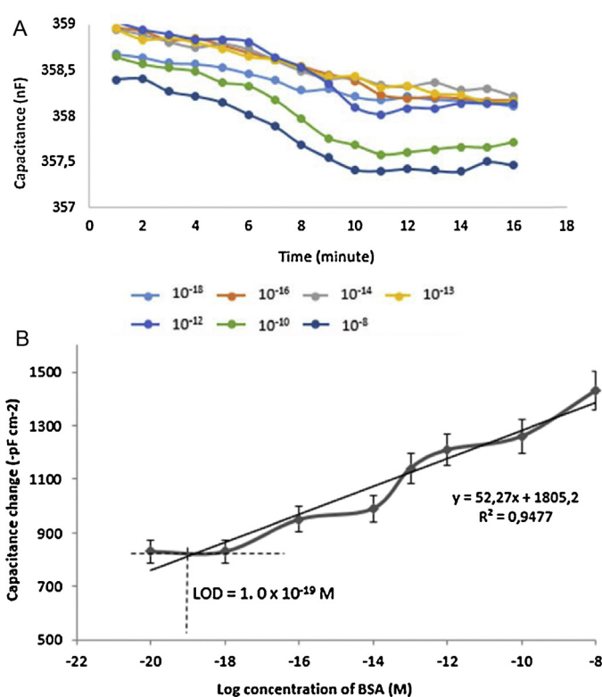
Fig. 5. (A) Capacitance of the BSA imprinted electrode vs. BSA concentrations (M) under optimum conditions (Flow rate: 100 \mu L/min; sample volume: 250 \mu L; running buffer: 10 mM phosphate, pH: 7.4; regeneration buffer: 25 mM glycine-HCl, pH: 2.5; T: 25 °C). At t = 0 the target BSA analyte was injected to the flow cell containing the gold transducer containing the micro contact imprinting surface. Prior to each injection, the surface was regenerated using 25 mM glycine-HCl, pH 2.5 (not shown in this graph). (B) Capacitance change vs. logarithm of BSA concentrations for the microcontact-BSA imprinted electrode under optimum conditions (Flow rate: 100 \mu L/min; sample volume: 250 \mu L; running buffer: 10 mM phosphate, pH: 7.4; regeneration buffer: 25 mM glycine-HCl, pH: 2.5; T: 25 °C).
