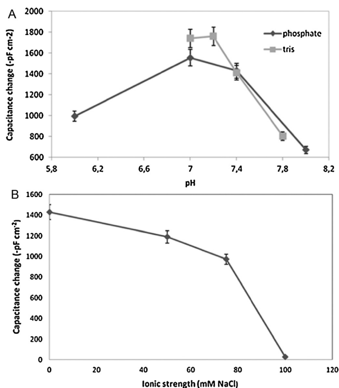
Fig. 4. (A) Effect of type and pH of the running buffer on BSA detection (BSA concentration: 1.0 \times 10^{-10} M; flow rate: 100 \mu L/min; sample volume: 250 \mu L; regeneration buffer: 25 mM glycine-HCl, pH: 2.5; T: 25 °C). (B) Effect of ionic strength of the running buffer on BSA detection (BSA concentration: 1.0 \times 10^{-10} M; flow rate: 100 \mu L/min; sample volume: 250 \mu L; running buffer: 10 mM phosphate, pH: 7.4; regeneration buffer: 25 mM glycine-HCl, pH: 2.5; T: 25 °C).
