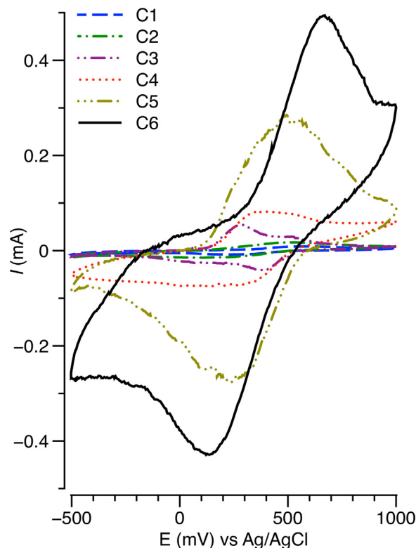
Fig. 6. Voltammograms of the PAni/ι-CGN biocomposites (C1 – 0.05 M, C2 – 0.1 M, C3 – 0.15 M, C4 – 0.2 M, C5 – 0.25 M, and C6 – 0.5 M).
