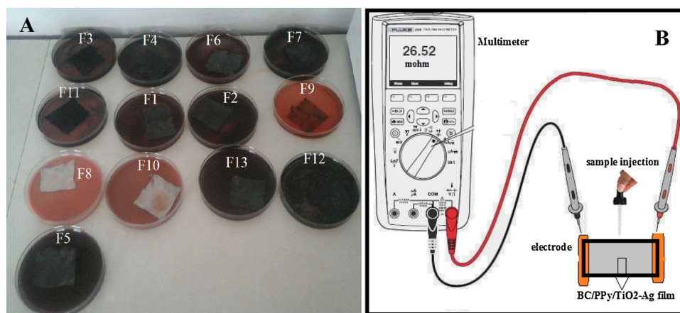
Fig. 1. Different BC, BC/TiO 2 -Ag, BC/PPy and BC/Py/TiO 2 -Ag films (A) and bacteria sample injection system to the sensors (B).
