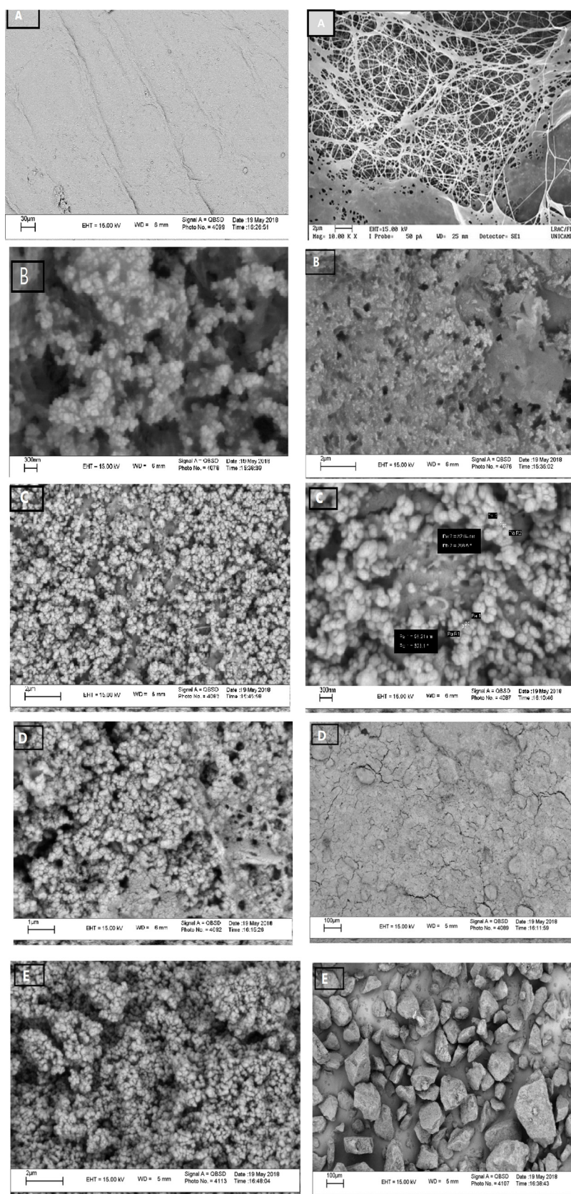
Fig. 2. SEM images of pure BC (A), BC/PPy (B), BC/TiO 2 -Ag (C), BC/PPy-TiO 2 -Ag (D) films and TiO 2 -Ag powder (E).
