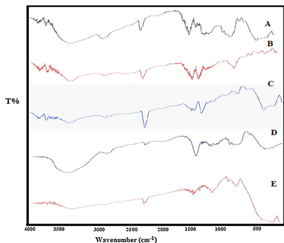
Fig. 3. FT-IR spectra of BC/TiO 2 -Ag (A), BC/PPy (B), BC/PPy/TiO 2 -Ag (C), pure BC (D), and pure TiO 2 -Ag (E).
