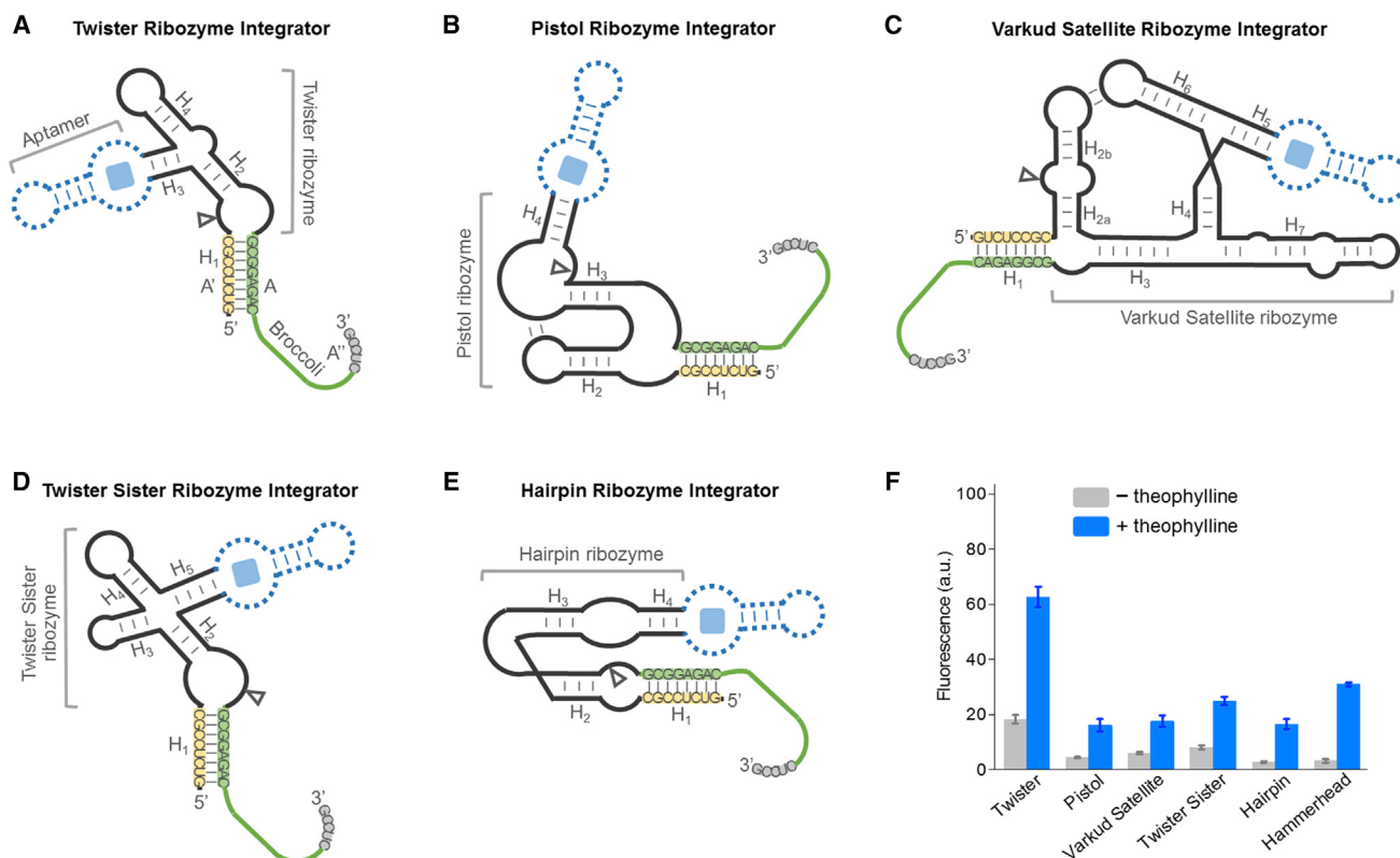
Figure 3. Generation of RNA Integrators with Diverse Natural cis -Acting Ribozymes
