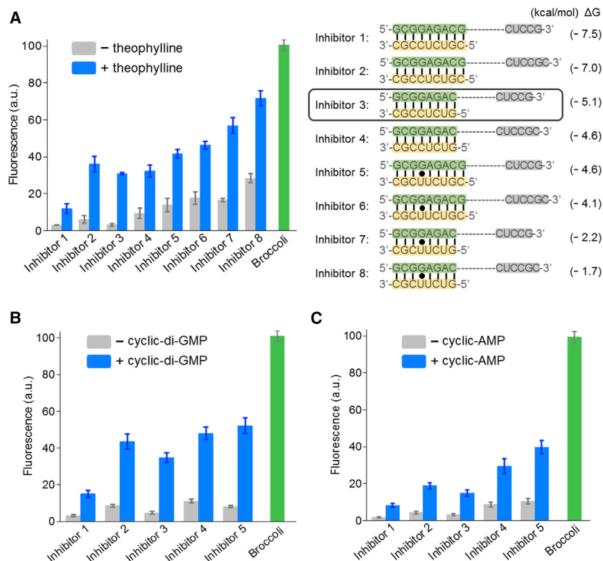
Figure 2. Optimization of the RNA Integrator Performance
