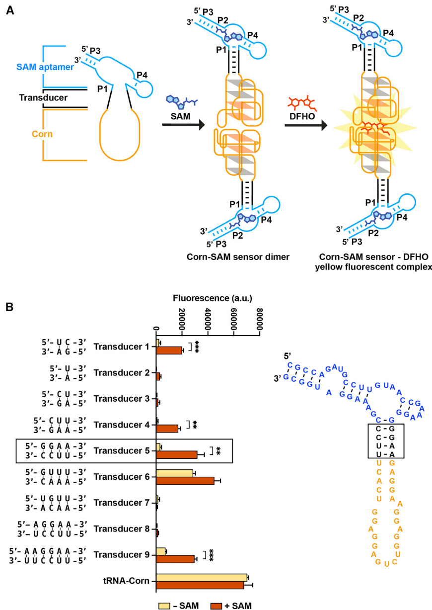
Figure 2. Design of a Corn-SAM Sensor
