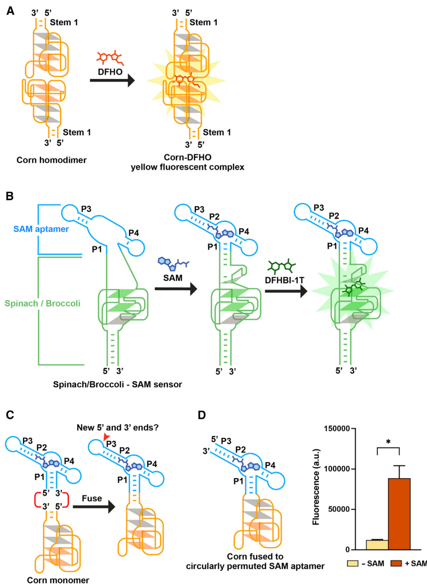
Figure 1. Strategy for Designing Metabolite Sensors Using Corn
