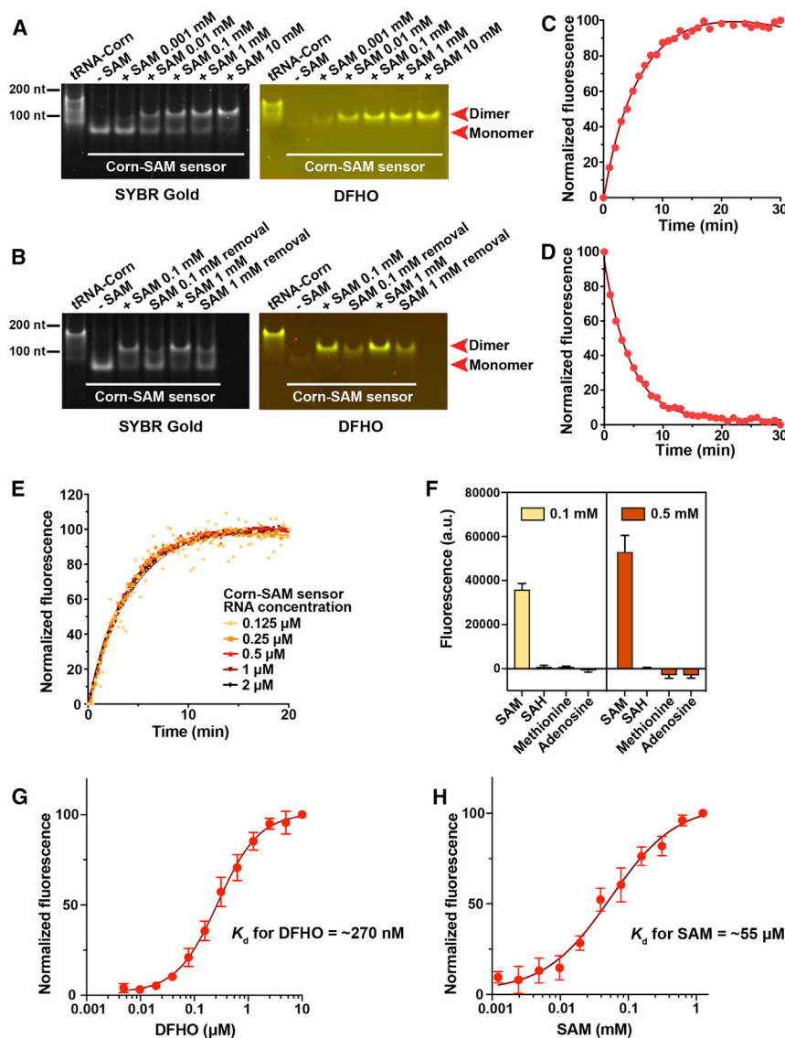
Figure 3. SAM Induces the Dimerization of the Corn-SAM Sensor
