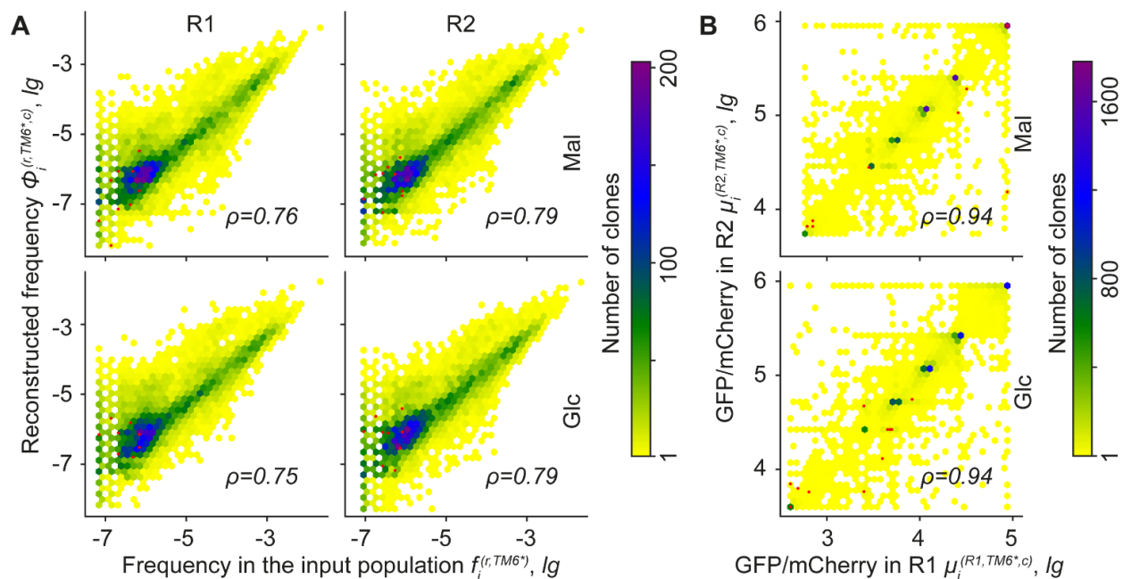
Figure S7. A robust assignment of GFP/mCherry ratio to each clone in C45-HHRz library is based on its relative frequency in sorted cell populations. A. Correlation between the absolute frequency of a clone in the C45-HHRz library input population before sorting f_i (x-axis) and its reconstructed frequency after sorting \Phi_i (y-axis), which results from summing up its relative frequencies calculated for each sorted cell population. See Notes S2-S3 and Table S2 for details. The correlation is estimated with the Spearman's coefficient \rho . The presented data correspond to the clones that are supported by more than 2 reads in each of the four sorted TM6* populations (2 replicates \times 2 carbon sources) and that are found in two input TM6* populations (2 replicates), therefore, 12,348 clones in R1 and 12,413 in R2. B. Correlation between GFP/mCherry ratios assigned to each clone \mu_i in two independent sorting experiments (R1, R2) of C45-HHRz library in TM6* background cultured either on maltose or glucose. The presented data correspond to 15,031 clones that are supported by 4 reads or more in each of the four sorted TM6 populations (2 replicates \times 2 carbon sources). In correlation plots in A and B , the x-y space has been binned into discrete hexagons, and the color of a hexagon denotes the number of clones lying within. A calibrated color-scale reference is indicated on the right of each panel. The red points indicate the 11 hits identified by the high-throughput screening. Note that 9 out of 11 hits were identified in input populations, and that on the top plot in B some red points overlap.
