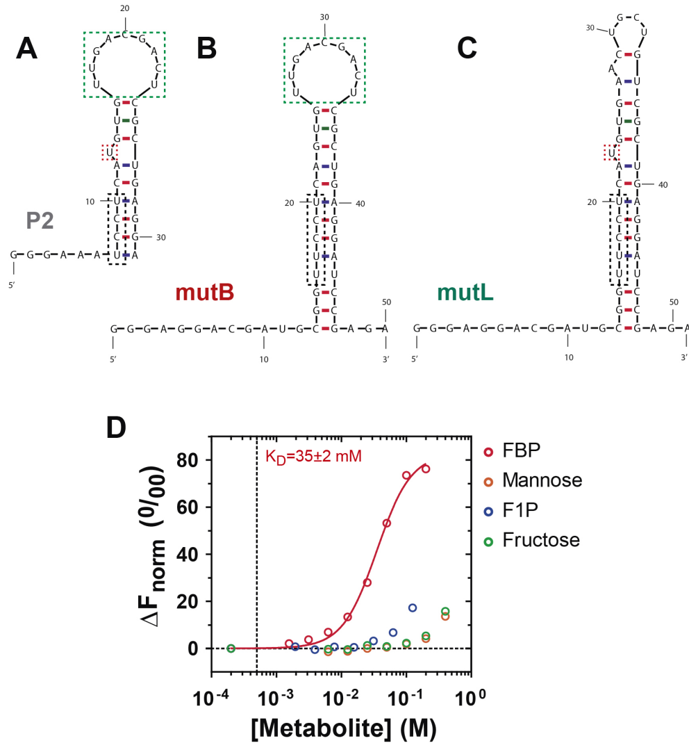
Figure S2. Secondary structure models of C45 mutants used in binding analyses. Deletion of U23 bulge in C45 does not alter the aptamer's selectivity. A. A utant targeting the base of the conserved stem of C45 with the 5' (G1 to G12) and 3' (A49 to A51) tails as well as the base of the conserved stem (C13 to U16 and U45 to G48) deleted. B-C. Mutants targeting the regions that underwent changes in SHAPE reactivity upon FBP binding: the U-bulge ( B , mutB : U23 was deleted) and C45 loop ( C , mutL : nucleotides U27 to U34 of the loop were substituted by the complementary sequence). RNA secondary structure models were retrieved using the energy minimization algorithm Mfold (M. Zuker, 2003, Nucleic Acids Res. 31 (13), 3406-15). Red and blue lines indicate Watson and Crick base pairs; green lines indicate Wobble or Hoogsteen base pairs. D. MST analysis of binding of mutB to monosaccharides (fructose, mannose) and phosphorylated metabolites (F1P, fructose-1-phosphate; FBP, fructose-1,6-bisphosphate). Apparent dissociation constant ( K_D ) was estimated using a non-linear regression model assuming one binding-site and specific binding with Hill slope.
