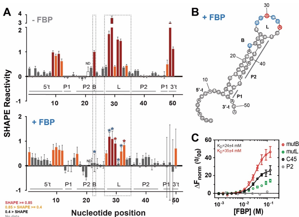
Figure 2. C45 aptamer adopts a stem-loop secondary structure and, upon FBP binding, changes its tertiary structure, involving the loop. A. 1-methyl-6-nitroisoatoic anhydride (1M6)-SHAPE reactivity profiles of C45 aptamer in the presence (+FBP, bottom panel) or absence (-FBP, top panel) of FBP (86 mM). Bars represent the average of SHAPE reactivities of each nucleotide from five independent experiments; error bars represent the standard error of the mean. Bar colors are used to categorize SHAPE reactivity in three levels: dark grey for low, orange for intermediate and red for high reactivity. SHAPE reactivity values ranges are indicated in the legend (bottom left). Asterisks indicate significant differences, where differences in reactivity were higher than 0.3 and p-values from two-sided student's t-test lower than 0.05; blue and red asterisks indicate a significant decrease or increase of SHAPE reactivity in the presence of FBP, respectively. Boxes with dotted lines delimit bulge (B) and loop (L) regions in C45 aptamer, where clustered differences in SHAPE reactivity occur. Different parts of the aptamer are indicated below the bars (5'-t and 3'-t: tails in 5' and 3' ends, respectively; P1, P2: stems 1 and 2; B: bulge; L: loop) B. Schematic representation of predicted C45 RNA secondary structure obtained with RNAstructure software, which considers energy minimization coupled to SHAPE reactivity. As in A, blue and red indicate nucleotides showing a significant decrease or increase of SHAPE reactivity in the presence of FBP C. Microscale thermophoresis (MST) analysis of FBP binding to mutants targeting the regions that altered SHAPE reactivity upon FBP binding: the U-bulge (mutB: U23 deletion) and C45 loop (mutL: U27 to U34 substitution by its complementary sequence). C45 and mutant P2 (deletion of the base of the conserved stem: G1-U16 and U45-A51) show the extremes of the affinity to FBP. Points represent the mean \pm S.D. of three independent experiments.
