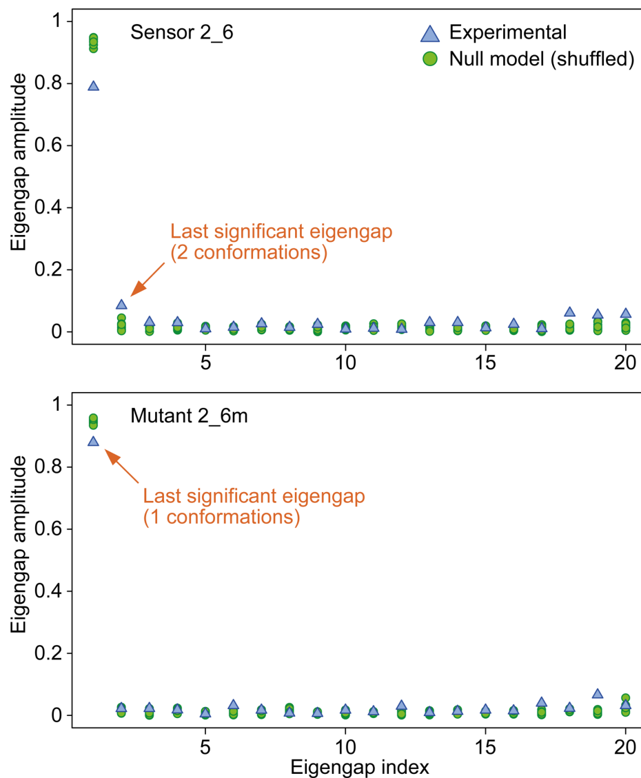
Figure S8. The sensor 2_6 has two conformations inside the cell whereas the mutant 2_6m folds in only one conformation. Eigengap plots of the differences in magnitude between consecutive eigenvalues. Spectral analysis has been performed using the set of reads covering positions 4-70 (relative to the C45-HHRz RNA device). Eigenvalues are taken from the normalized graph Laplacian matrix constructed using 20 reactive adenosine and cytosine residues.
