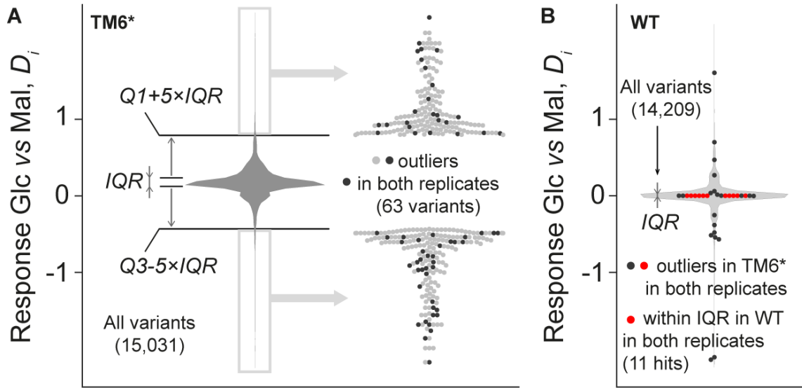
Figure 5. Hit selection in high-throughput in vivo screening of C45-HHRz variants that respond to differences of intracellular FBP. A. Identification of variants in C45-HHRz library expressed in the TM6^* strain that have different response while growing on glucose versus growing on maltose, associated with low and high intracellular FBP, respectively. To compare a variant's response to the change in intracellular FBP, we calculate the measure Response Glc vs Mal, D_i (y-axis; see Table S2 for details), a transformed measure of the change in the GFP/mCherry ratio ( \lg \mu_i^{Glu} / \mu_i^{Mal} ), and check if its value deviates from those of other variants. The distribution of this response D_i of all the variants is depicted in the violin plot. We select variants with the extreme response values that are located beyond the segment [Q1 - 5 \cdot IQR, Q3 + 5 \cdot IQR] (grey boxes on the left, grey and black dots on the right), where Q1 and Q3 are the lower and upper quartiles, and IQR is the interquartile range. To exclude variants that end up in the selection due to technical noise, we repeated the sorting experiment and looked for clones with consistently deviating response (63 clones, black dots on the right). All the clones in this analysis are covered by 4 sequencing reads or more in each of the four sorting experiments (2 carbon sources \times 2 independent experiments). B. Exclusion of variants showing an intracellular FBP-independent response. Wild-type (WT) cells display a similar FBP level when cultured in glucose or in maltose, and thus, hits should not show a response between these carbon sources in C45-HHRz library expressed in wild-type background. 11 variants are located within the IQR of the response in C45-HHRz library in the wild type in two independent sorting experiments, these variants are thus considered the hits from the screening. The presented distribution and its IQR used for selection is calculated from the data of variants supported by 4 sequencing reads or more in each of the four sorting experiments; the values corresponding to the dots were obtained using the data supported by at least 2 reads in each of the four sorting experiments. For simplicity of the representation, in both A and B , we present the data corresponding to one replicate experiment (R1). See Note S3 describing the hit selection in more detail.
