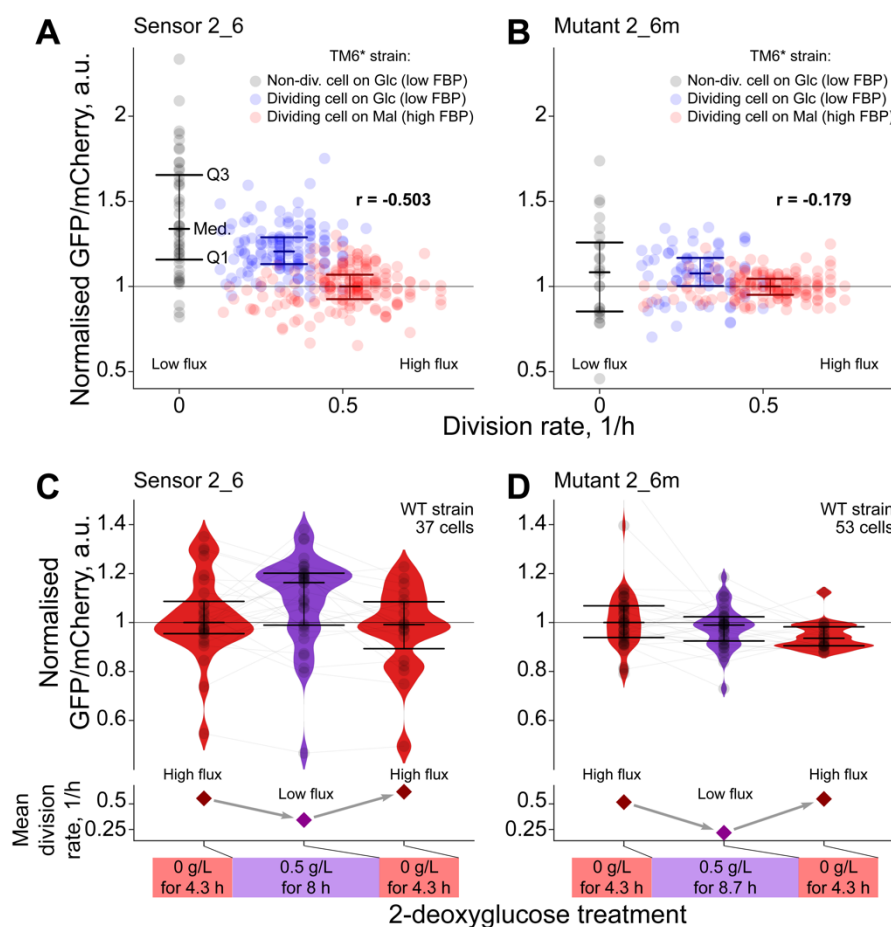
Figure 8. The FBP sensor functions as a glycolytic flux biosensor. A-B. The GFP/mCherry ratio of the sensor 2_6 (A) or its mutant 2_6m (B) in three categories of cells, namely, non-dividing TM6* cells consuming glucose (44 in 2_6 and 24 in 2_6m), dividing TM6* cells consuming glucose (138 in 2_6 and 77 in 2_6m) and dividing TM6* cells consuming maltose (183 in 2_6 and
