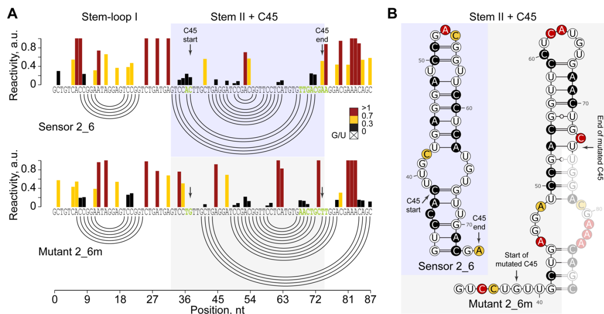
Figure 7. The intracellular-FBP sensor in vivo maintains the structural elements of the C45 aptamer that are critical for FBP binding in vitro . A. In vivo DMS-MaPseq analysis of the C45-HHRz RNA device in the sensor 2_6 and its mutant 2_6m. Bases differing between the two sequences are highlighted in green. Bars are color-coded according to base reactivity (low: black, medium: yellow, high: red; G and U do not show reactivities). Mutational data has been normalized by box-plot normalization. Reactivities were capped at 1 for representation purposes. Experimentally-constrained secondary structures are depicted as arc plots. B. Secondary structure models of Stem II merged with the C45 aptamer (Stem II + C45) in the sensor 2_6, and of the corresponding region in the mutant 2_6m. Bases are colored according to reactivities shown in A. The arrows demark the aptamer C45 (or its mutated version) within the C45-HHRz RNA device of 2_6 (or 2_6m), the sequences beyond the arrows belong to HHRz. C40U is a transition already observed in 2_6 at the level of high-throughput screening.
