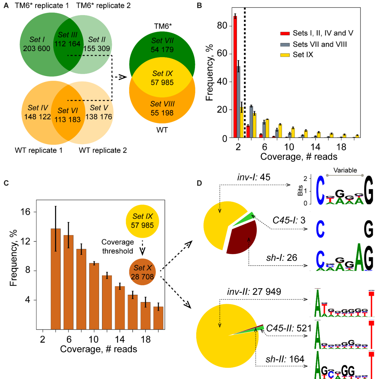
Figure S5. Molecular exploration of the diversity and composition of the pre-selected C45-HHRz RNA device library with a functional ribozyme moiety. A. Venn diagrams showing the distribution of unique sequences in different C45-HHRz library input samples used in this study. The total number of unique sequences found in each sample is distributed among different sets. The unique sequences found in two biological replicates of the same strain ( TM6* or wild type) correspond to sets III and VI. The unique sequences found in both strains (sets III and VI) correspond to the set IX. The set sizes are presented on the segments of the Venn diagrams. B. The distribution of coverage among the sequences in the sets (I, II, IV and V) found within individual biological replicates only, in the sets (VII and VIII) found in two replicates of the same strain only and in the set (IX) found in all the four populations. The bar length and the error whiskers shows the mean and two standard deviations of the frequency for a group of sequences (three groups are shown with different colors) in the four populations (samples). See Note S2 discussing
