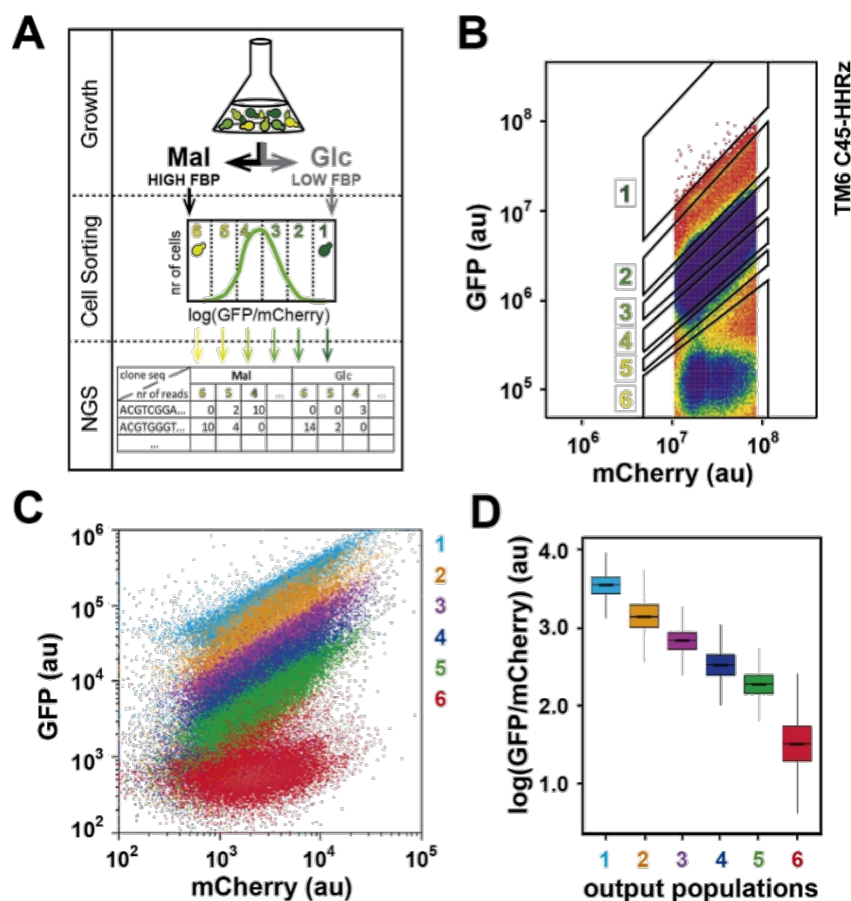
Figure 4. Sorting of C45-HHRz RNA device library yields six sub-populations with distinct GFP/mCherry ratios. A. Experimental pipeline of the high throughput in vivo screening of C45-HHRz RNA devices that respond to FBP. TM6* cells with the C45-HHRz library are grown in medium with either glucose or maltose (top panel). Cells are sorted into six sub-populations according to their GFP/mCherry ratios (middle panel). Sorted cells sub-populations are subjected to next-generation sequencing to identify the distribution of each clone throughout the population. B. Sorting of C45-HHRz RNA device library. A representative example of the gating of a FACS sorting experiment is shown (C45-HHRz library grown in glucose; 378,309 cells plotted). Cells with an intermediate 1-log-wide mCherry expression were gated. We used this gating because we found that the GFP signal was less robust in cells with low mCherry expression in clonal populations ( c.f. GFP-mCherry signal overlap among different HHRz versions for mCherry values between 5 \times 10^5 - 10^7 in Figure S6A), while in cells with intermediate mCherry levels dispersion of GFP values remained constant across the bins (Figure S6B). Sorting gates were established according to GFP/mCherry ratio, ranging from the signal of fully active (gate 6) to that of inactive ribozymes (gate 1). The width of the gates 2-5 was set according to the width of a cell population from a single clone in GFP/mCherry plot. C. Overlay of GFP-mCherry scatter plots obtained from regrown, sorted sub-populations. Sorted sub-populations were grown for several generations prior to analysis. 20,000 cells from each sub-population are plotted. D. Single-cell GFP/mCherry ratio distribution in sorted sub-populations from C45-HHRz library
