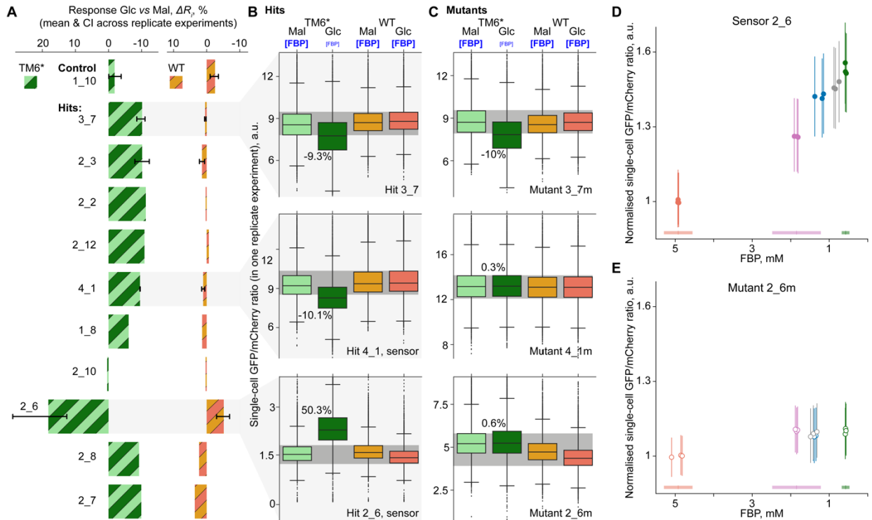
Figure 6. Validation of individual hits as FBP sensor candidates. A. Response of hits in cells cultivated in glucose as compared to cells cultivated in maltose ( Response\ Glc\ vs\ Mal, \Delta R_i ). Intracellular FBP concentration differs in TM6* strain and stays the same in the wild-type (WT) strain, when cells are grown on these two carbon sources (Glc, glucose; Mal, maltose). Response\ Glc\ vs\ Mal, \Delta R_i is calculated as the percentage of the change in the GFP/mCherry ratio between the cells cultivated in glucose and maltose as compared to the cells cultivated in maltose: \Delta R_i = \frac{1}{|G|} \cdot \sum_{t \in G} \frac{M(i, Glc, t) - M(i, Mal, t)}{M(i, Mal, t)} \cdot 100\% , where i is a hit, M(i, Glc, t) and M(i, Mal, t) are the median GFP/mCherry ratios in the population of cells grown on glucose and maltose, respectively; G is the set of three ( |G| ) time points t in the exponential part of a culture's growth curve. The bar and whisker lengths denote the mean value of \Delta R_i and its 95%-confidence interval calculated for the replicate cultivation experiments. No whiskers are shown in case of single cultivation experiment. The following numbers of data points were used to calculate the mean and the confidence interval in both TM6* and WT: 6 for 1_10 in both strains, 3 for 3_7, 2 for 2_3, 3 for 4_1 and 3 for 2_6. B-C. The single-cell distribution of the GFP/mCherry ratio in the four populations (2 strains \times 2 carbon sources) at one time point t in the growth curves of selected hits (B) and their mutants (C). The box shows the interquartile range IQR , the line in the center of it denotes the median M(i, Mal, t) or M(i, Glc, t) , the whiskers spread until Q1 - 1.5 \times IQR or Q3 + 1.5 \times IQR , where Q1 and Q3 are the lower and upper quartiles.
