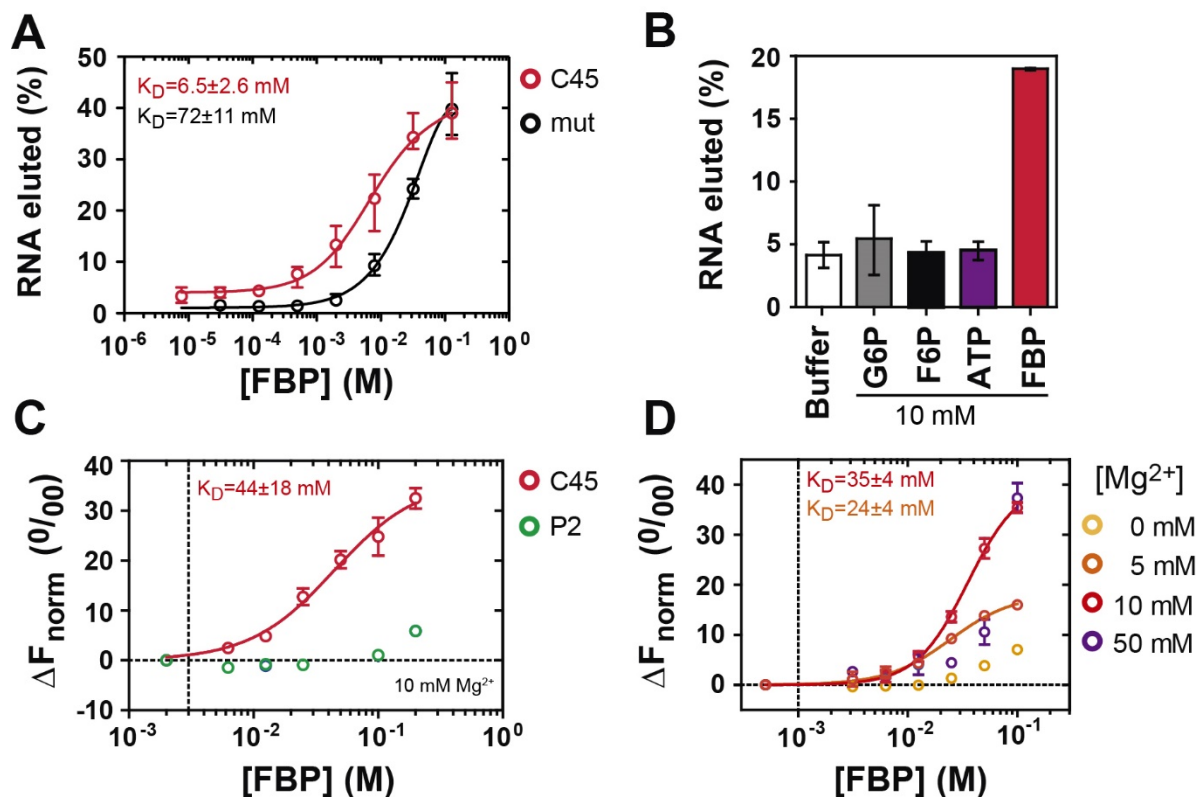
Figure 1. The aptamer C45 binds FBP under physiological conditions. A. Binding assays of an RNA clone (C45) retrieved by SELEX and a mutant variant (mut), in which the stem structure predicted to exist in most selected clones is disrupted (Figure S1). Fluorescently labeled (CAL Fluor Red 610) RNAs were incubated with FBP immobilized to sepharose, and eluted with different concentrations of free FBP. B. Assay done as in A, but where 10 mM solutions of glucose-6-phosphate (G6P), fructose-6-phosphate (F6P), adenosine-triphosphate (ATP), or fructose-1,6-bisphosphate (FBP) were used to release RNA from a sepharose column with immobilized FBP. Fluorescence released by the last washing step before elution (Buffer) is indicated. C. Microscale thermophoresis (MST) analysis of free FBP binding to Cy5-labeled C45 aptamer and a mutant lacking the 5' and 3'-end tails and the four pair of nucleotides that make up the base of the conserved stem (P2) (Figure S2). Binding assays were carried out in cytoplasmic buffer CB (See Methods) with 10 mM MgCl_2 . D. MST analysis of FBP-binding to C45 in solution under different MgCl_2 concentrations. Apparent dissociation constants ( K_D ) were estimated using a non-linear regression model assuming one binding-site and specific binding with Hill slope. In D, K_D values correspond to binding assays carried out with 10 and 5 mM MgCl_2 , respectively. In yeast, the intracellular free magnesium concentration is reported to be in the range from 0.1 to ~2 mM (Van Eunen et al., 2010; Zhang et al., 1997). Results in A-D represent the mean and the interquartile range from three replicates. Dashed lines in C-D indicate 0 in x and y axes.
