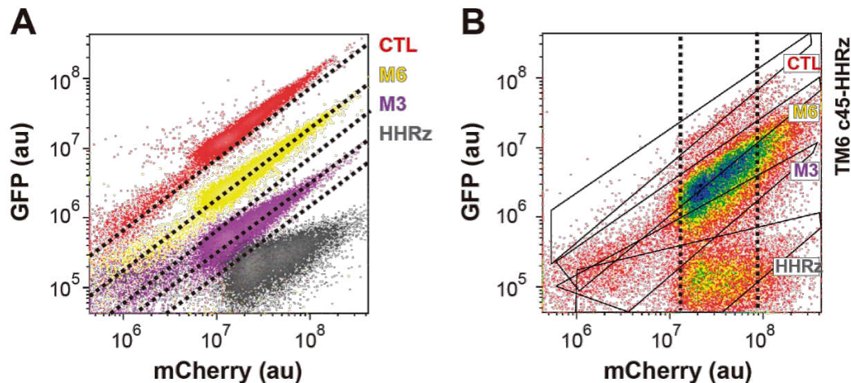
Figure S6. Criteria to set the gate bounds for sorting C45-HHRz RNA device library. A. Setting gates based on GFP/mCherry ratio. Overlay GFP-mCherry dot plot of different HHRz clones used to delimit the full-scale output of the reporter system used in the screening (Figure S3). HHRz , tobacco ringspot virus (sTRSV) HHRz wild-type sequence; CTL , inactive control ribozyme with scrambled active site; M3 and M6 , graded ribozymes with distinct sequences in loops I and II displaying different self-cleaving activity. The upper and lower bounds (dotted lines) of the dynamic range of our reporter system correspond to HHRz (maximal activity) and CTL (no activity). The GFP-mCherry space spanning between these bounds is segmented into four bins whose size (width) is set according to the size that an individual clone has (and which represents roughly half of the intrinsic noise of GFP-mCherry expression). Note that bounds between bins are set so that they split the cell cloud of clones with intermediate GFP/mCherry ratio values ( M3 , M6 ) by half. B. Gating cells based on their mCherry value to reduce noise. GFP-mCherry dot plot of C45-HHRz RNA device library. Polygons depict GFP-mCherry cell clouds of clones used to set sorting gates based on GFP/mCherry ratio as shown in A. Note that, in case of the mCherry expression values lower than about 10^7 but still considered positive for mCherry (Figure S3), cell populations displaying different GFP/mCherry ratios (polygons) get closer to each other and overlap. In contrast, cells with high mCherry values diverge, and differences in the ratio become less predictable. Gating cells with an intermediate mCherry expression value (between dotted lines) generates a more robust ratio output for cells in the populations.
