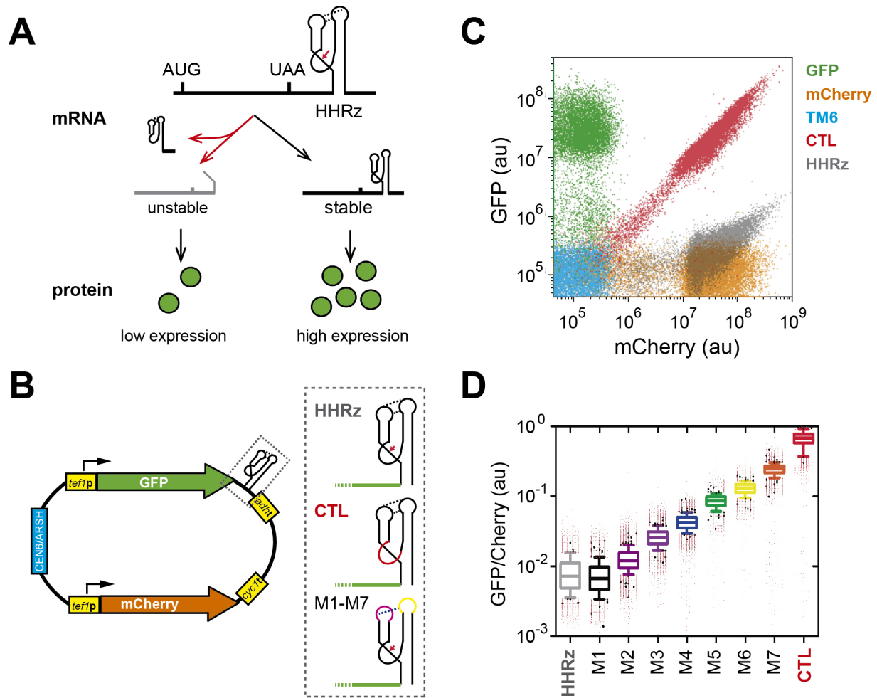
Figure S3. An in vivo reporter system that couples RNA conformational changes with a measurable quantitative fluorescent readout. A. The tobacco ringspot virus (sTRSV) hammerhead ribozyme (HHRz) is inserted downstream the stop codon (UAA) of a reporter gene. Self-cleaving activity yields transcripts with shorter 3'UTR, which are less stable than transcripts with uncut 3'UTR. The red arrow denotes the cutting point. B. Schematic drawing of the map of the plasmid backbone (pCS1748, (Liang et al. , 2012)) used to clone the C45-HHRz library in the in vivo screening approach. HHRz , the tobacco ringspot virus (sTRSV) HHRz wild-type sequence; CTL , the inactive control ribozyme with a scrambled active site (red); M1-M7 , a set of graded ribozymes with distinct sequences in loops I (magenta) and II (yellow) (Townshend et al. , 2015), which are predicted to display different long-distance tertiary structure interactions between loops I and II (dotted line), hence different self-cleaving activities that would differently affect GFP mRNA stability and protein expression. The green lines next to the HHRz schematic structures represent the rest of the GFP mRNA including the coding region. C. Overlay FACS dot plot showing GFP-mCherry expression pattern in controls used in this study. The dynamic range of this reporter system is covered by the space spanning from (and including) CTL (red cloud) to HHRz (grey cloud). TM6 , the untransformed double-negative host strain; GFP , the GFP-only control plasmid pCS1585; mCherry , the mCherry-only control plasmid pCS1749. D. The box plot showing the distribution of the GFP/mCherry ratio in single cells
