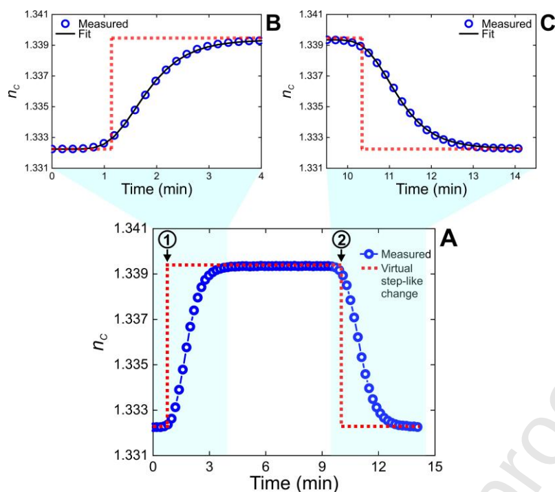
Fig. 6 A. Flushing of an SH812-08 OWLS flow cell with 6% (v/w) glycerol solution. Measured solution RI ( n_c ) as a function of time (blue circles). Experimental phases: introduction of glycerol solution (1) and DI water (2) into the flow cell. n_c values were calculated based on the 3-layer mode equations. The dashed red lines represent the unrealistic, but commonly used, case when the change of bulk concentration in the flow cell is assumed to be immediate and is described by a step function. B-C. Two relevant sections of the flushing curve were fitted by Eq. (40) (logistic function), resulting in the fitted curves (black solid line) and the following fit parameters: q = 0.03277 , g = 0.04284 ( B ); q = 0.03018 , g = 0.06972 ( C ).
