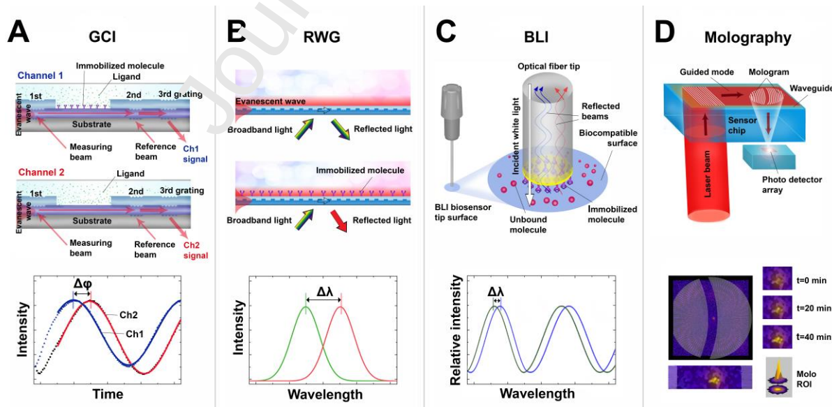
Fig. 2 Measuring principles of cutting-edge label-free optical biosensor technologies. Schemes on the top and graphs on the bottom represent the measurement setup and raw measurement data of the corresponding technique. The diagrams and graphs are adapted from the below listed references.
