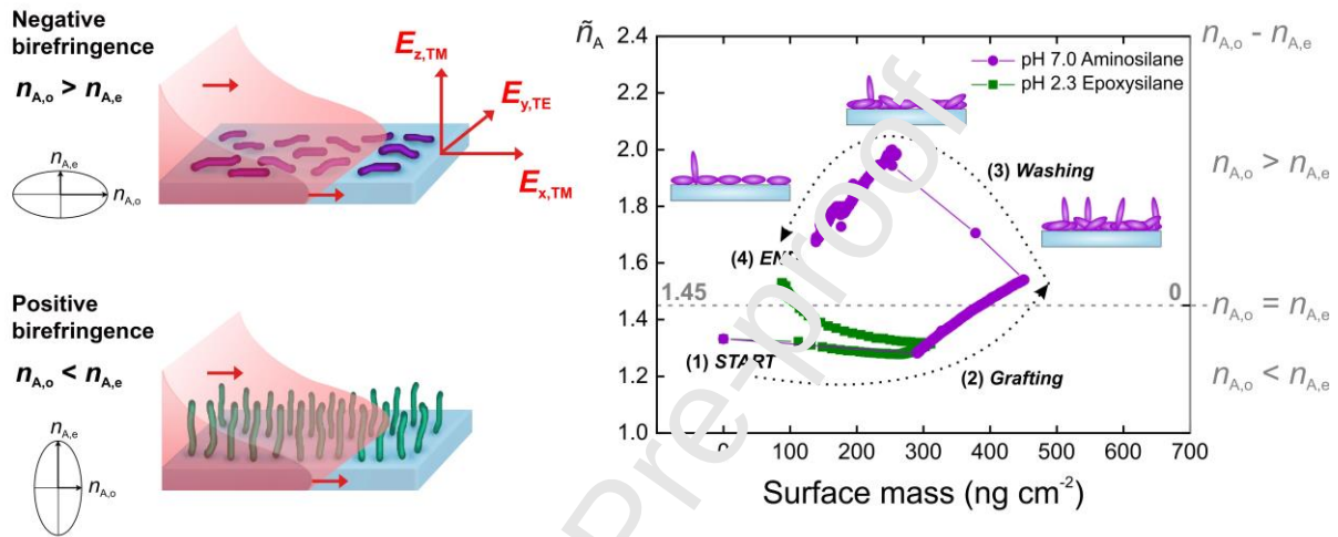
Fig. 17 Principle of OWLS sensitivity to adlayer structure and its exploitation on obtaining structural information. Two distinctive situations are shown where negative birefringence is produced by only polymer chains lying down and positive birefringence is produced by only end-grafted chains. The refractive index ellipsoids (left) demonstrates the relative magnitude of n_{A,o} and n_{A,e} in the case of the two structures. The drawings highlight both the adlayer structures and the orientational sensitivity of the TE and TM waveguide modes by indicating the electric field directions of the sensing modes. The data shown in the \tilde{n}_A - M graph represents the formation of carboxymethyl dextran (CMD) layer grafted to OWLS chip surface using different surface chemistries as indicated in the legend. The expected RI value of CMD ( \tilde{n}_A = 1.45 ) given on the \tilde{n}_A axis can be used as a reference point on the right birefringence axis. The direction of the experiment in time and the separate experimental phases are indicated by the arrows and numbers. While using aminosilane-modified surface at pH 7.0 resulted in mostly side-on grafting of the CMD chains, on epoxysilane-modified surface at pH 2.3 the end-on grafting dominated over a considerable part of the grafting. However, at the end of the experiment, the layer structure was found to be rather lying down. The data were adapted from Ref [30]. [Adapted from Ref. [30], copyright 2016 Elsevier]
