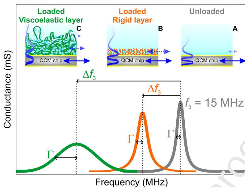
Fig. 15 Principle of QCM sensitivity to adlayer structure. The inset drawings on the top correspond to the bottom resonance curves and represent QCM chips in different conditions. See the colors for matching the drawings and curves. Inset image A represents an unloaded QCM chip, where only a thin part of the bulk solution oscillates together with the crystal. The shear wave generated by the chip oscillation is also shown. B . If the QCM chip is loaded by a thin and rigid adlayer with a low water content, the decay of the penetrating shear wave is similar to the unloaded case, only a frequency shift is detected, but \Gamma is almost unchanged. C . In case of a thick, viscoelastic adlayer potentially possessing a large water content, the layer does not oscillate perfectly together with the crystal resulting in an increase in dissipation and thus a marked widening in \Gamma .
